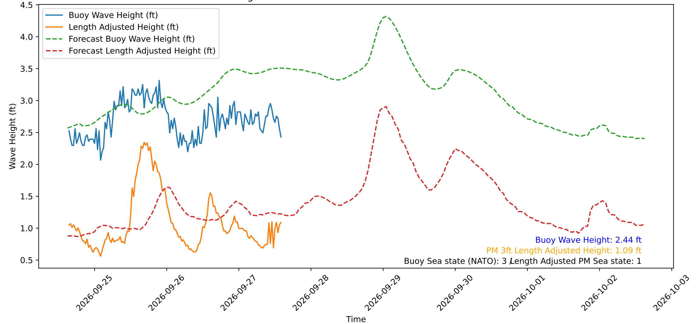
Wave Heights over Time for Red Beach at 2026-09-27 15:10:50
