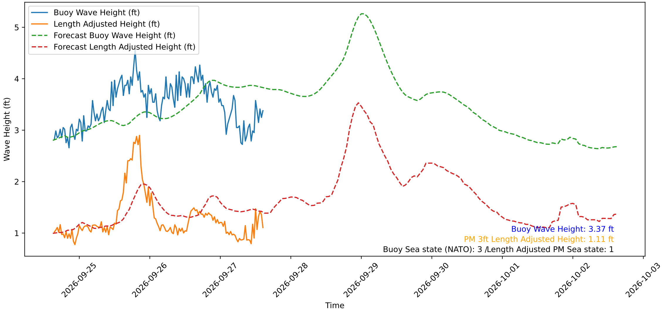
Wave Heights over Time for Green Beach at 2026-09-27 15:11:13
