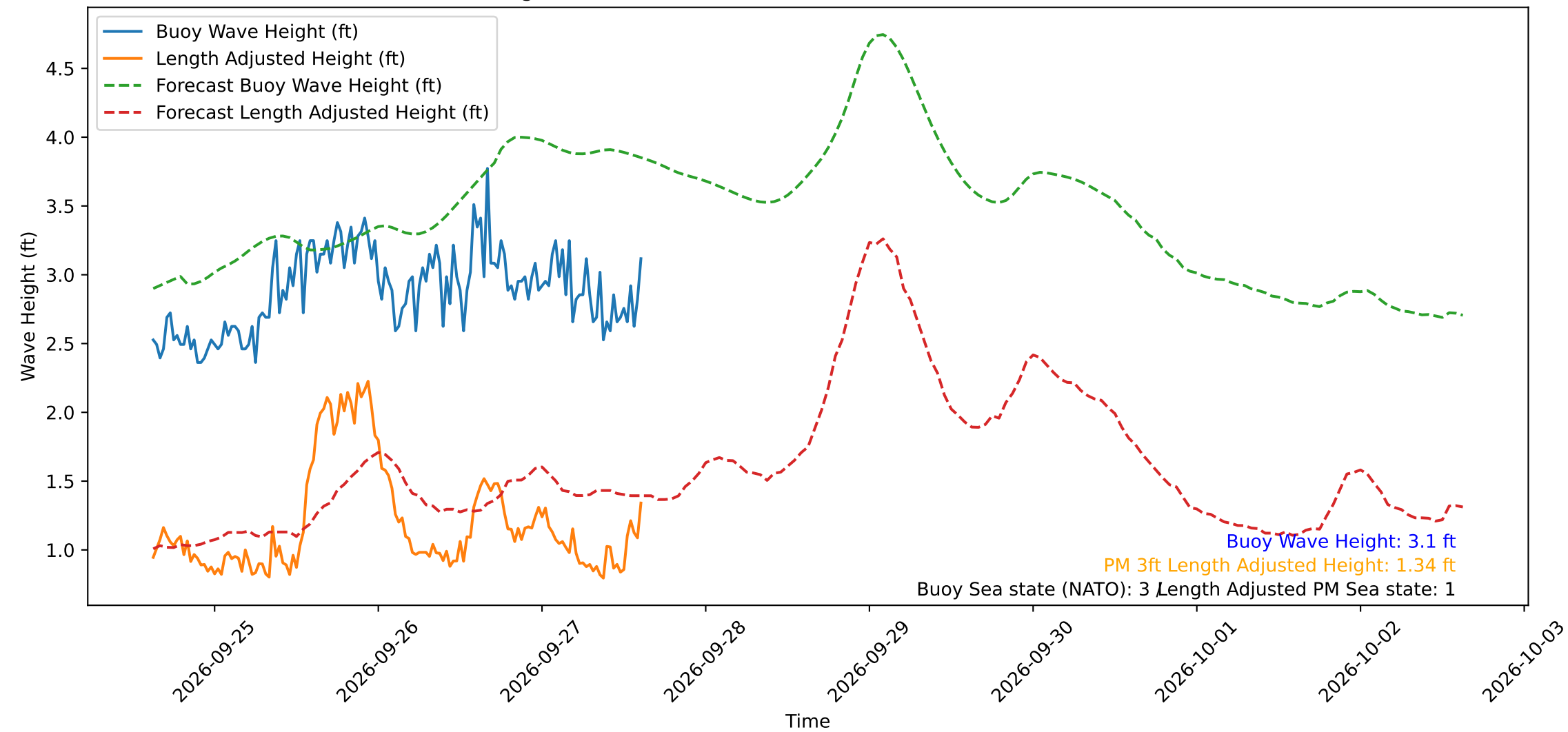
Wave Heights over Time for Oceanside Harbor at 2026-09-27 15:10:30
