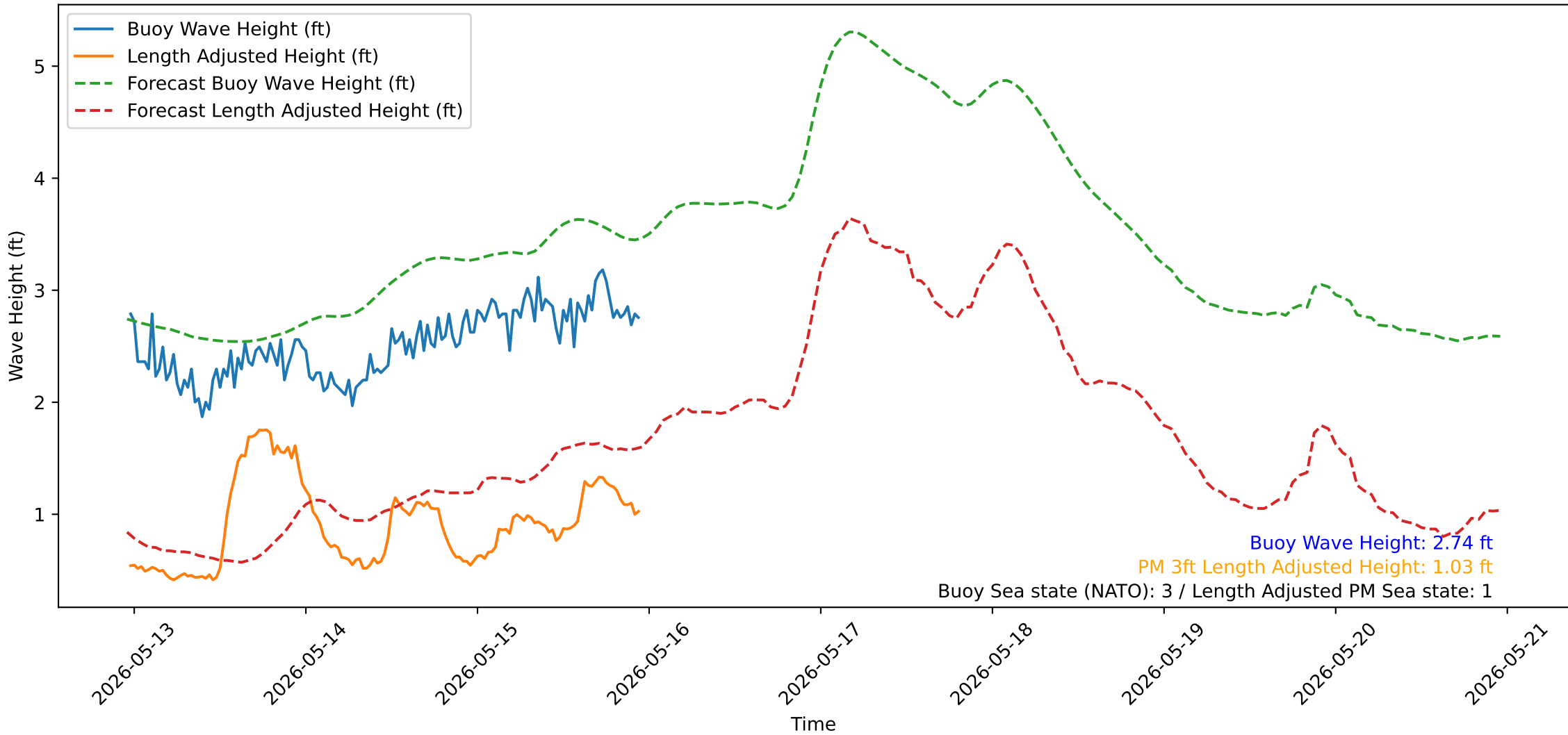
Wave Heights over Time for Red Beach at 2026-05-15 23:10:52
