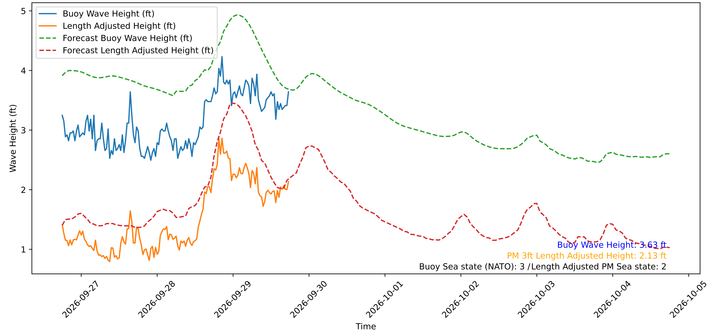
Wave Heights over Time for Oceanside Harbor at 2026-09-29 18:10:29
