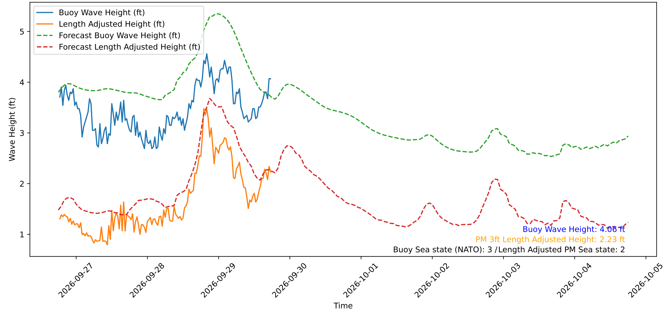
Wave Heights over Time for Green Beach at 2026-09-29 18:11:12
