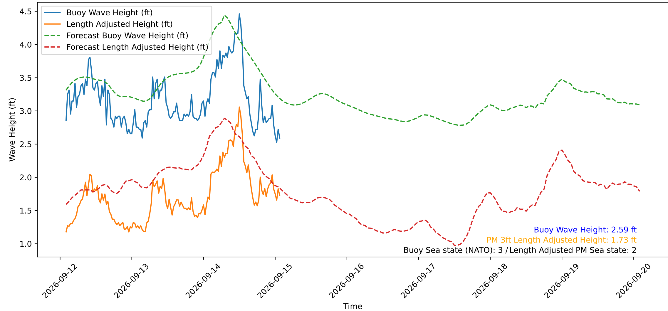
Wave Heights over Time for Oceanside Harbor at 2026-09-15 02:10:29
