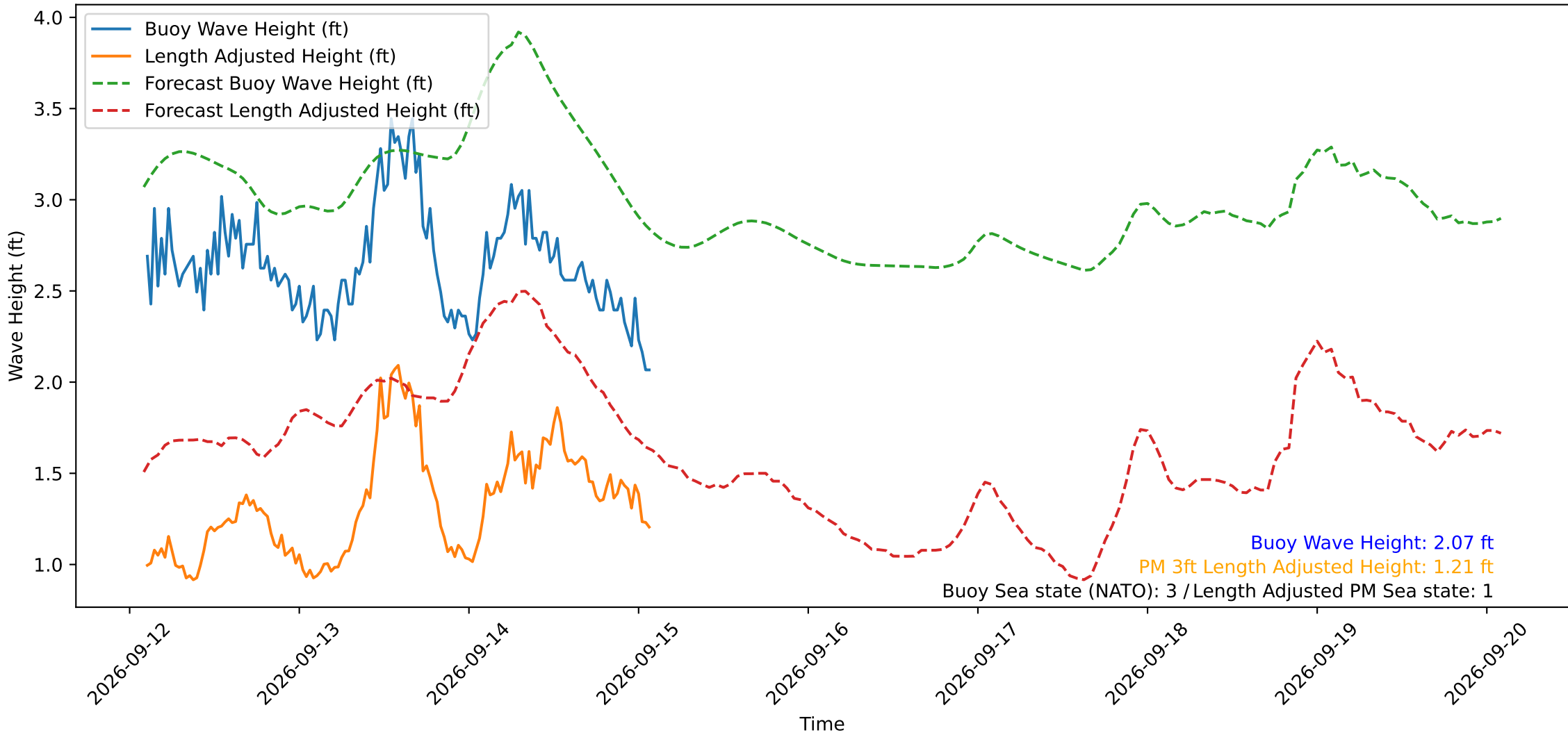
Wave Heights over Time for Red Beach at 2026-09-15 02:10:49
