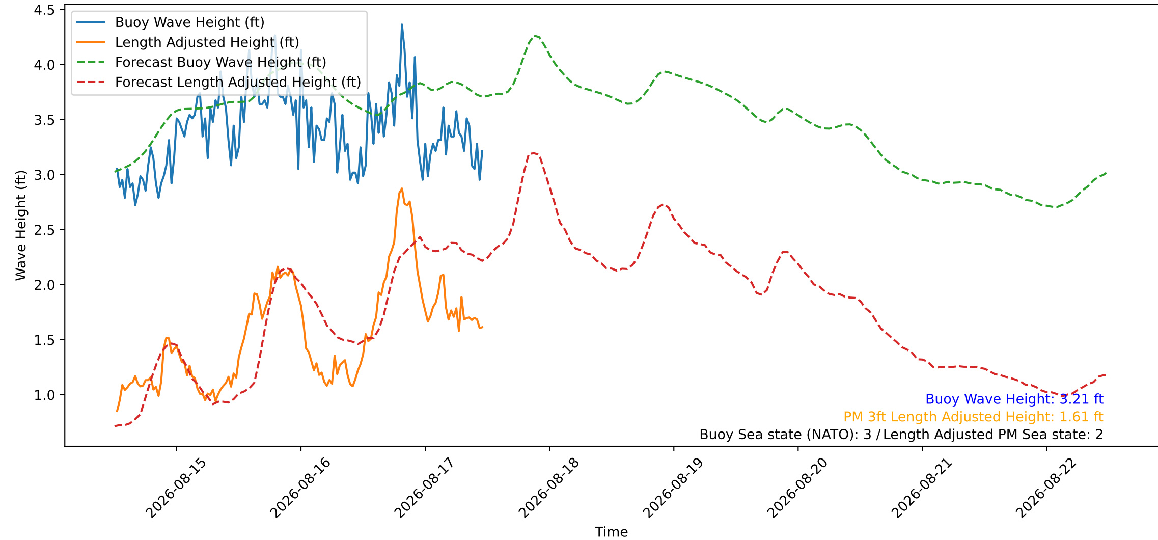
Wave Heights over Time for Green Beach at 2026-08-17 12:01:09
