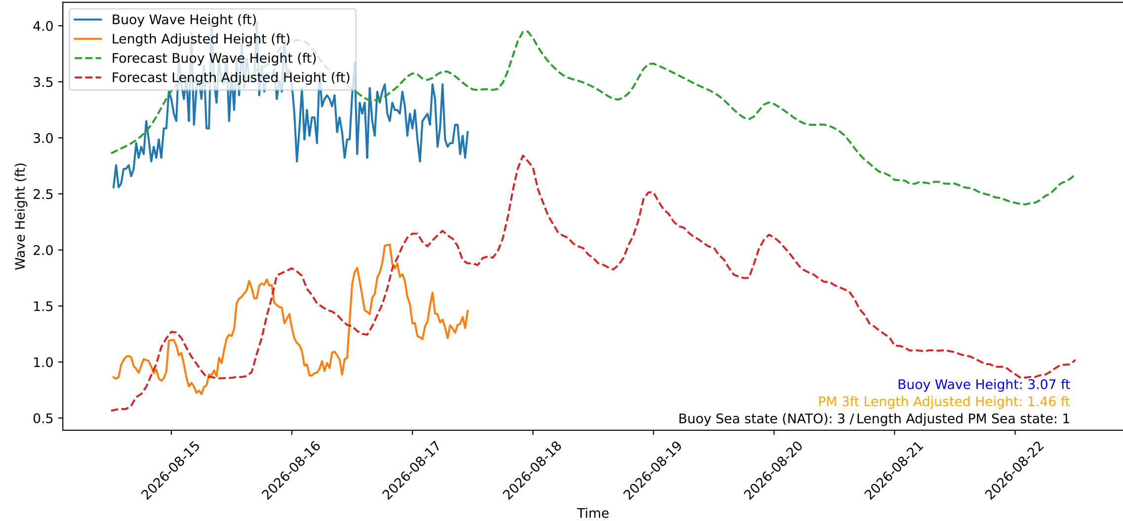
Wave Heights over Time for Red Beach at 2026-08-17 12:00:47
