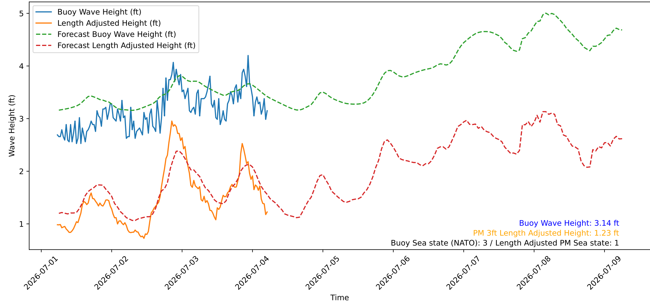
Wave Heights over Time for Green Beach at 2026-07-04 05:41:09
