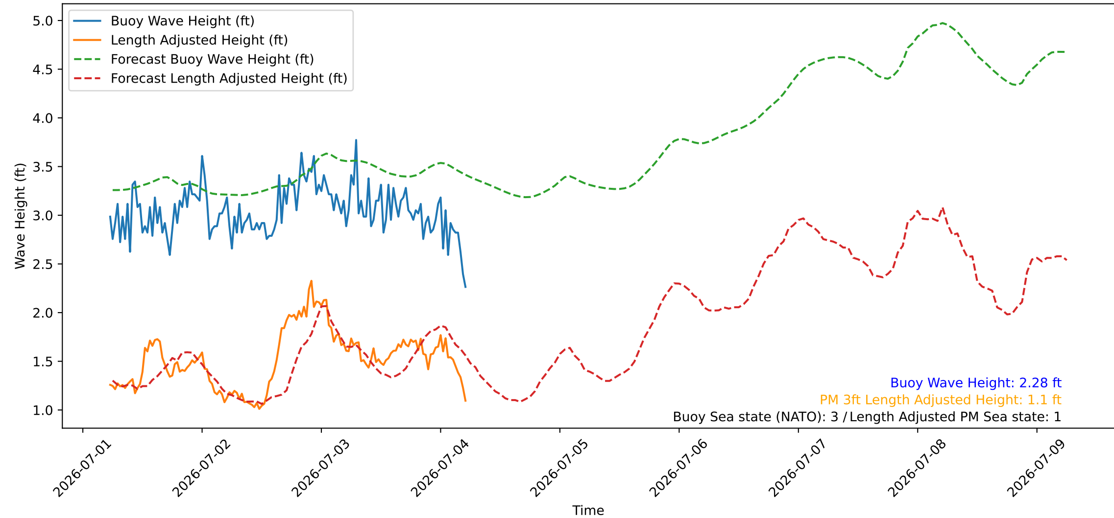
Wave Heights over Time for Oceanside Harbor at 2026-07-04 05:40:27
