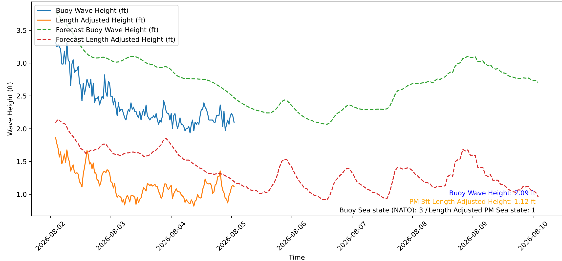
Wave Heights over Time for Green Beach at 2026-08-05 02:01:07
