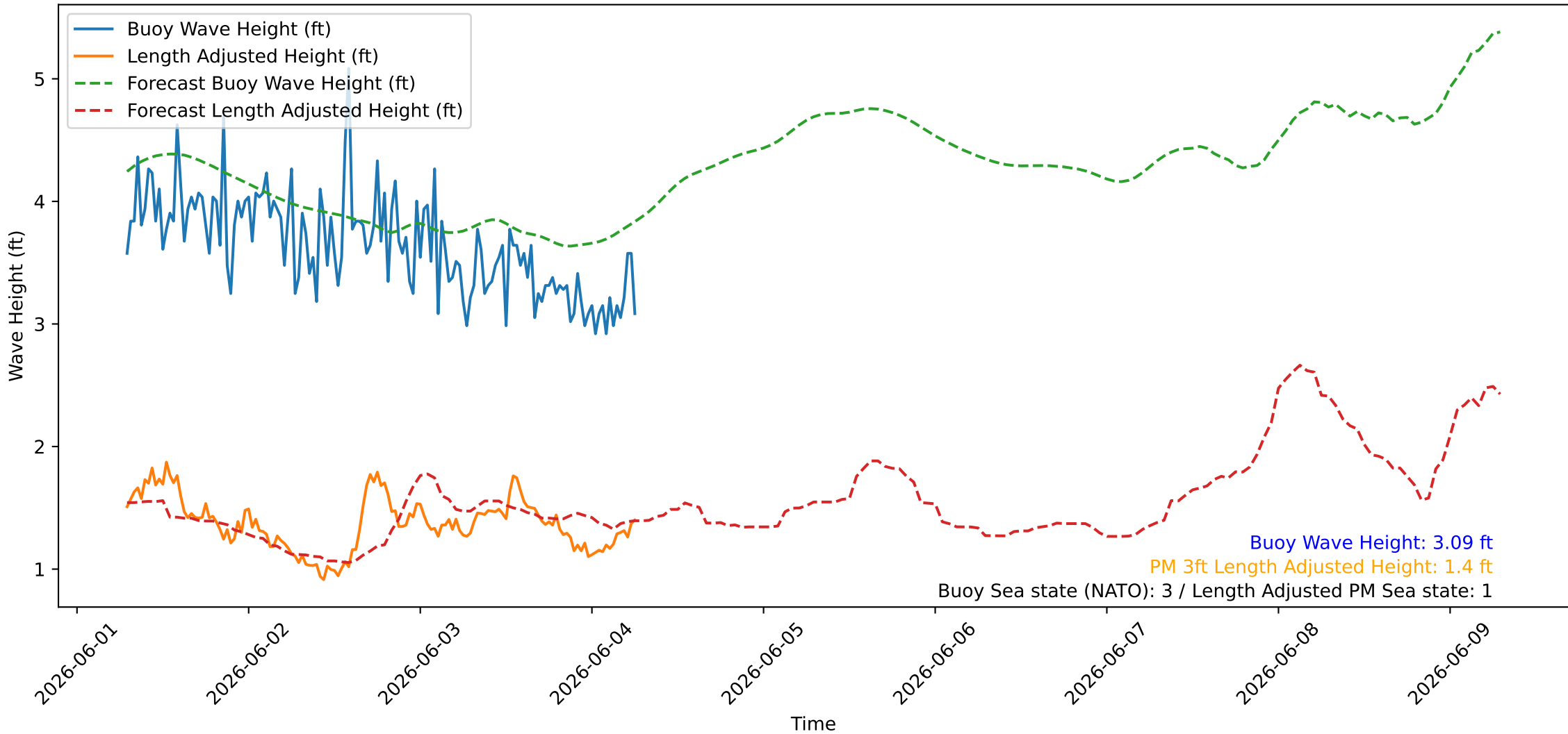
Wave Heights over Time for Oceanside Harbor at 2026-06-04 06:50:26
