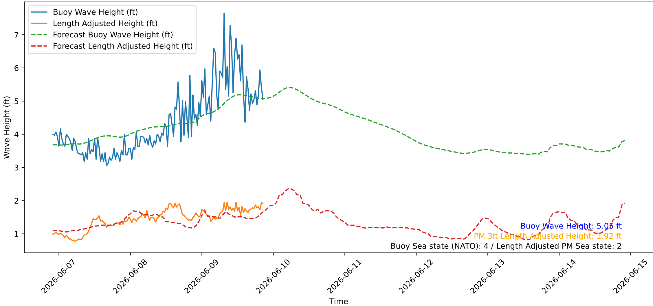
Wave Heights over Time for Red Beach at 2026-06-09 21:30:46
