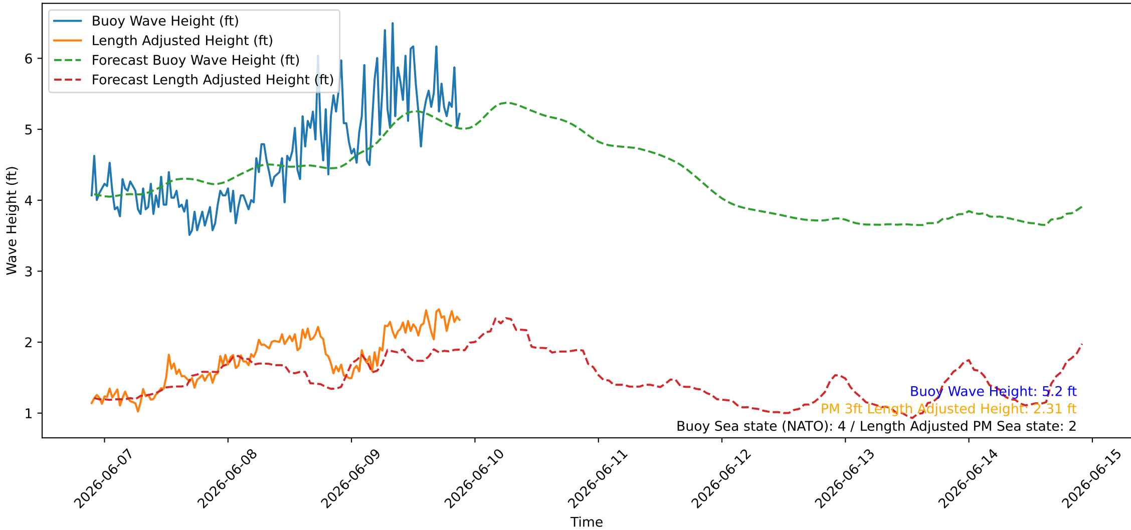
Wave Heights over Time for Oceanside Harbor at 2026-06-09 21:30:26
