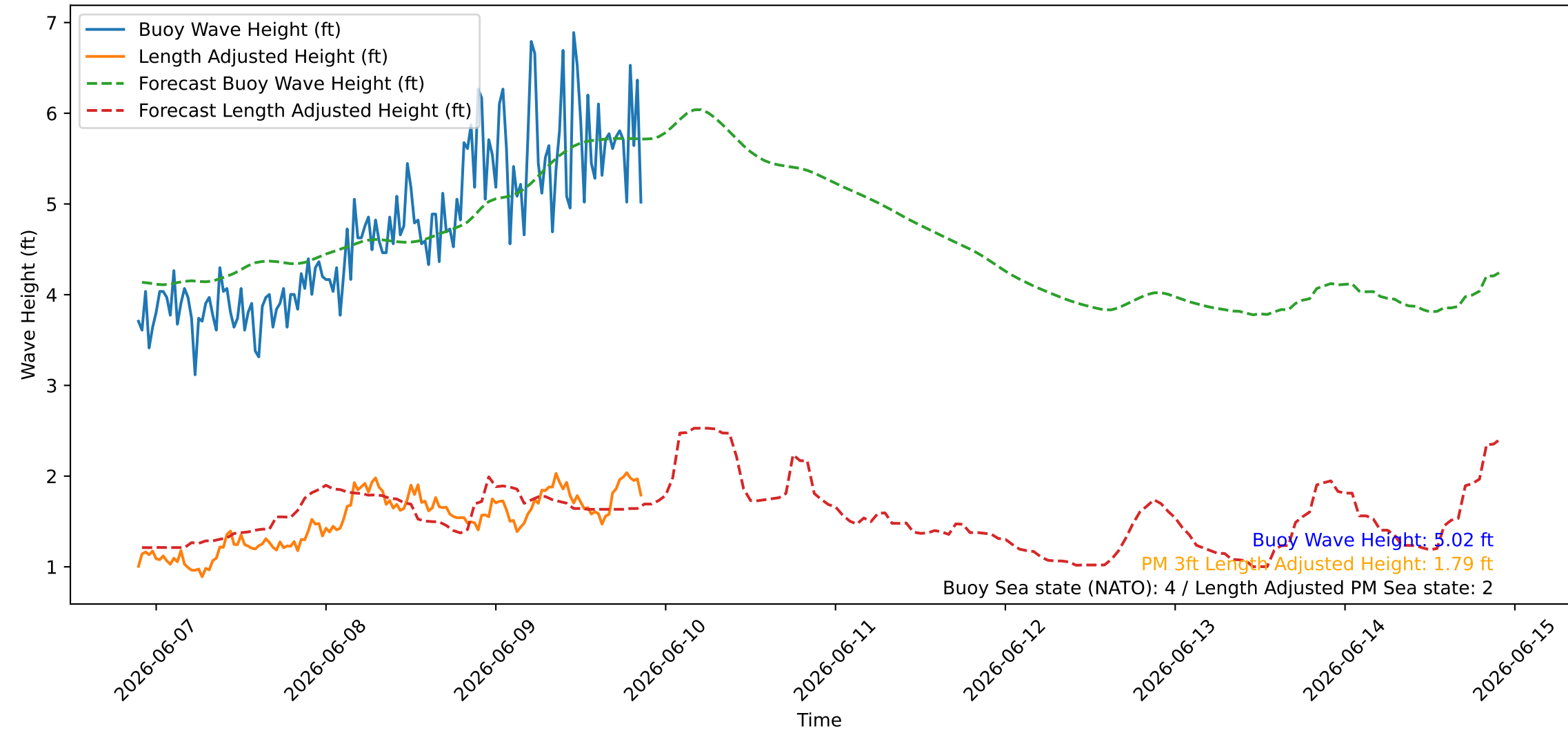
Wave Heights over Time for Green Beach at 2026-06-09 21:31:10
