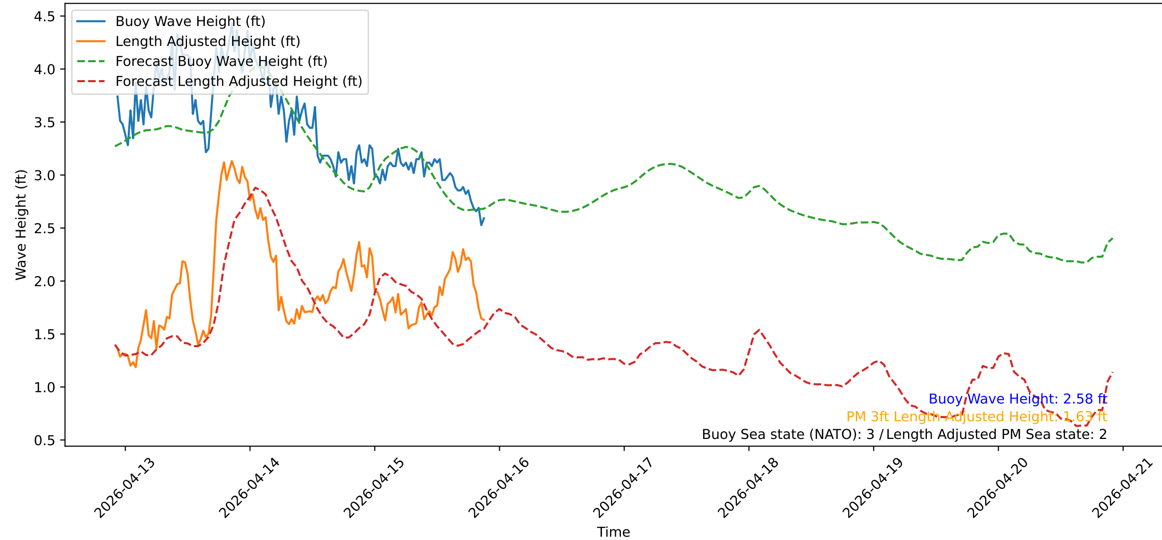
Wave Heights over Time for Red Beach at 2026-04-15 22:00:51
