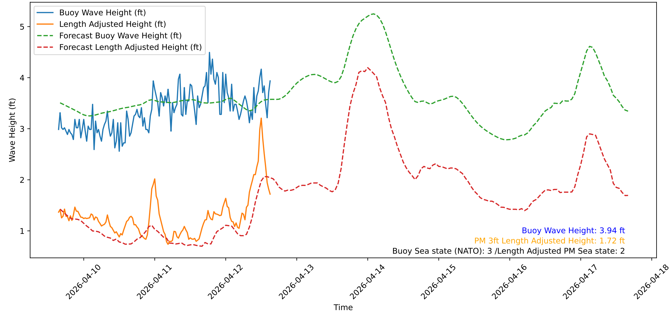
Wave Heights over Time for Green Beach at 2026-04-12 15:41:12
