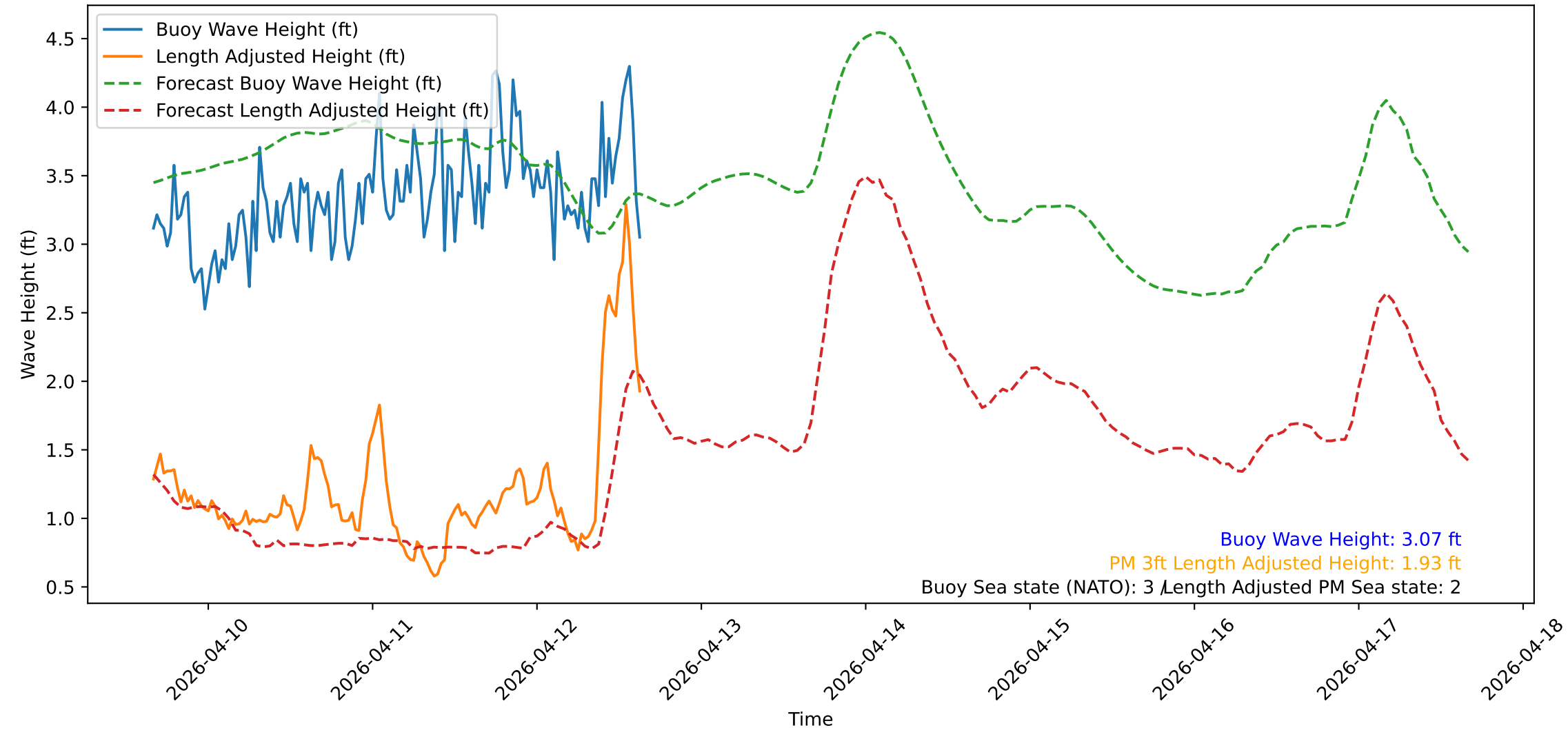
Wave Heights over Time for Red Beach at 2026-04-12 15:40:50
