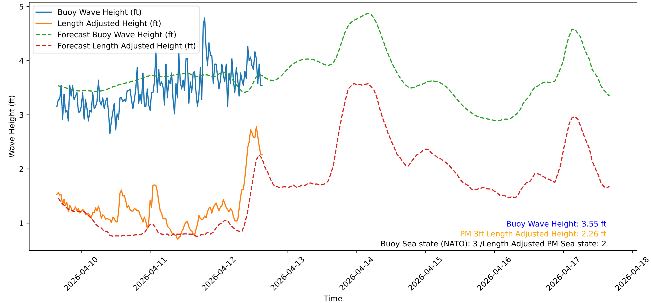
Wave Heights over Time for Oceanside Harbor at 2026-04-12 15:40:31
