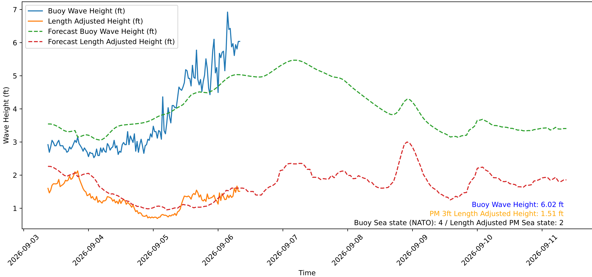
Wave Heights over Time for Red Beach at 2026-09-06 08:50:50
