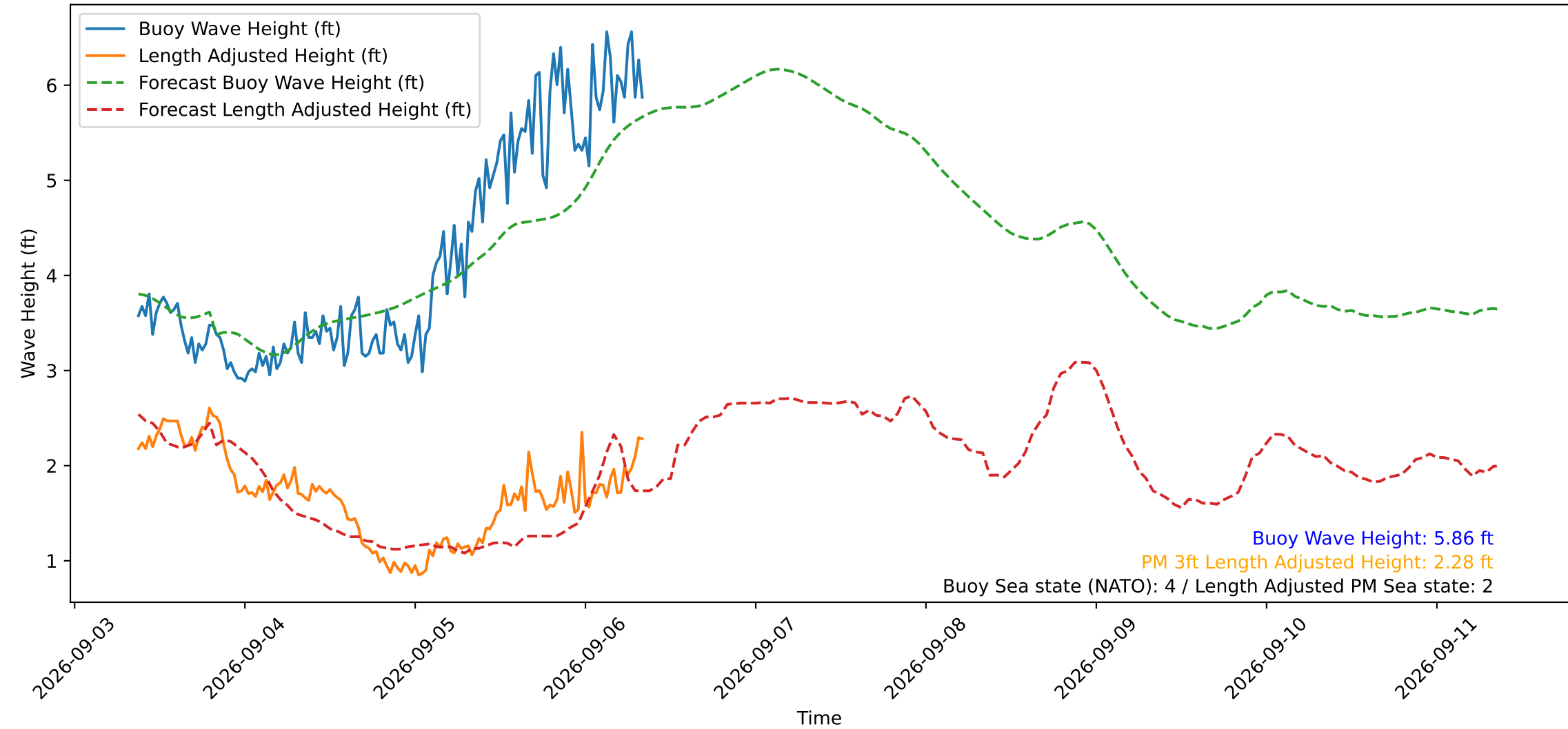
Wave Heights over Time for Oceanside Harbor at 2026-09-06 08:50:29
