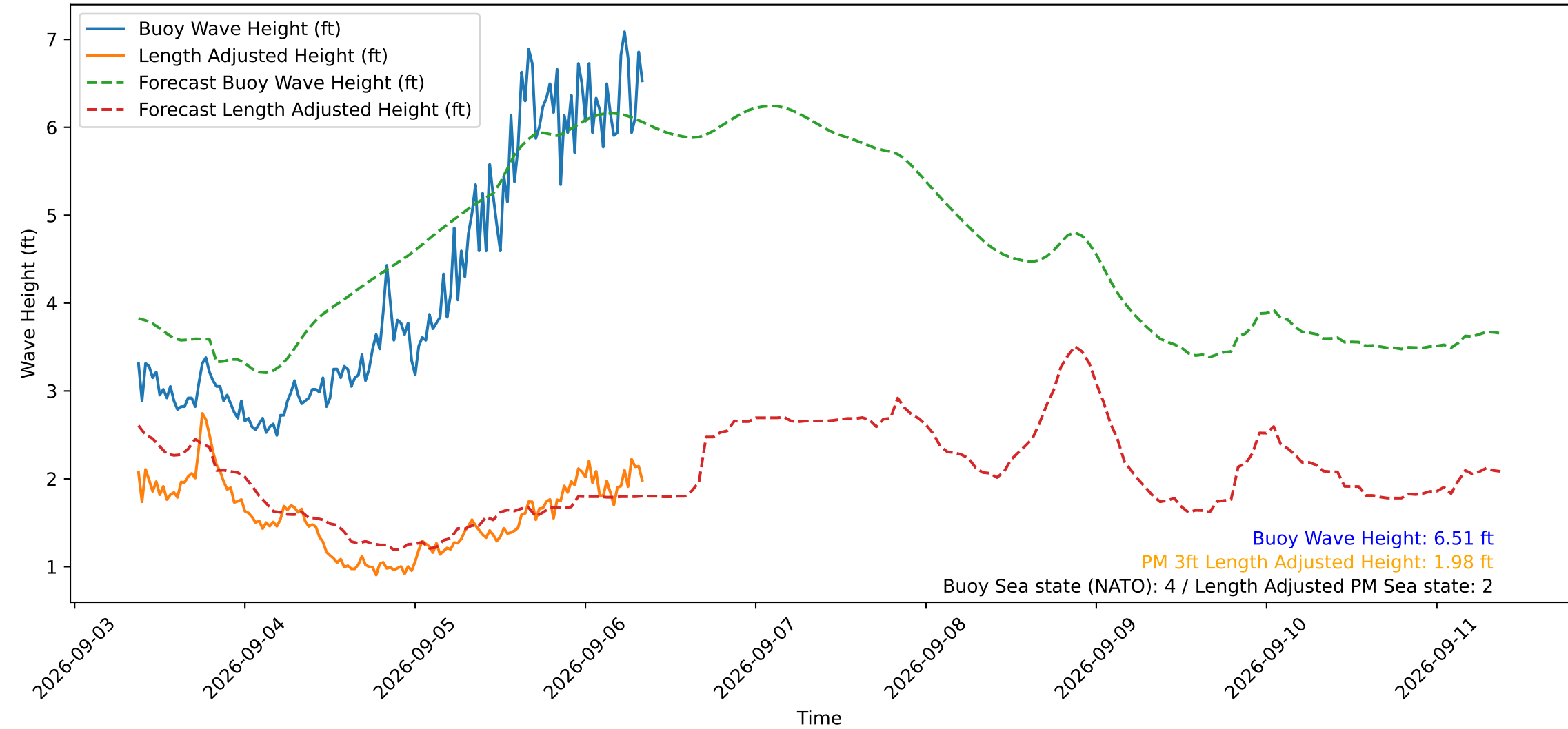
Wave Heights over Time for Green Beach at 2026-09-06 08:51:14
