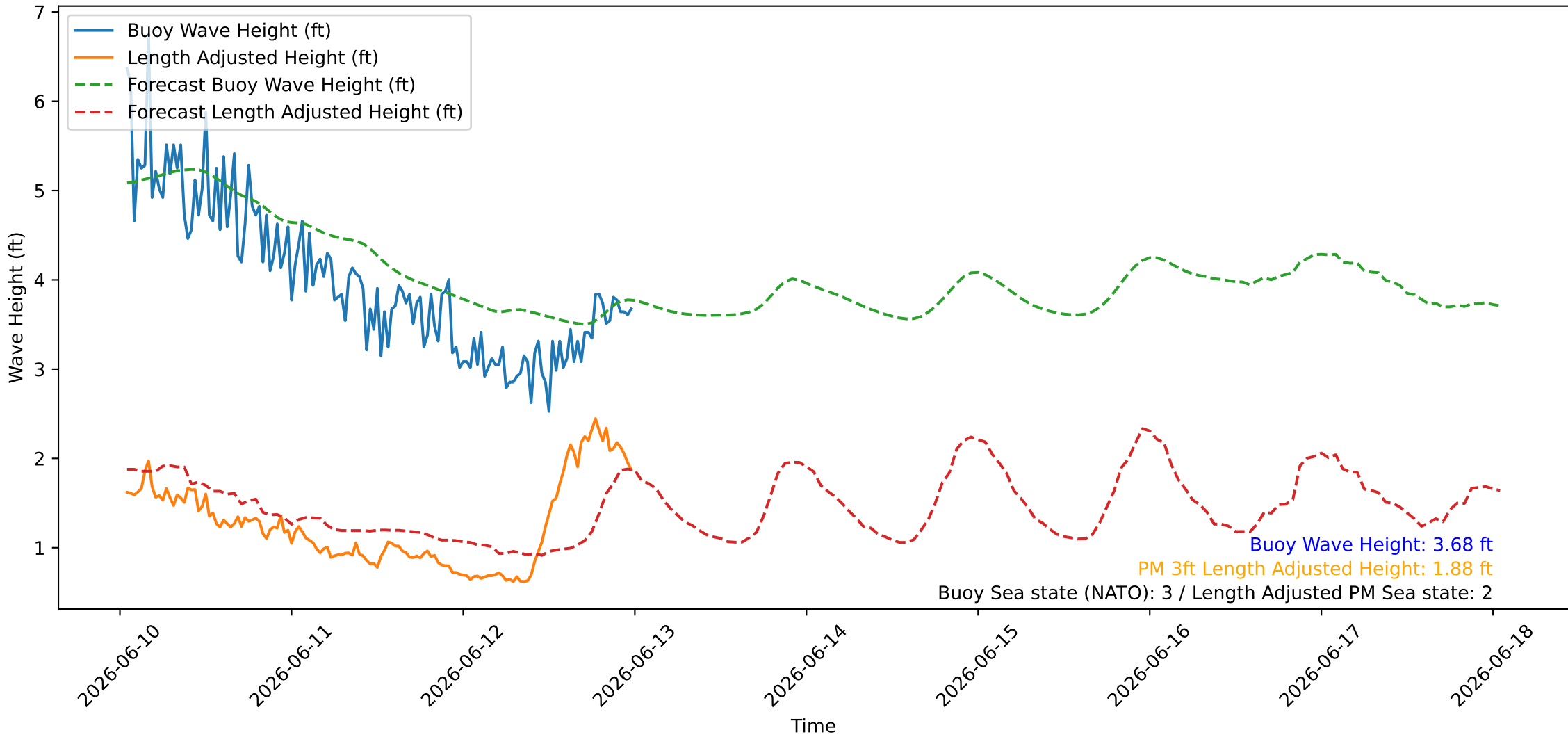
Wave Heights over Time for Red Beach at 2026-06-13 00:30:46
