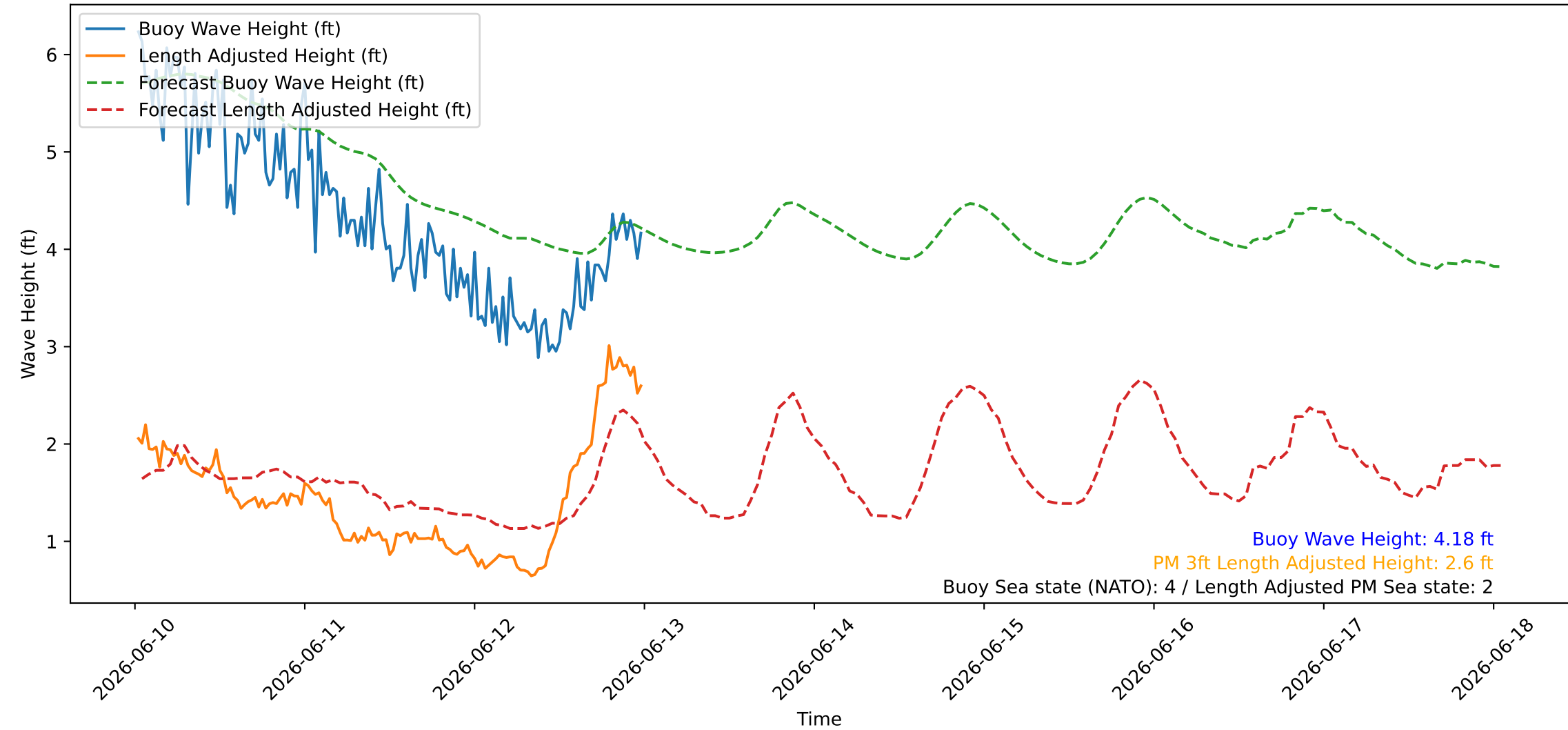
Wave Heights over Time for Green Beach at 2026-06-13 00:31:08
