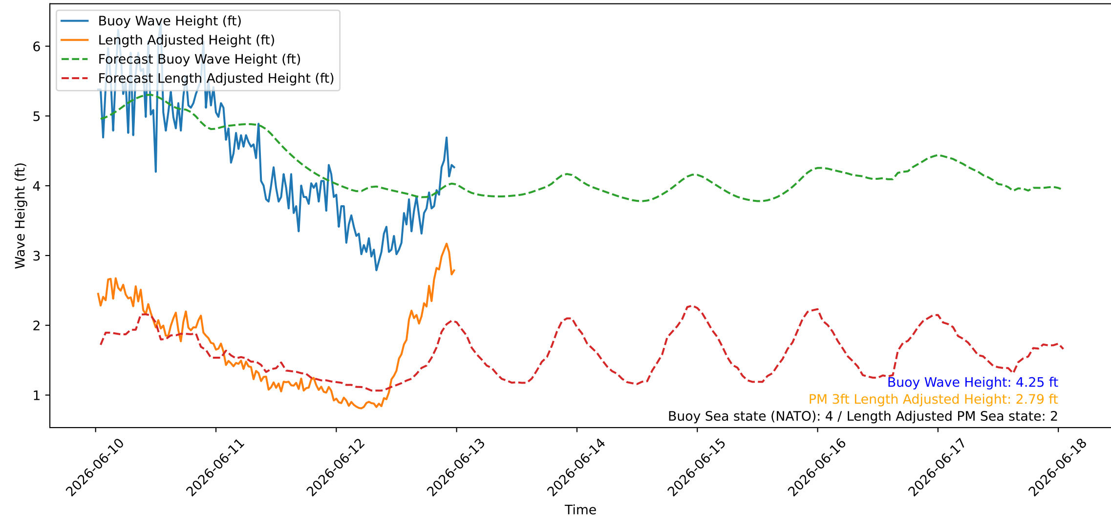
Wave Heights over Time for Oceanside Harbor at 2026-06-13 00:30:26
