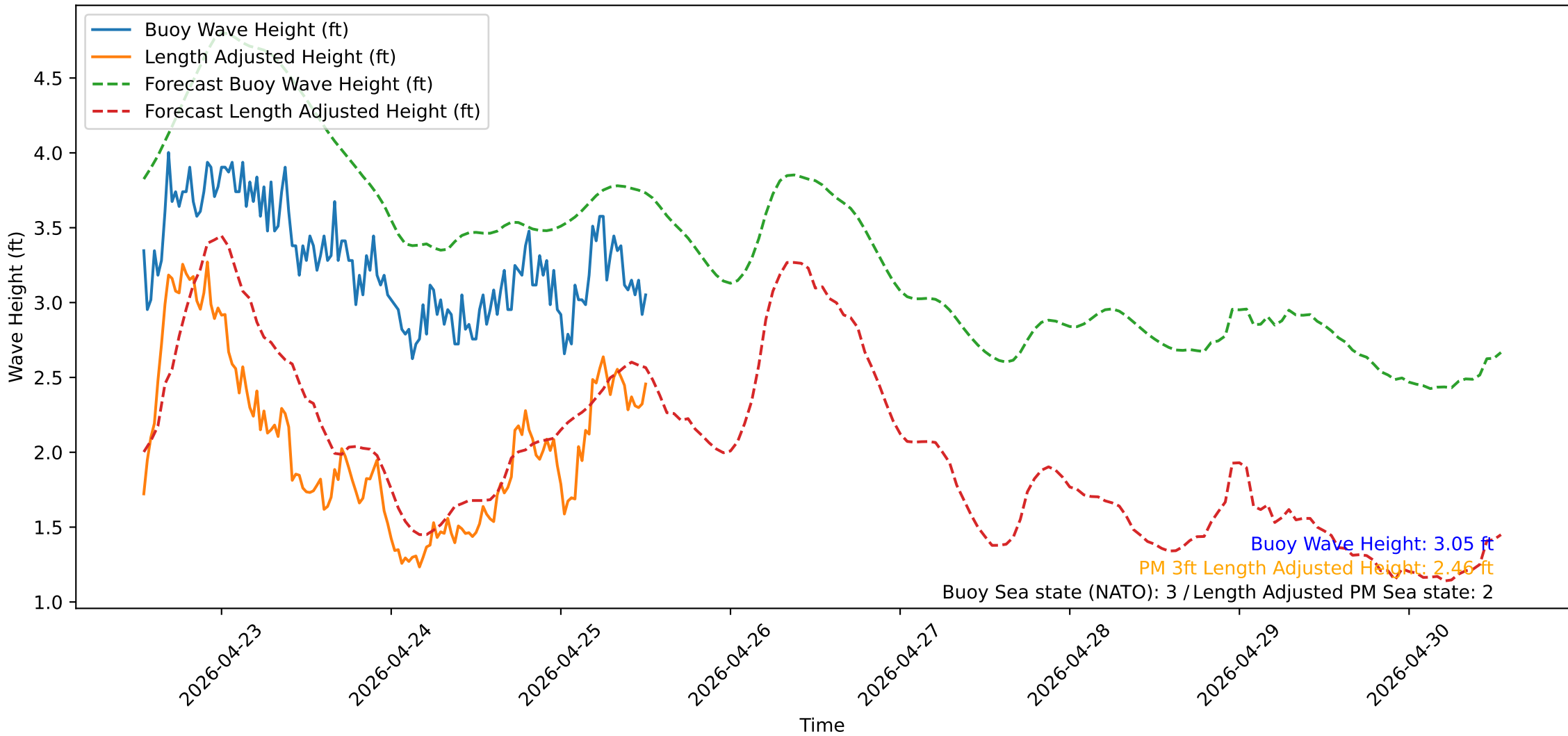
Wave Heights over Time for Green Beach at 2026-04-25 13:01:12
