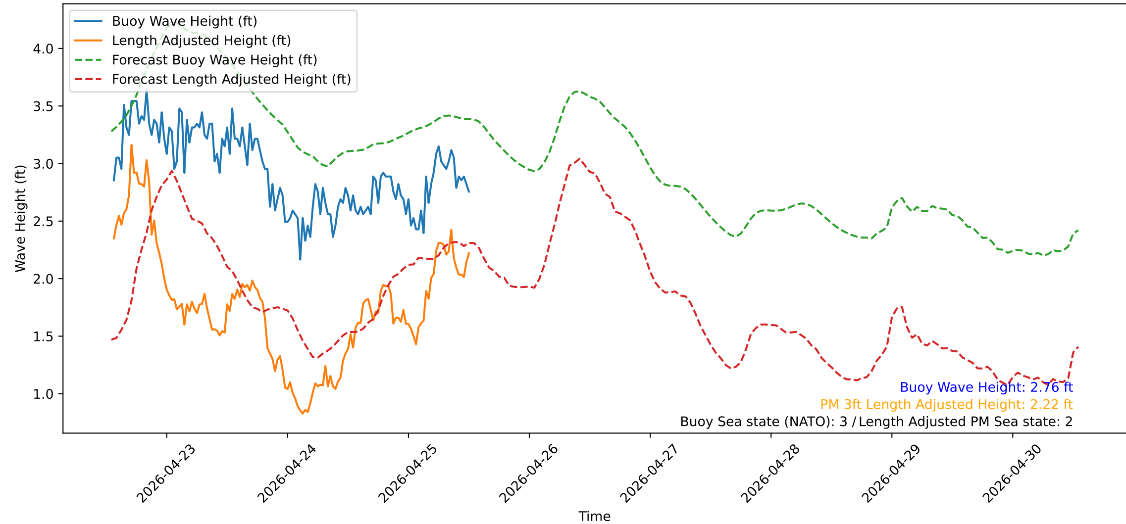
Wave Heights over Time for Red Beach at 2026-04-25 13:00:50
