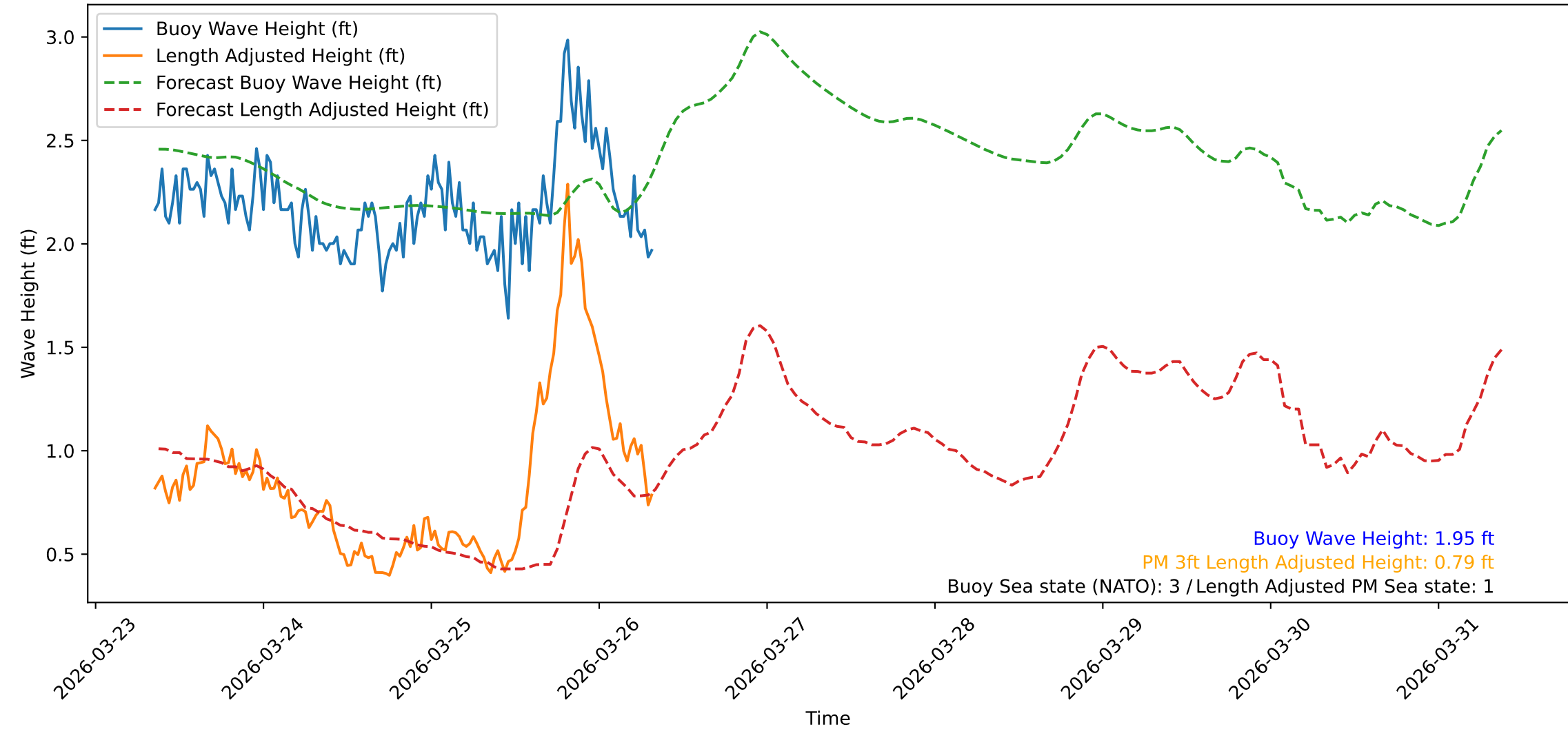
Wave Heights over Time for Green Beach at 2026-03-26 08:31:10
