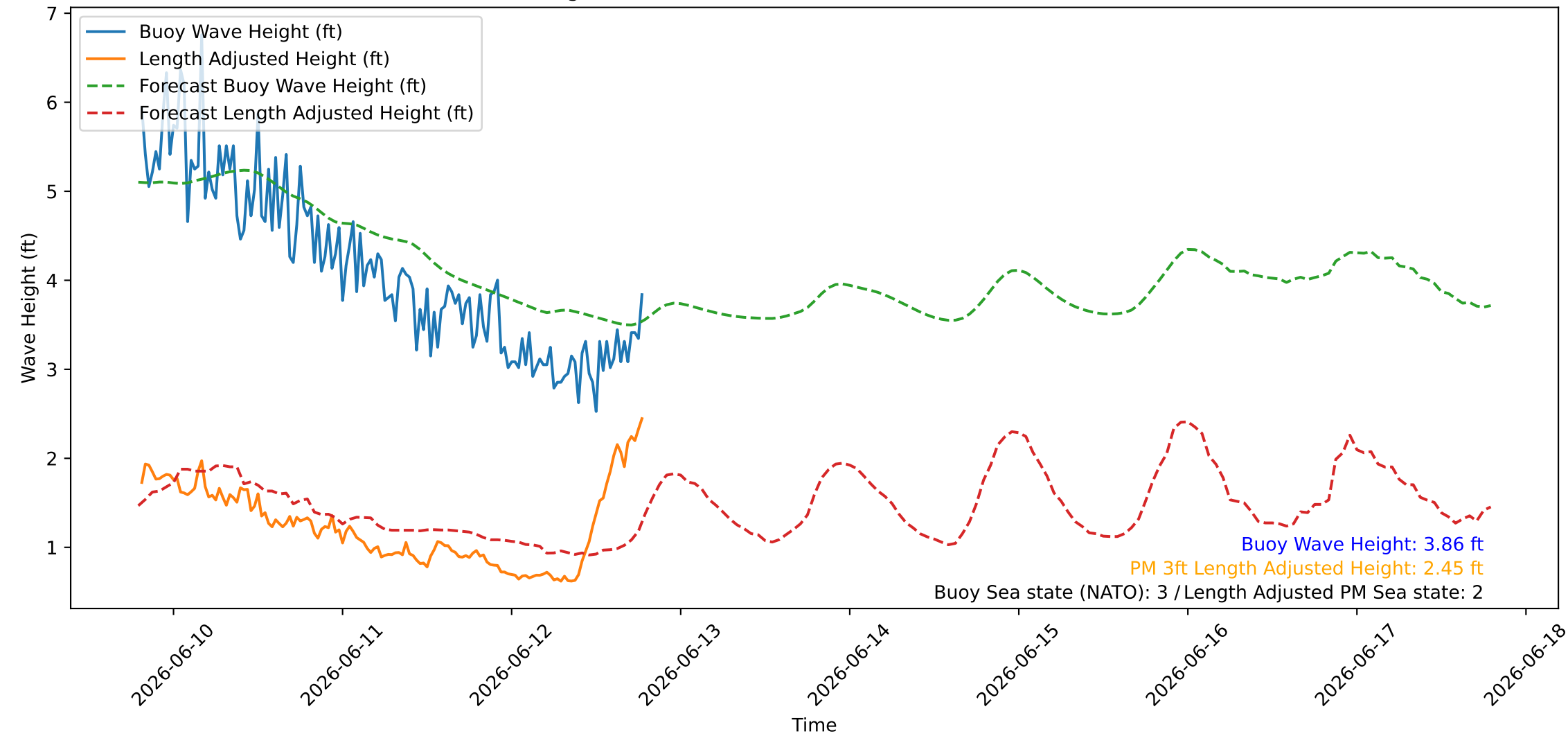
Wave Heights over Time for Red Beach at 2026-06-12 19:20:47
