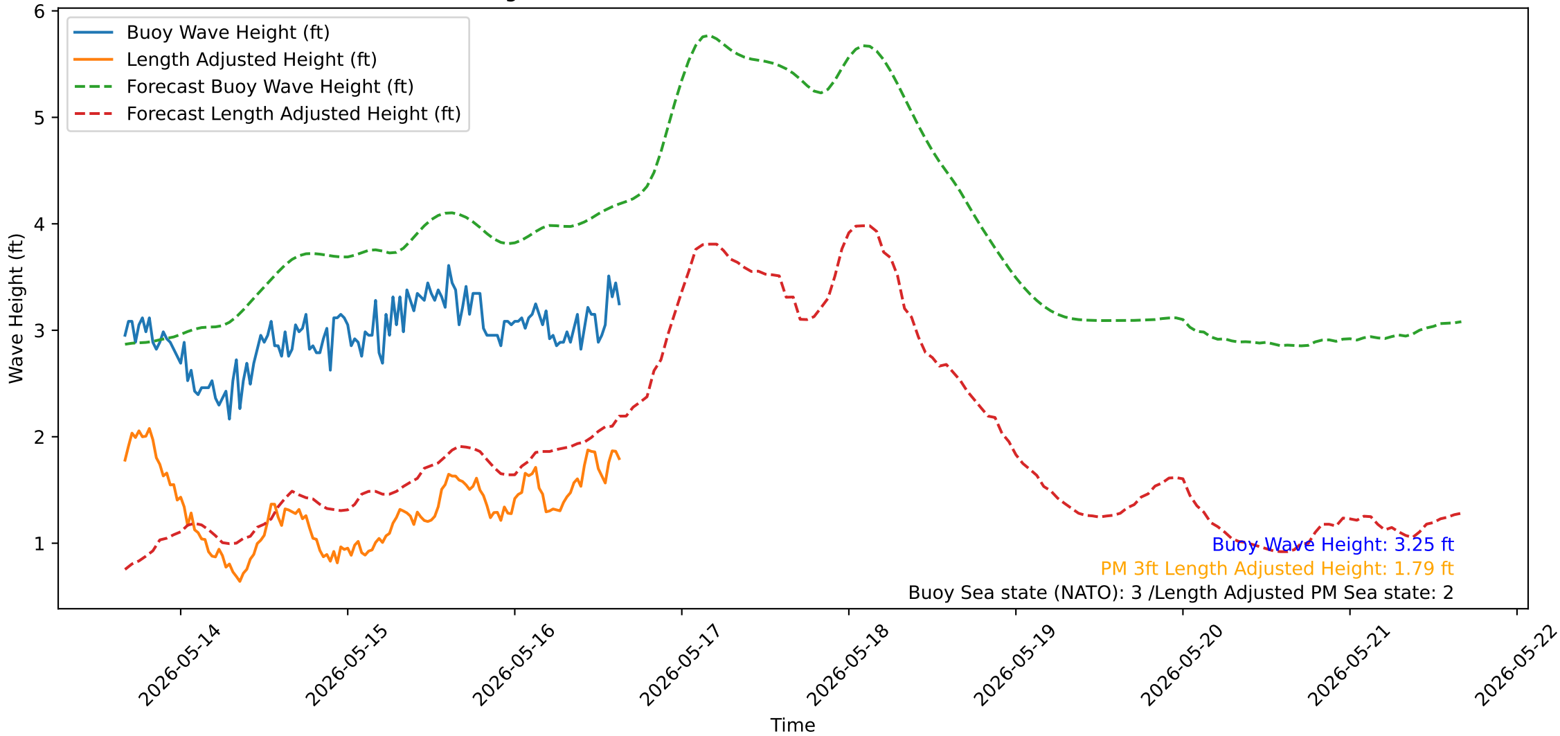
Wave Heights over Time for Oceanside Harbor at 2026-05-16 15:50:32
