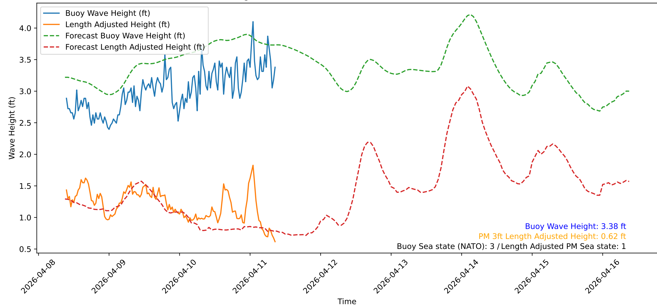
Wave Heights over Time for Red Beach at 2026-04-11 09:20:52
