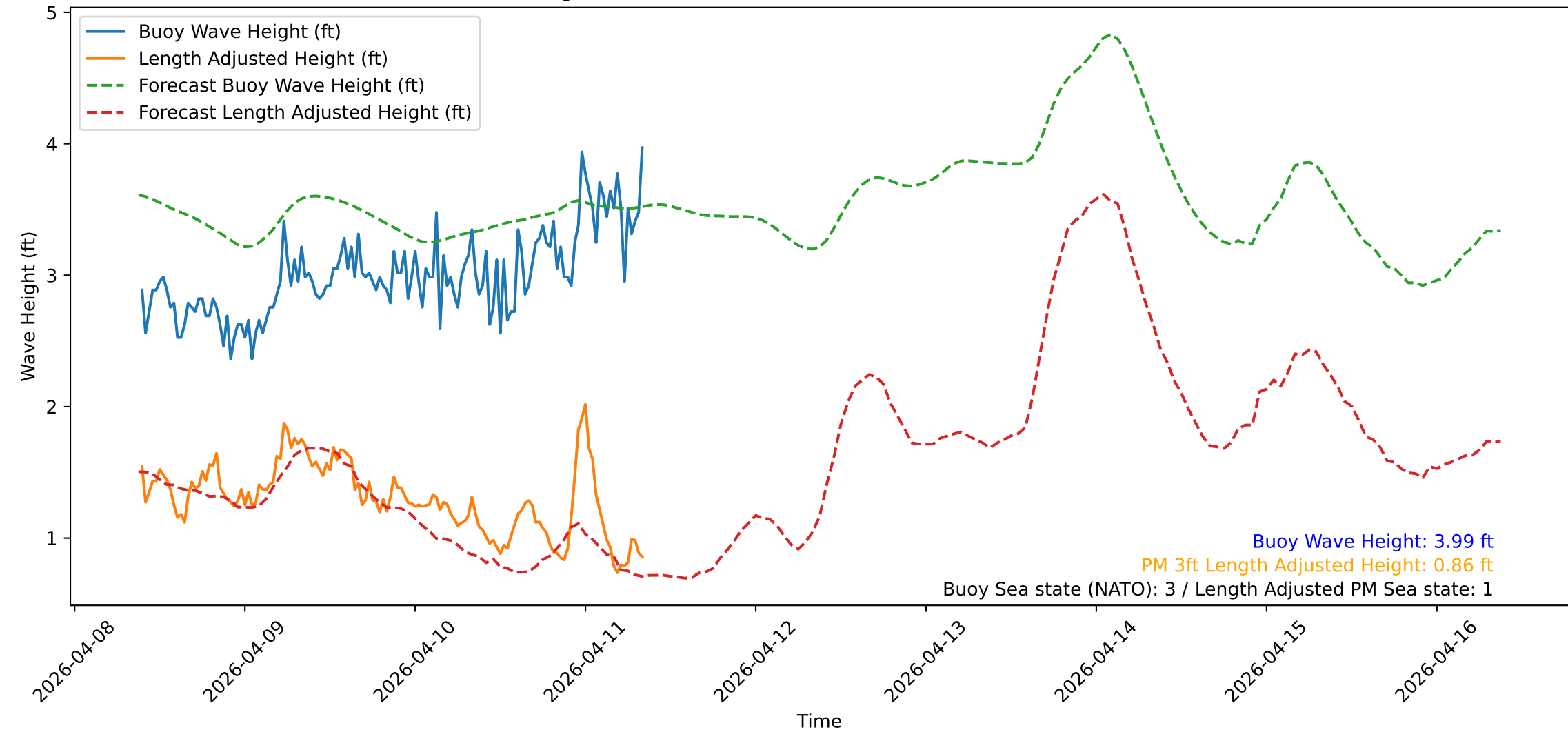
Wave Heights over Time for Green Beach at 2026-04-11 09:21:15
