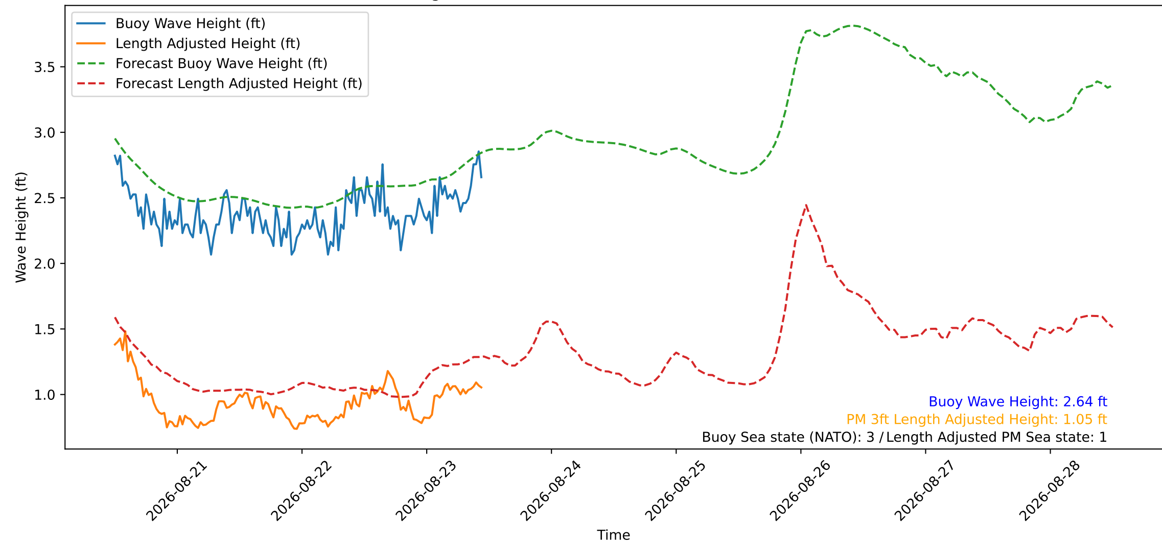
Wave Heights over Time for Red Beach at 2026-08-23 11:30:49
