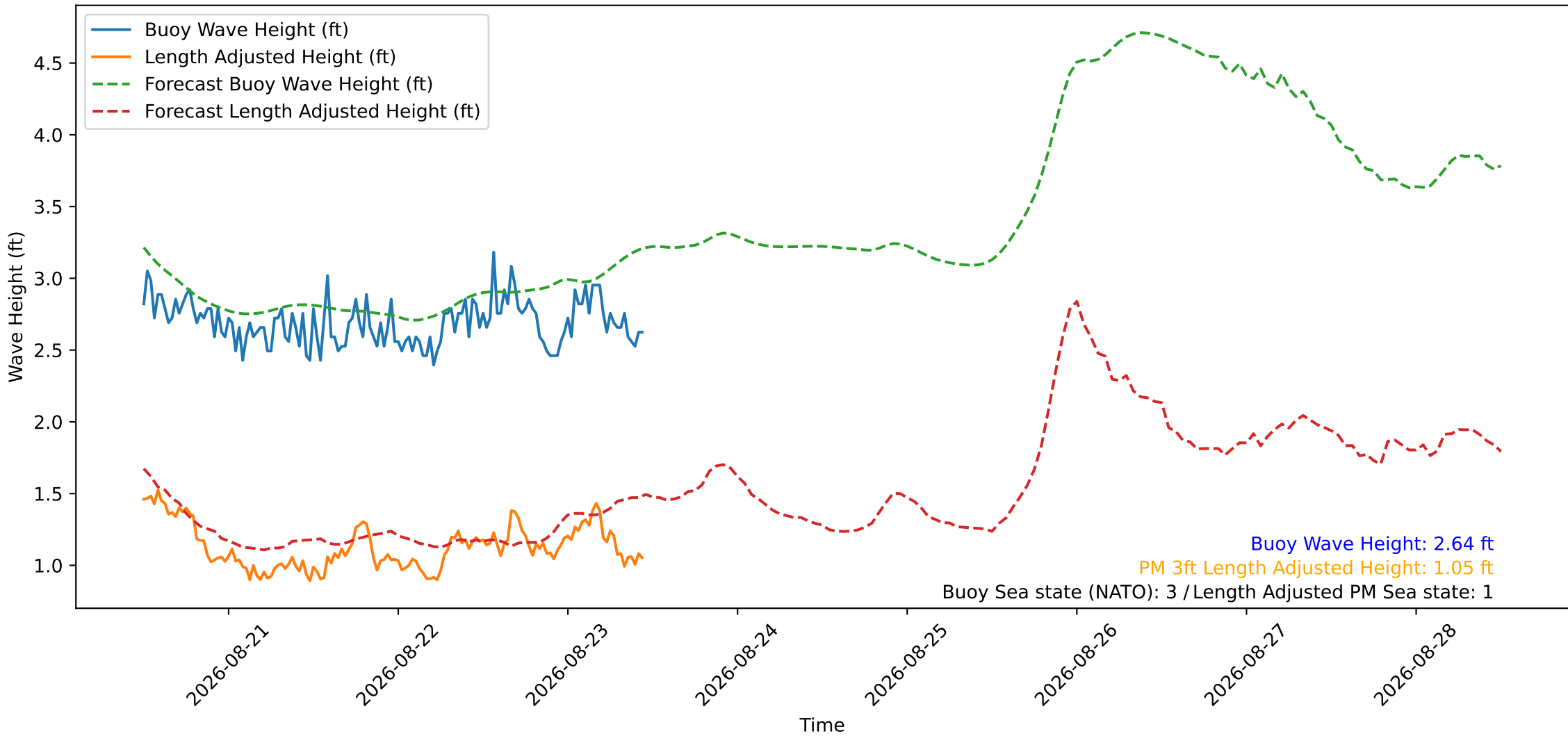
Wave Heights over Time for Green Beach at 2026-08-23 11:31:11
