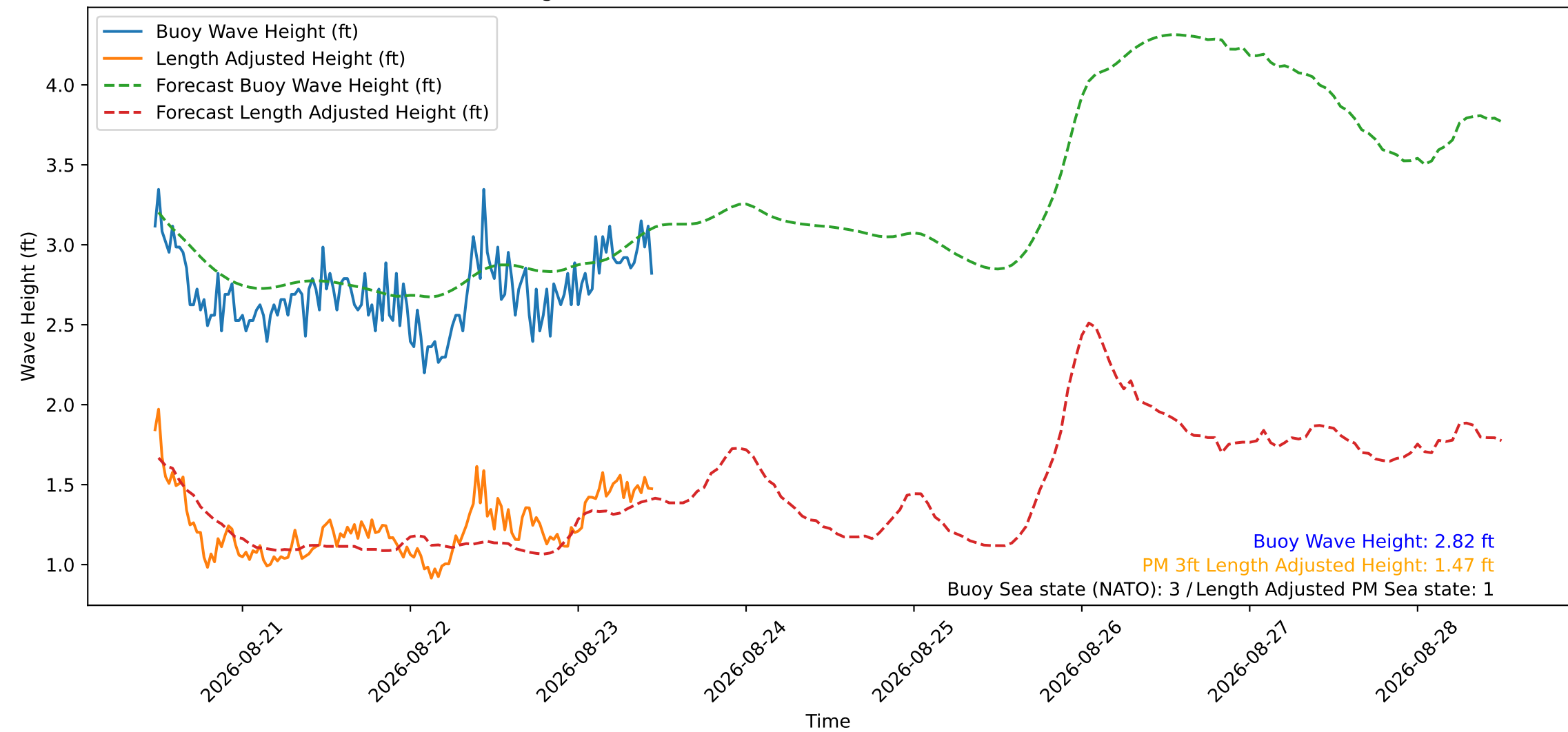
Wave Heights over Time for Oceanside Harbor at 2026-08-23 11:30:29
