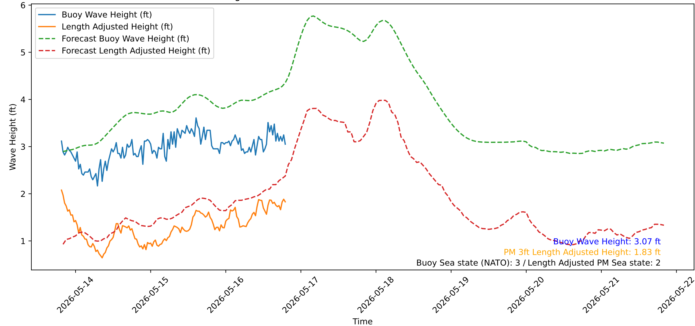
Wave Heights over Time for Oceanside Harbor at 2026-05-16 19:30:32
