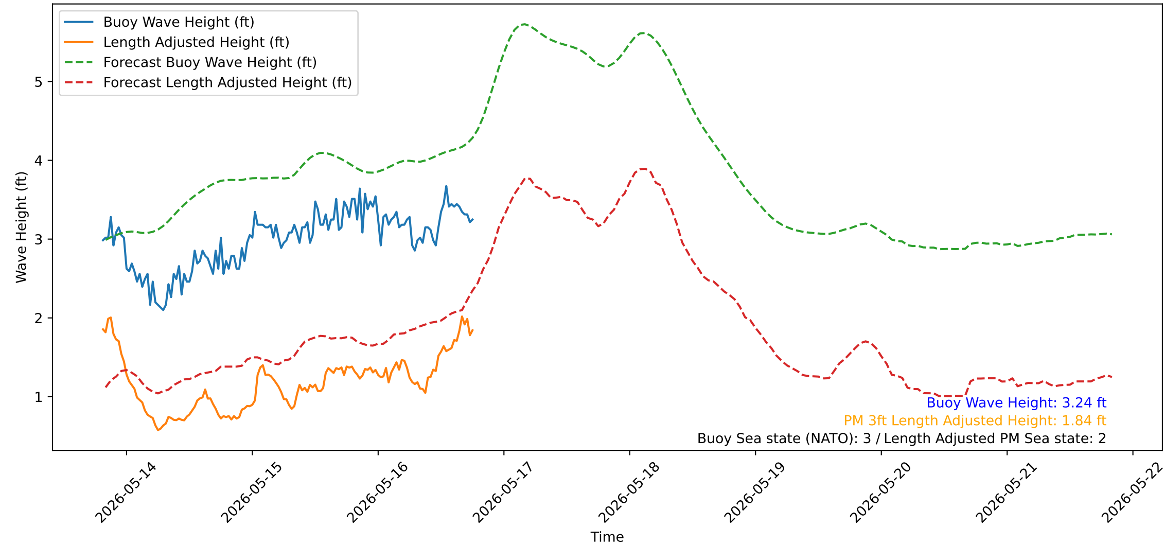
Wave Heights over Time for Green Beach at 2026-05-16 19:31:14
