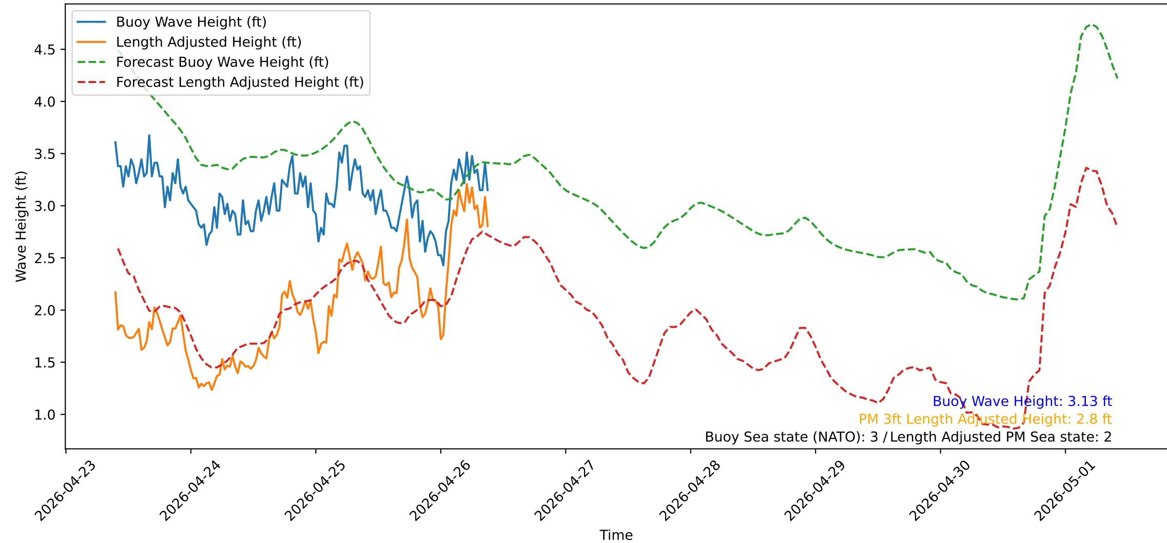
Wave Heights over Time for Green Beach at 2026-04-26 09:41:13
