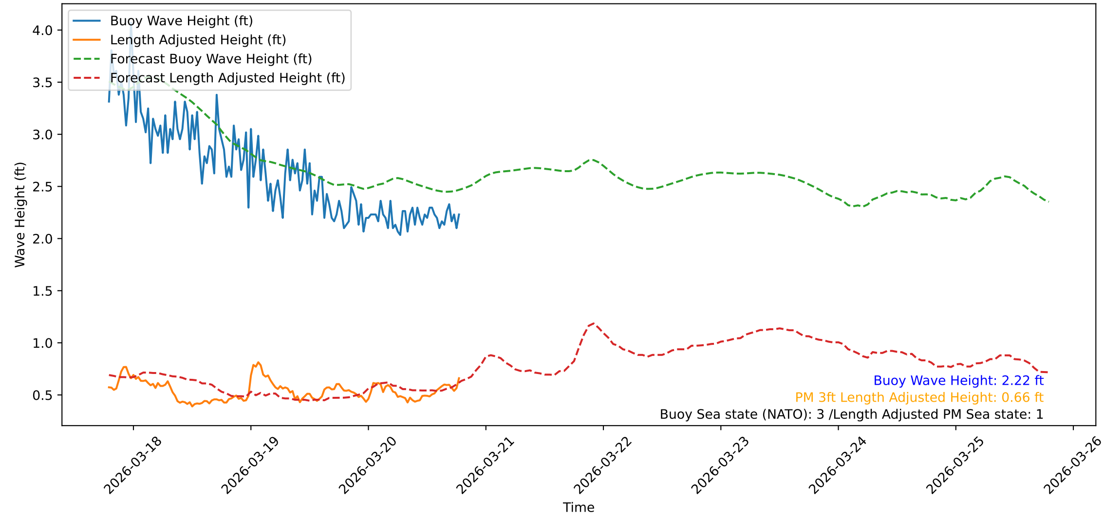
Wave Heights over Time for Green Beach at 2026-03-20 19:11:10
