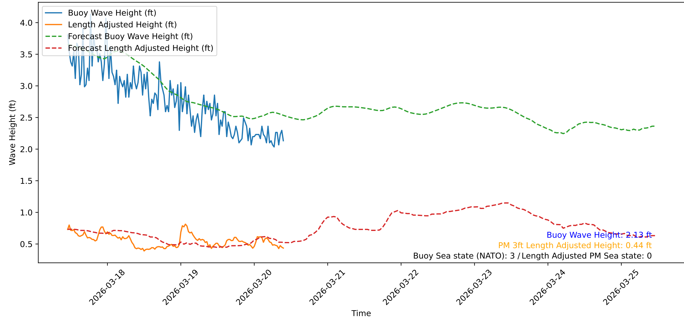
Wave Heights over Time for Green Beach at 2026-03-20 11:01:09
