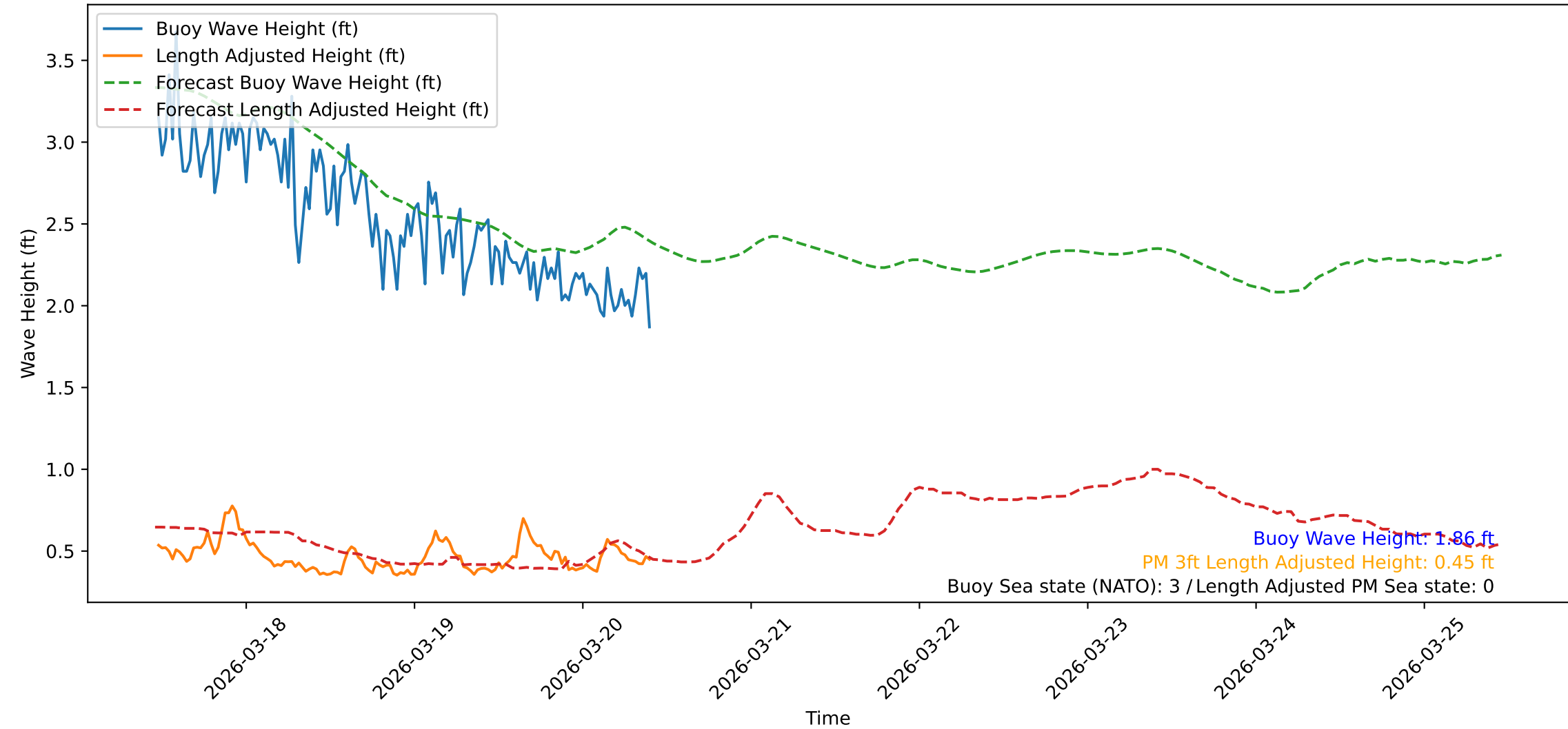
Wave Heights over Time for Red Beach at 2026-03-20 11:00:47
