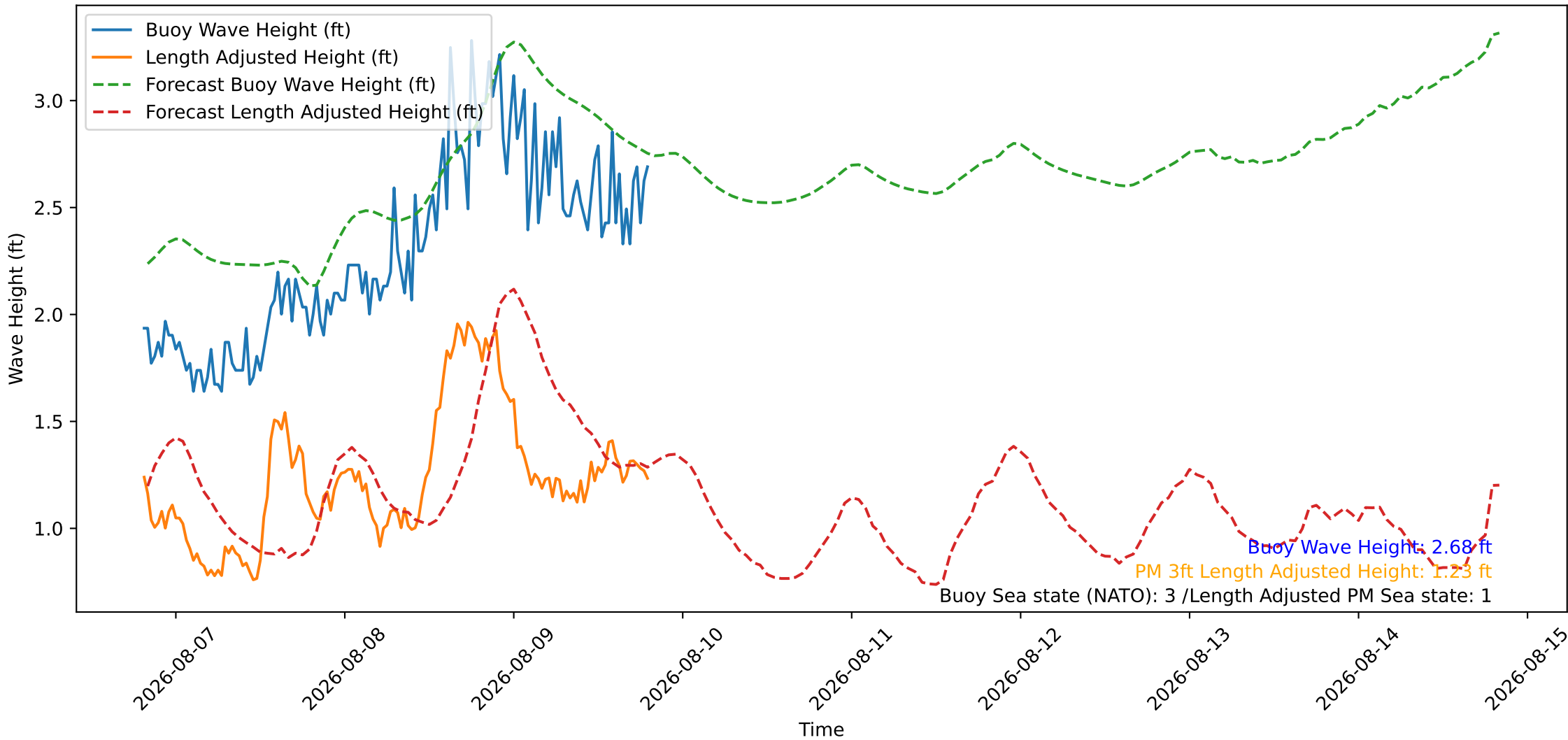
Wave Heights over Time for Oceanside Harbor at 2026-08-09 19:40:27
