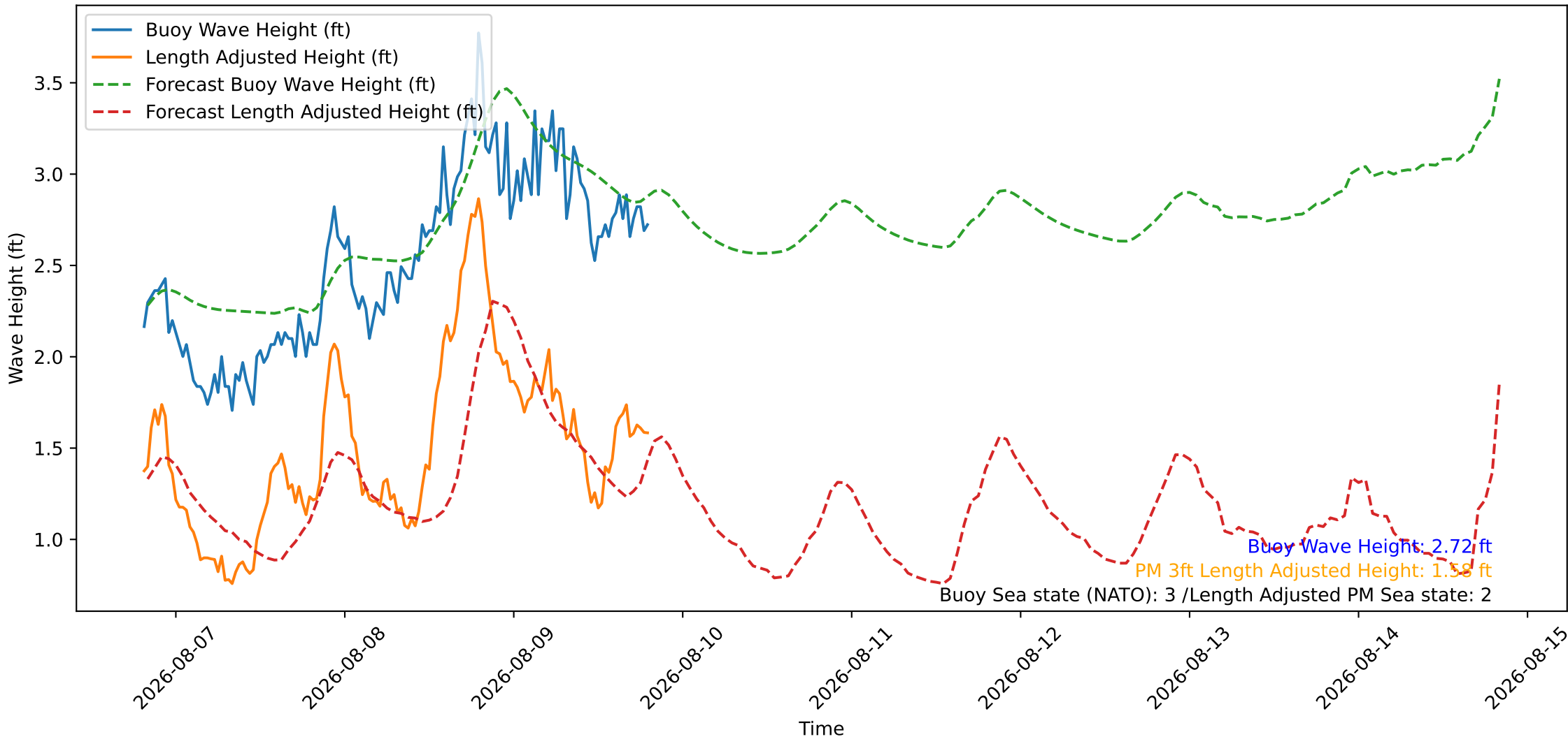
Wave Heights over Time for Green Beach at 2026-08-09 19:41:09
