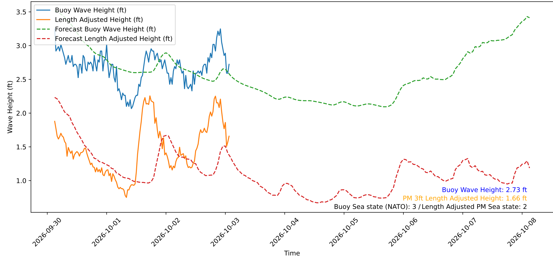
Wave Heights over Time for Red Beach at 2026-10-03 02:30:49
