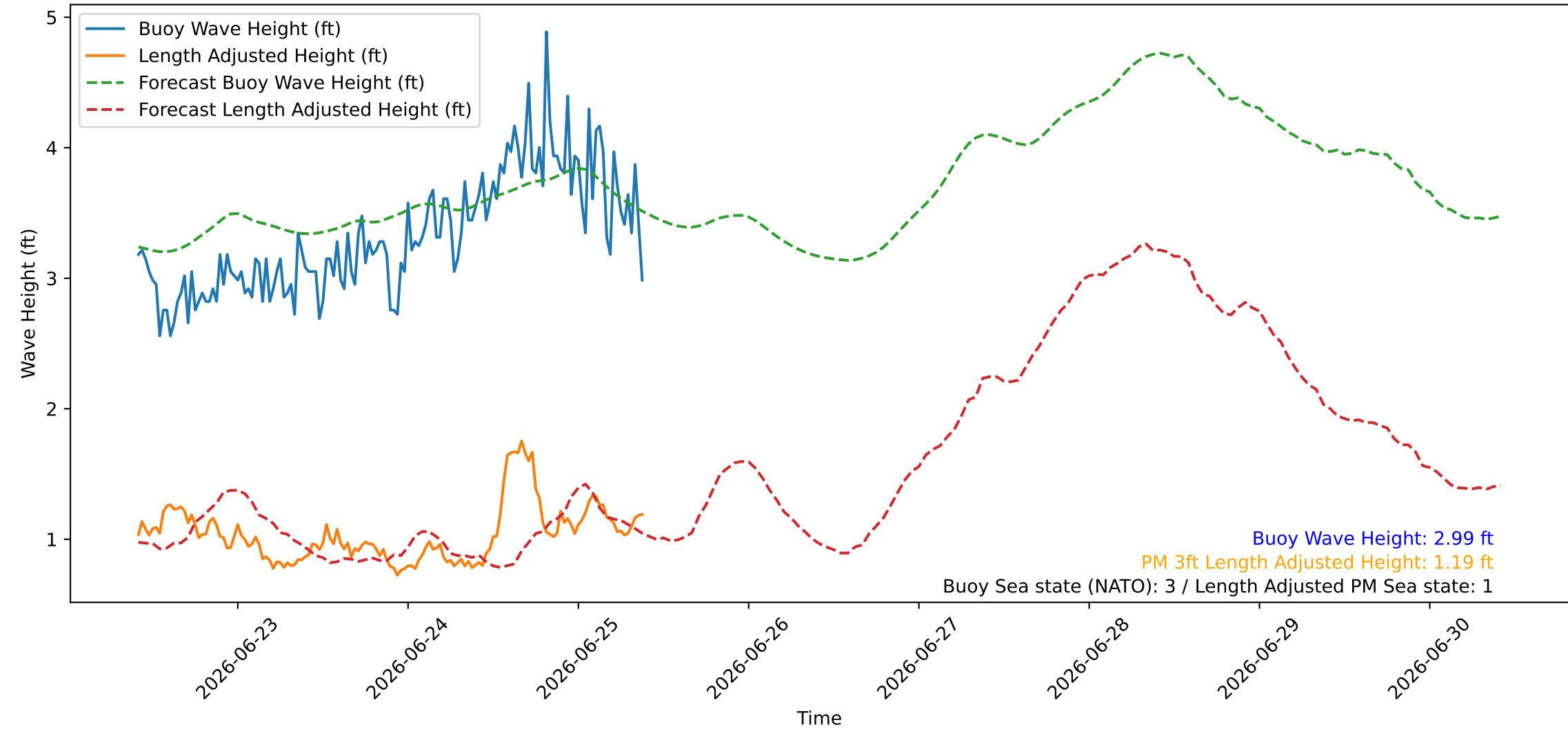
Wave Heights over Time for Oceanside Harbor at 2026-06-25 10:00:26
