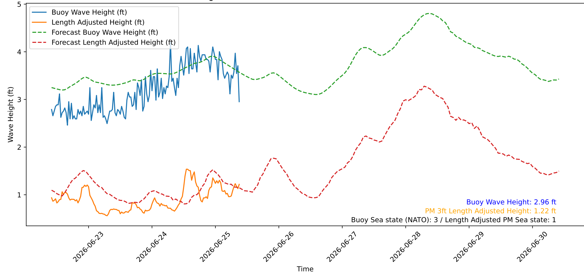
Wave Heights over Time for Green Beach at 2026-06-25 10:01:08
