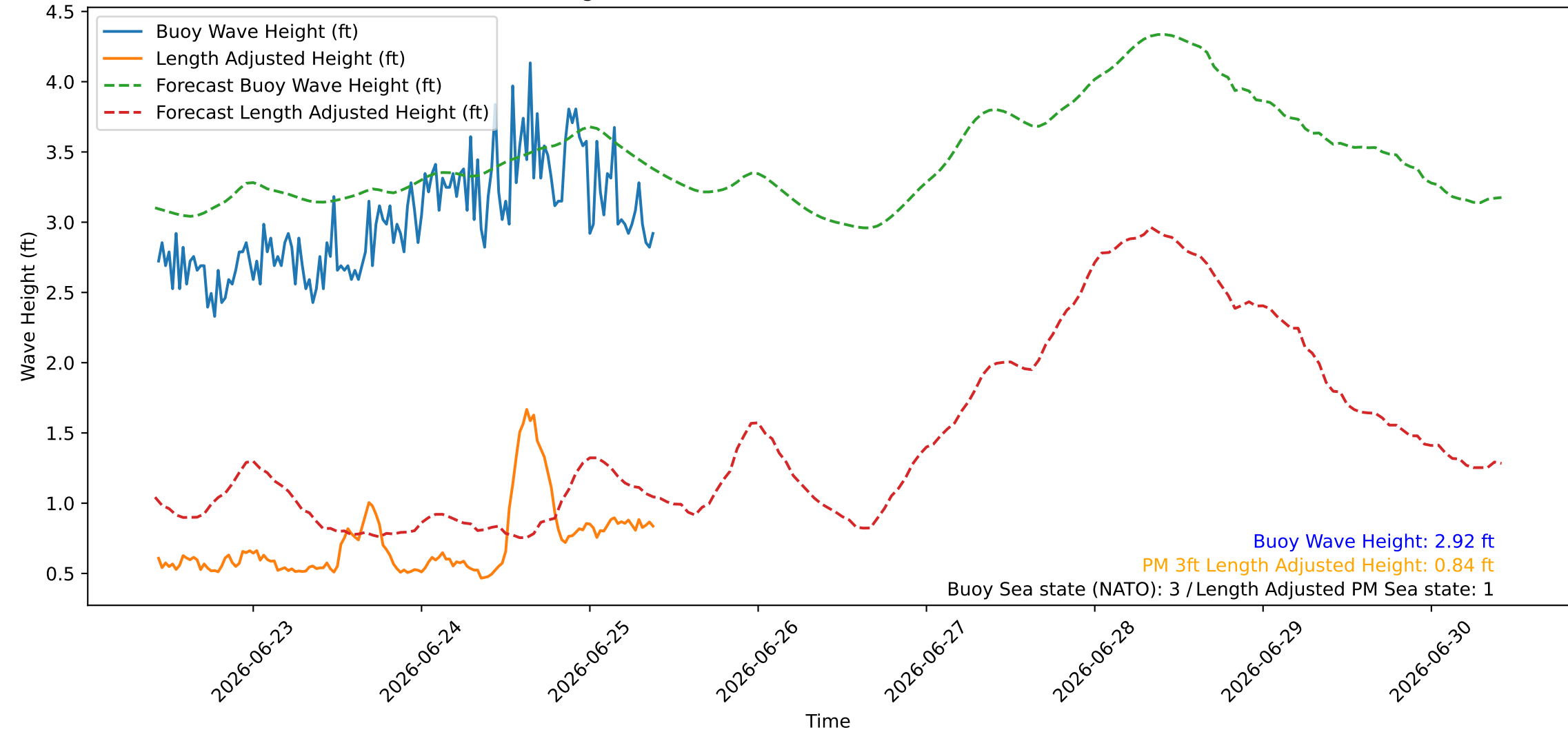
Wave Heights over Time for Red Beach at 2026-06-25 10:00:45
