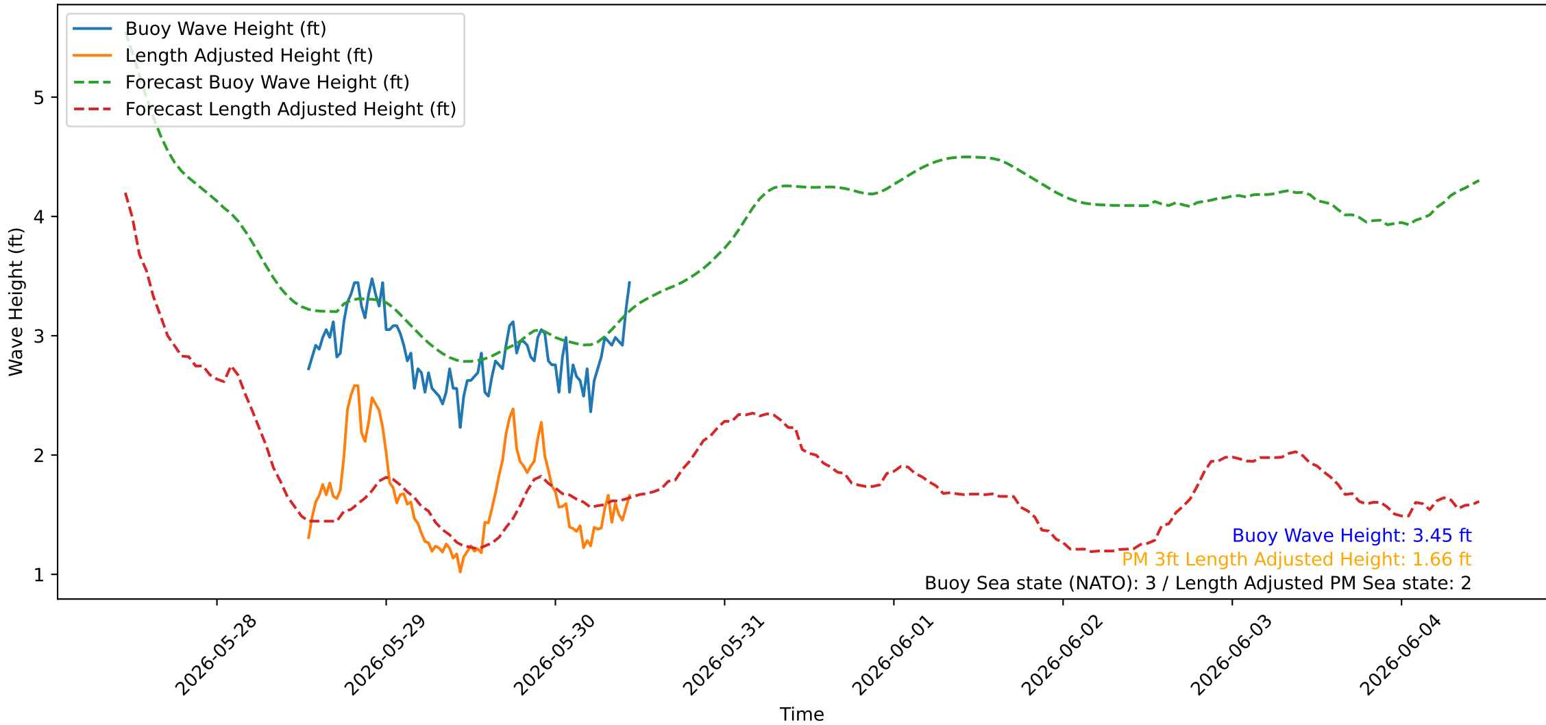
Wave Heights over Time for Oceanside Harbor at 2026-05-30 11:20:25
