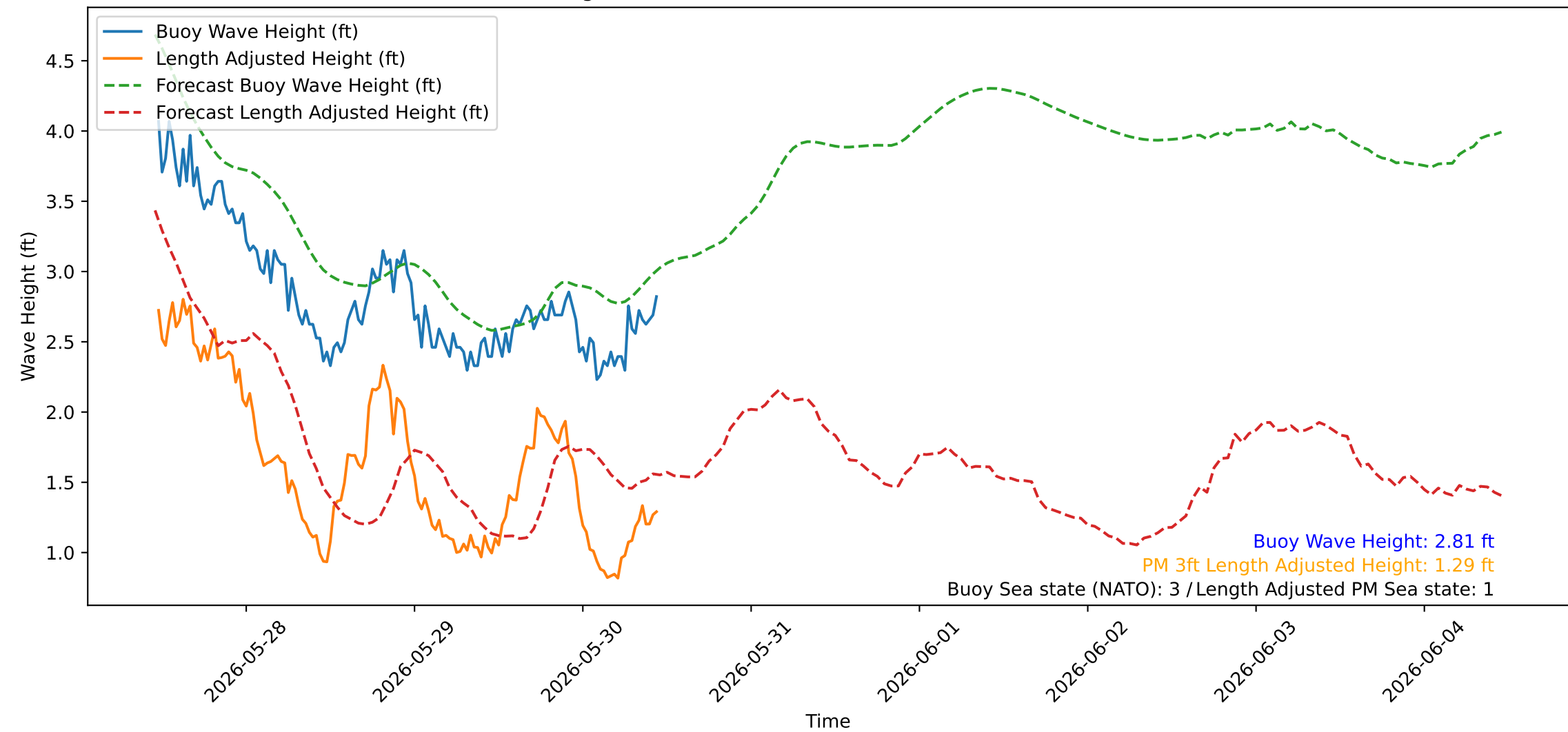
Wave Heights over Time for Red Beach at 2026-05-30 11:20:46
