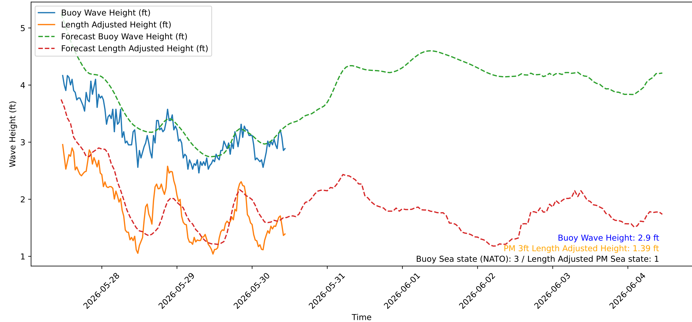
Wave Heights over Time for Green Beach at 2026-05-30 11:21:08
