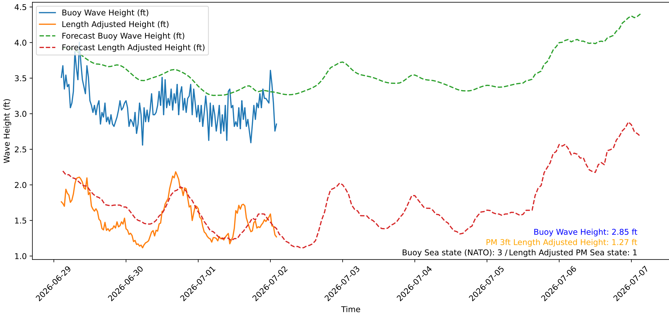
Wave Heights over Time for Oceanside Harbor at 2026-07-02 02:40:27
