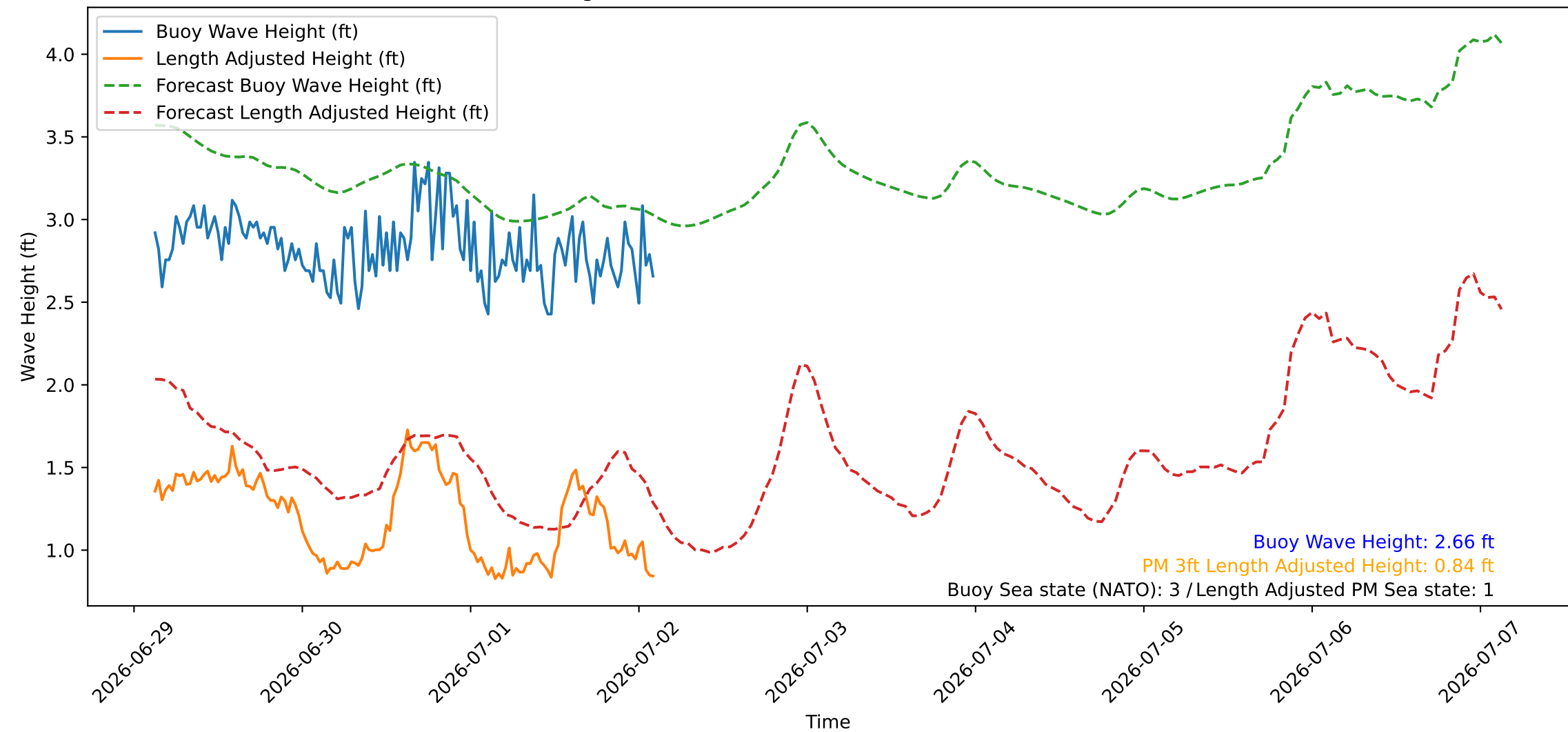
Wave Heights over Time for Red Beach at 2026-07-02 02:40:46
