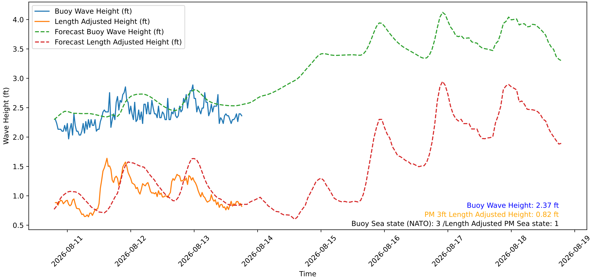
Wave Heights over Time for Red Beach at 2026-08-13 19:20:47
