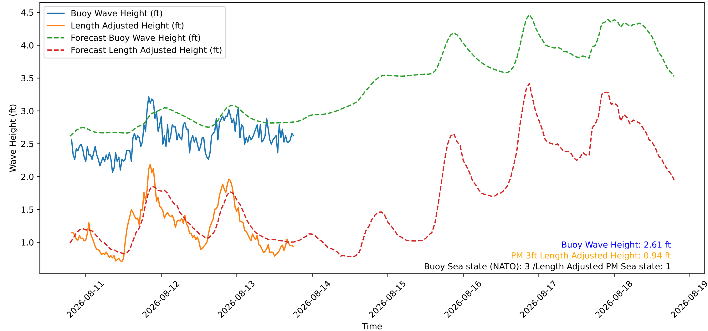
Wave Heights over Time for Green Beach at 2026-08-13 19:21:09
