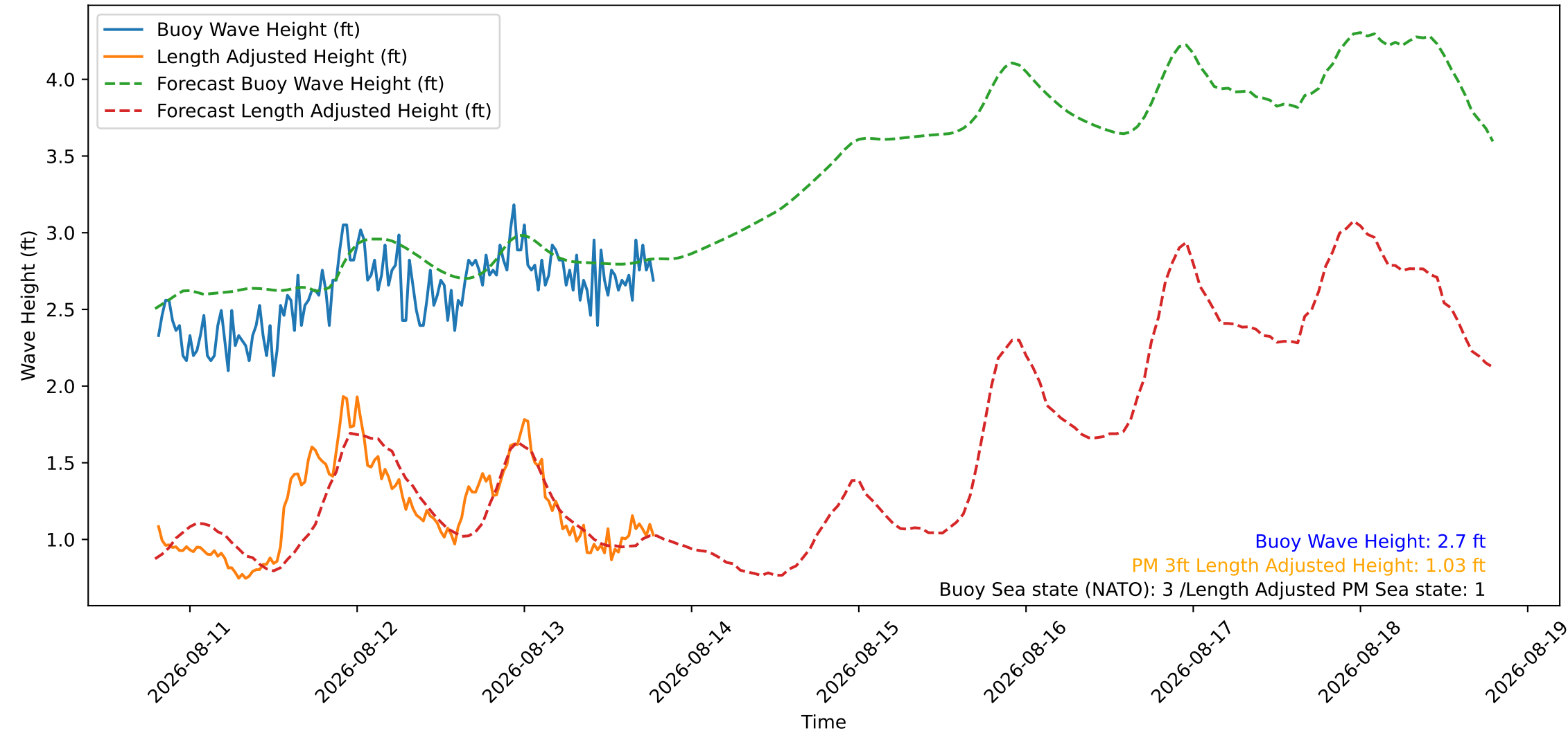
Wave Heights over Time for Oceanside Harbor at 2026-08-13 19:20:26
