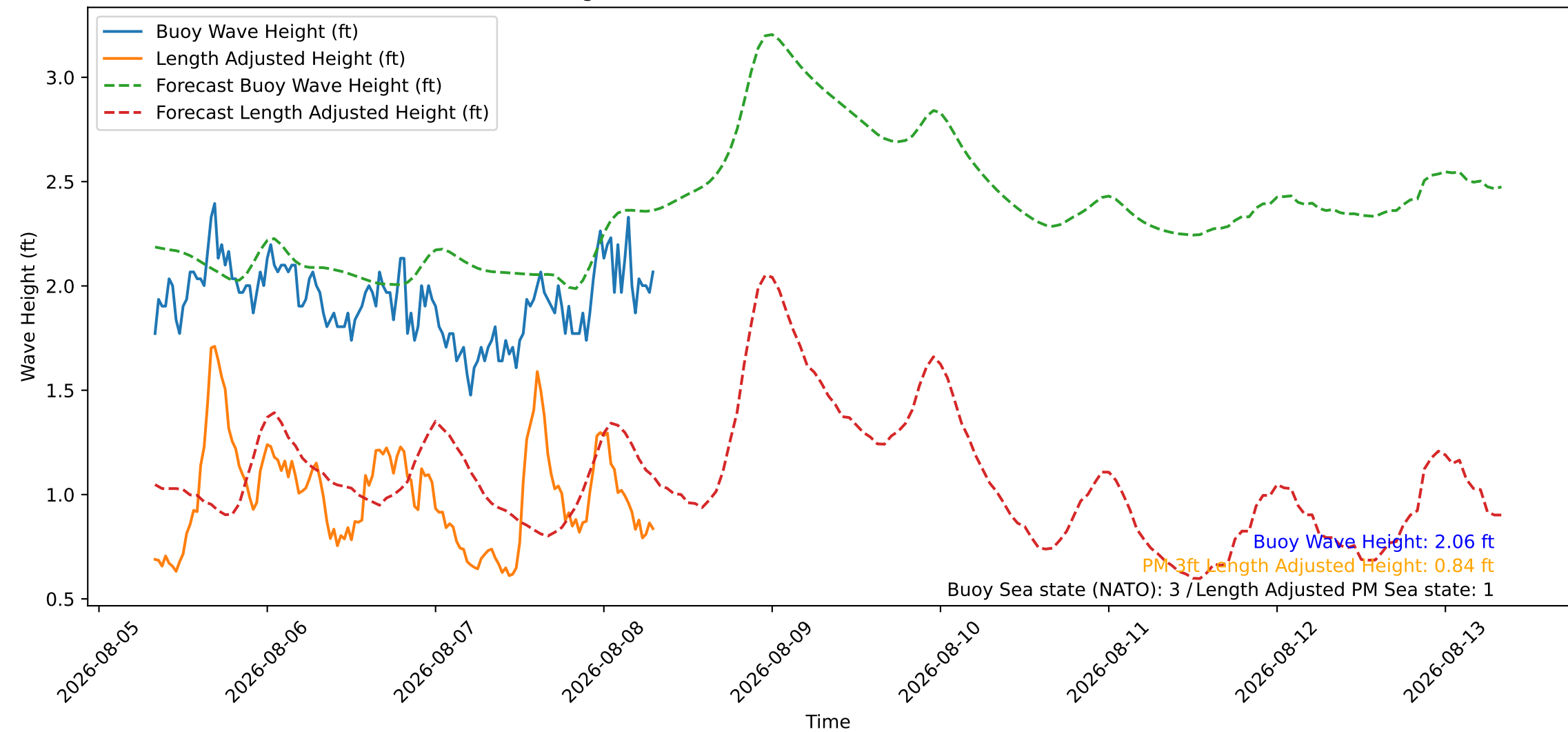
Wave Heights over Time for Red Beach at 2026-08-08 07:50:48
