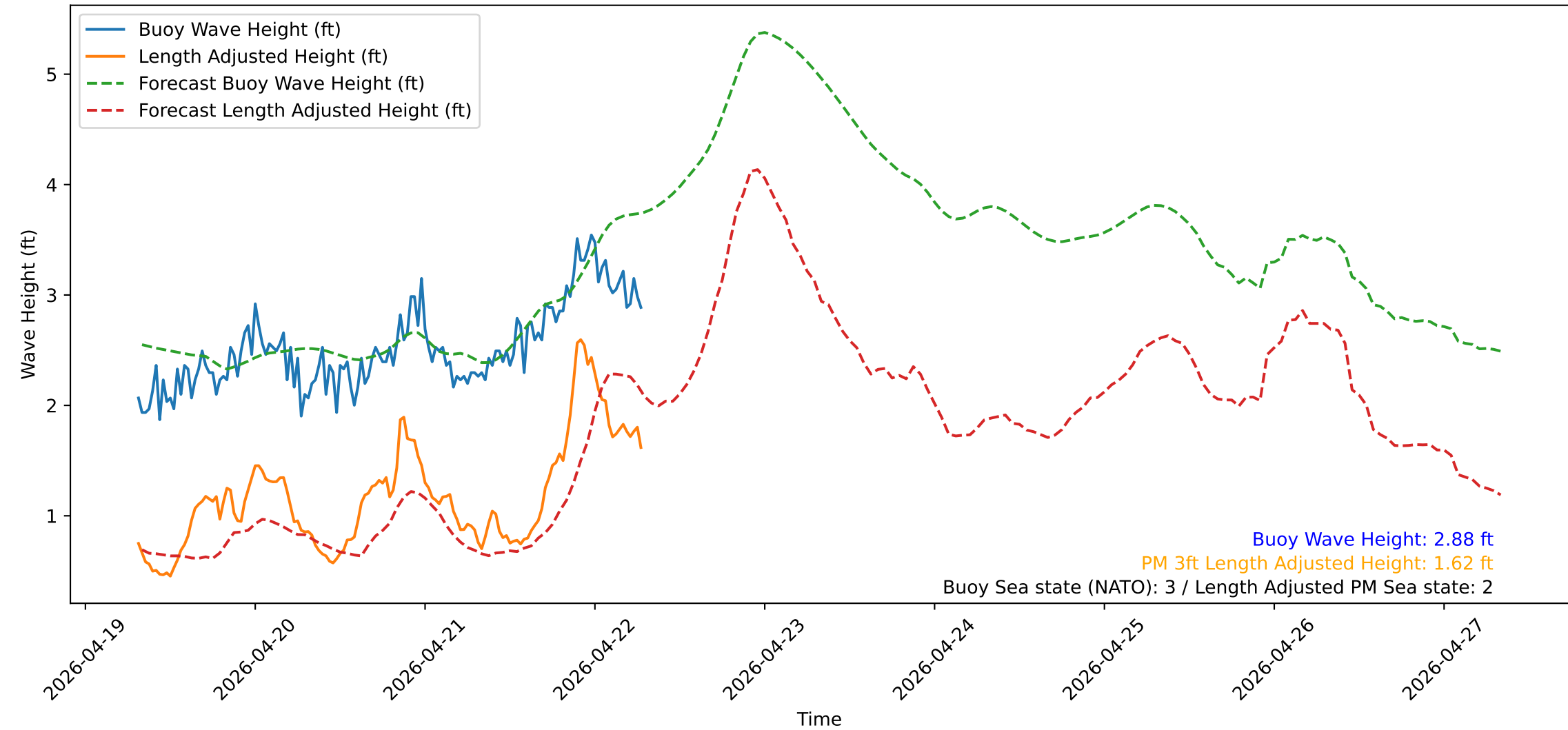
Wave Heights over Time for Green Beach at 2026-04-22 07:31:11
