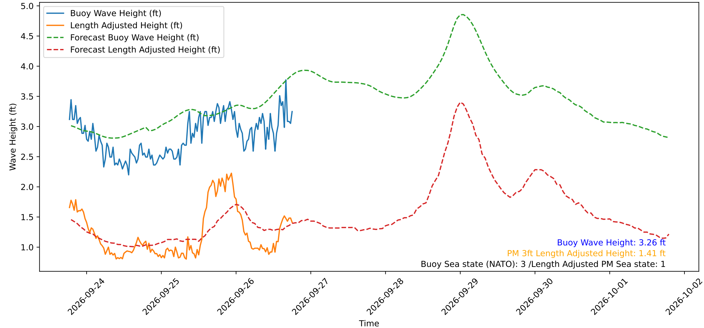
Wave Heights over Time for Oceanside Harbor at 2026-09-26 18:40:29
