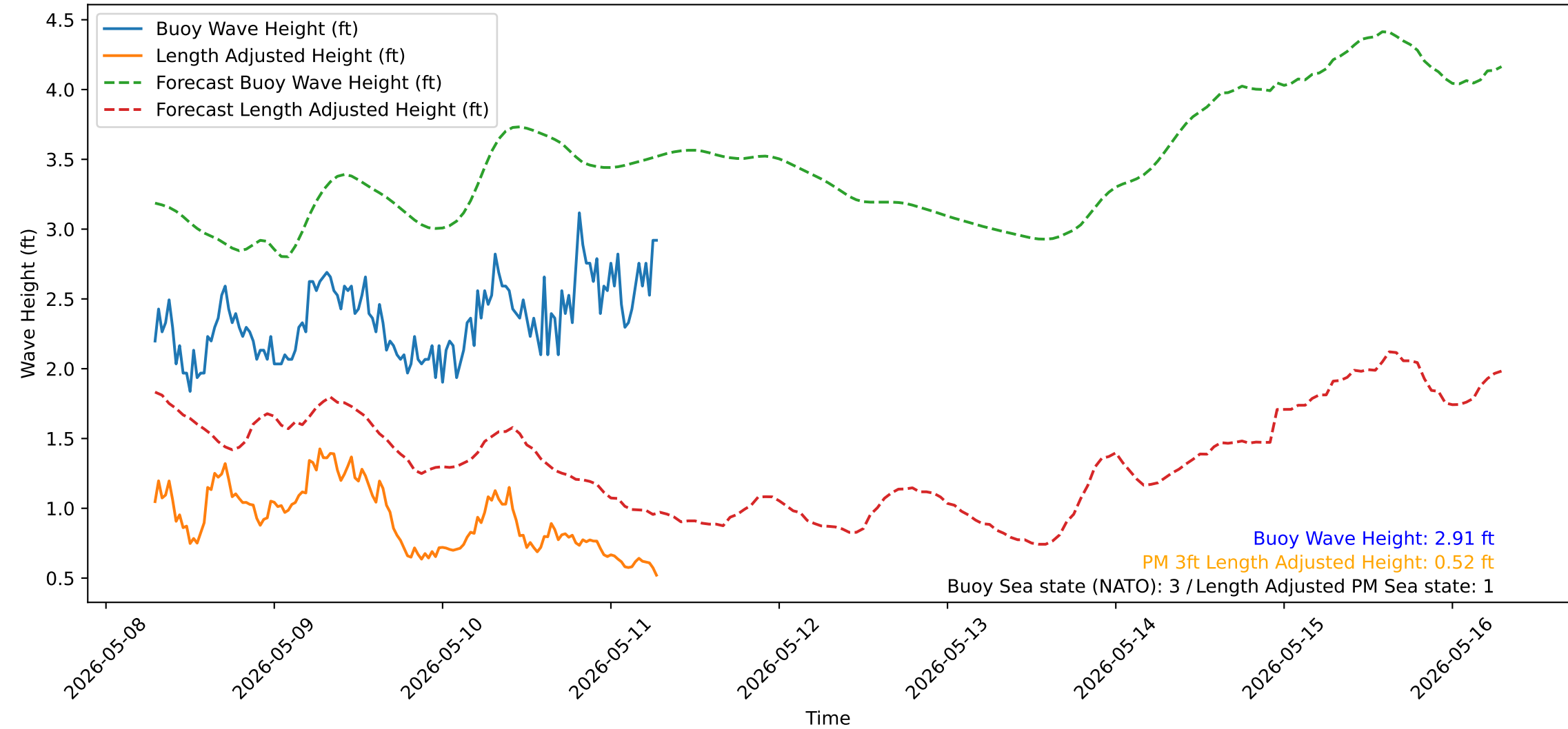
Wave Heights over Time for Green Beach at 2026-05-11 07:11:13
