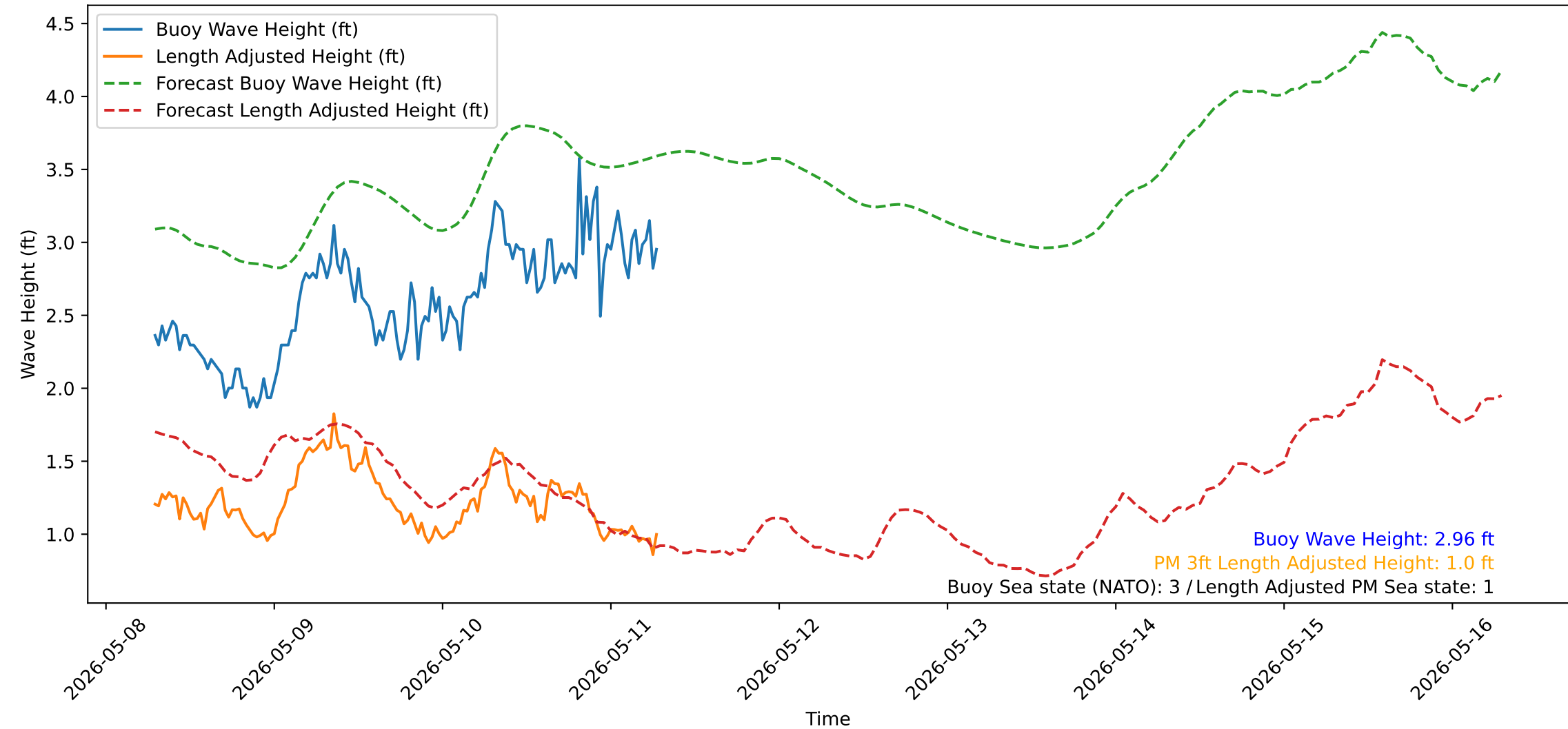
Wave Heights over Time for Oceanside Harbor at 2026-05-11 07:10:31
