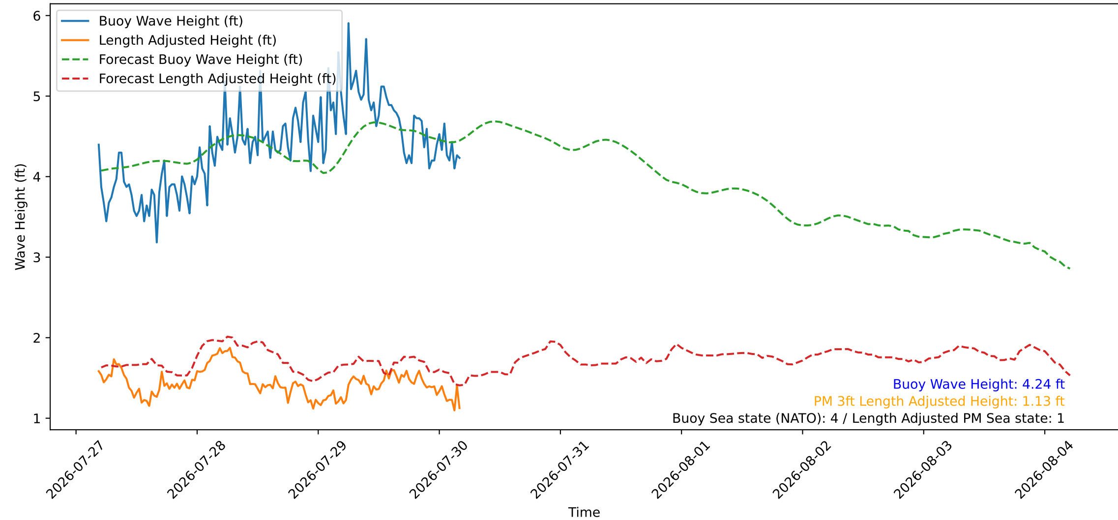
Wave Heights over Time for Oceanside Harbor at 2026-07-30 04:30:26
