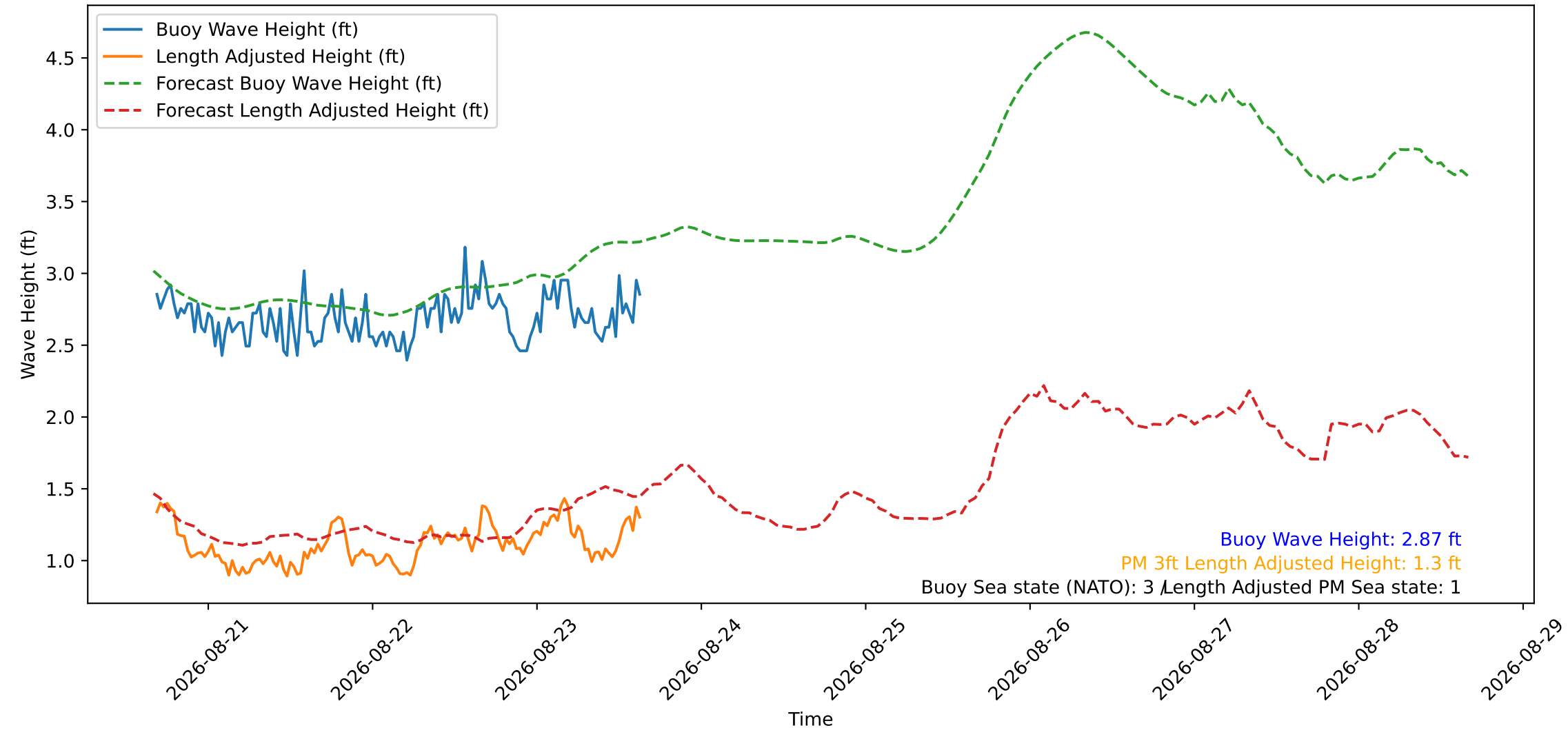
Wave Heights over Time for Green Beach at 2026-08-23 16:01:12
