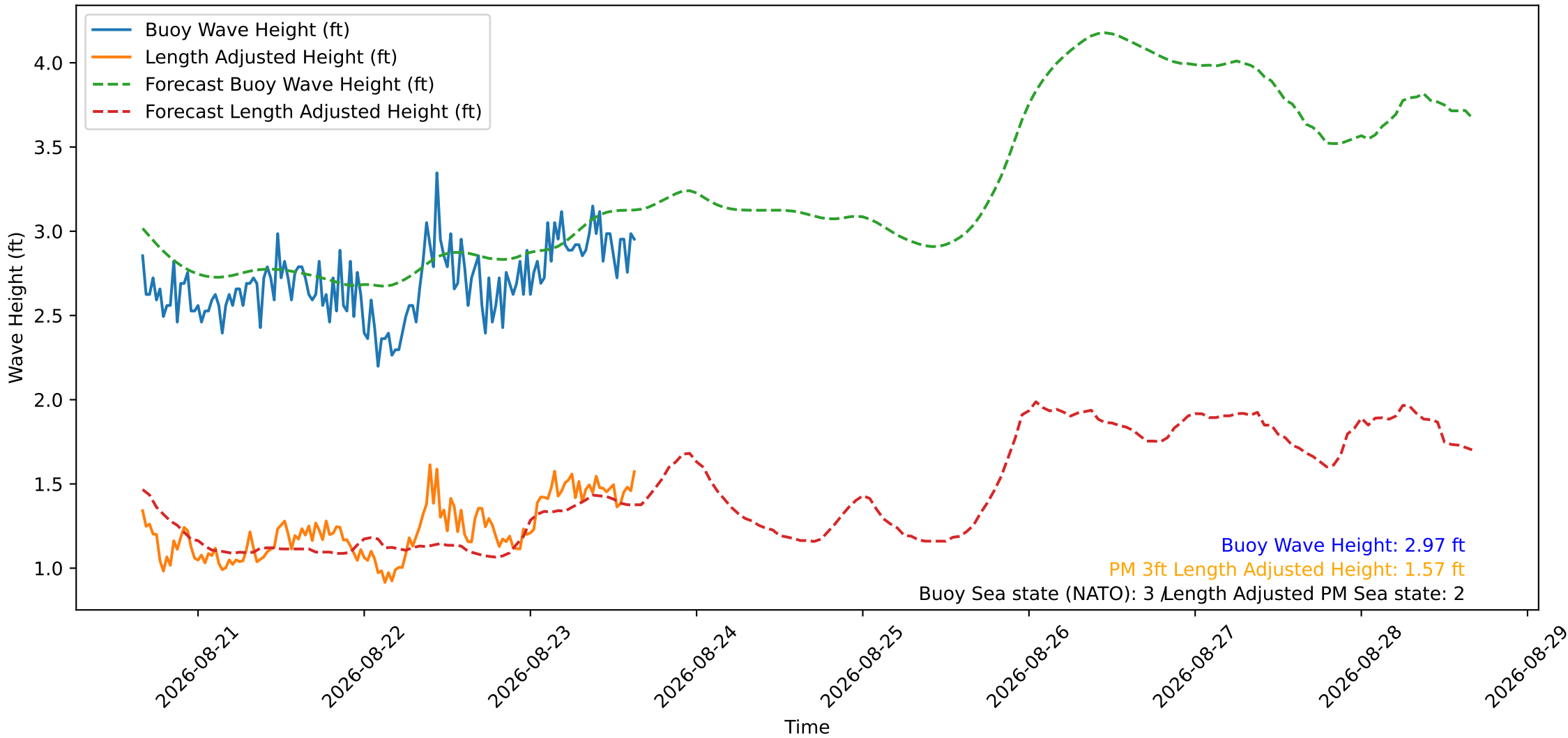
Wave Heights over Time for Oceanside Harbor at 2026-08-23 16:00:30
