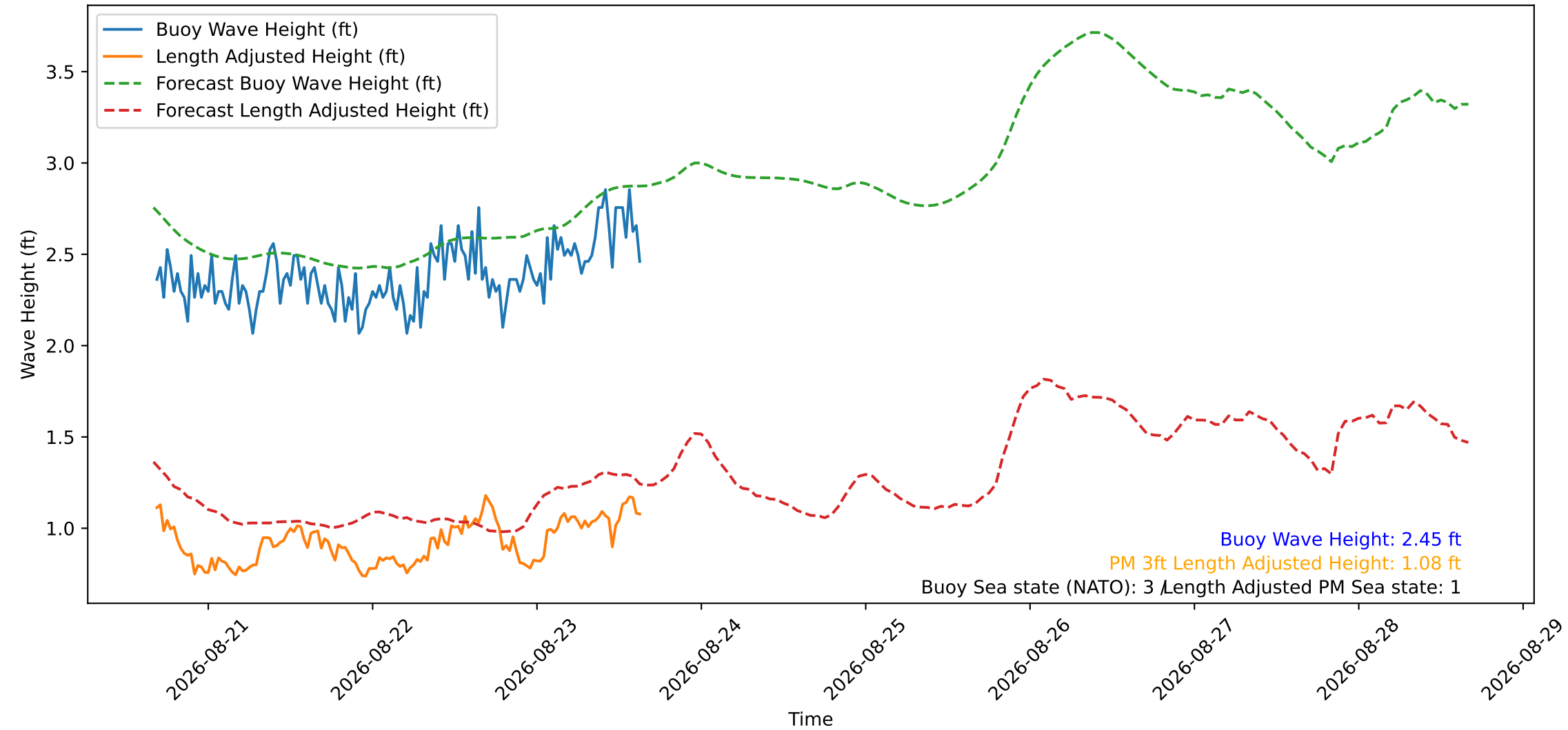
Wave Heights over Time for Red Beach at 2026-08-23 16:00:49
