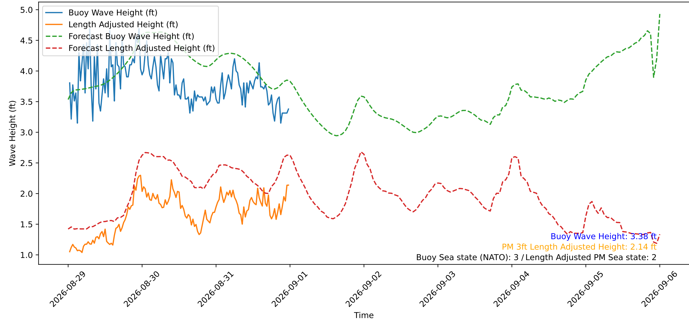
Wave Heights over Time for Red Beach at 2026-09-01 00:20:50
