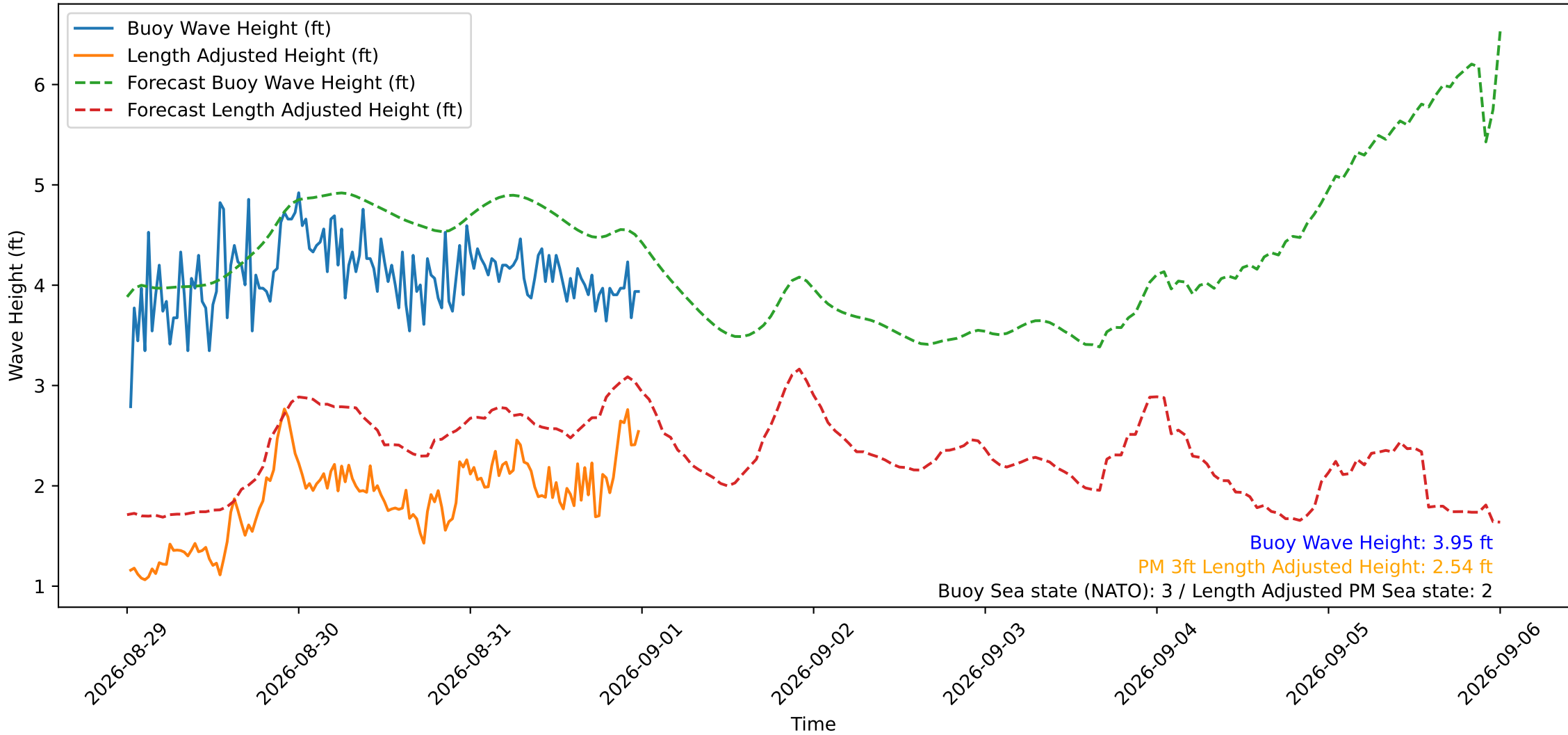
Wave Heights over Time for Green Beach at 2026-09-01 00:21:15
