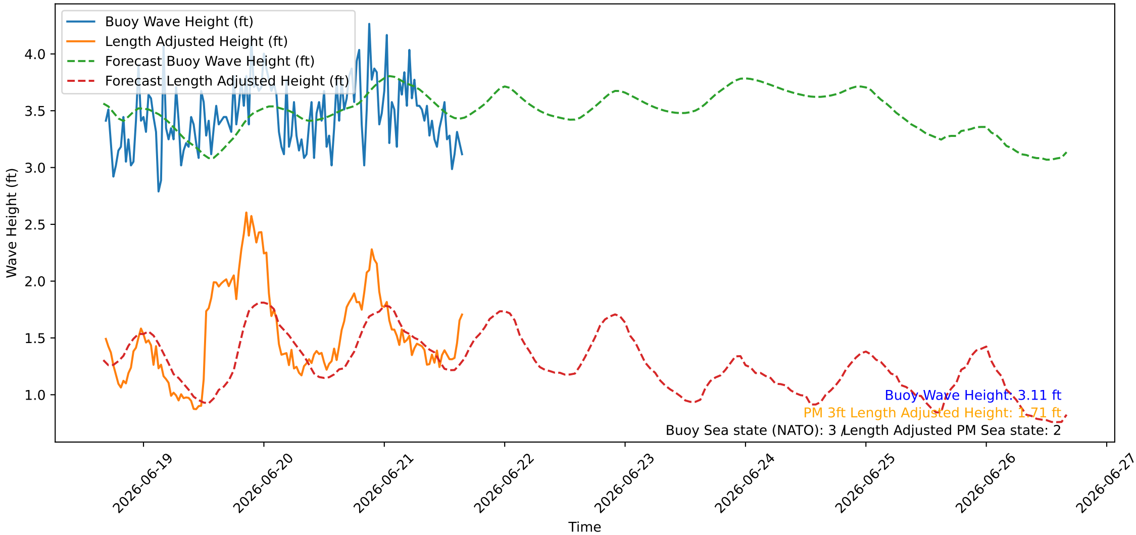
Wave Heights over Time for Oceanside Harbor at 2026-06-21 16:20:26
