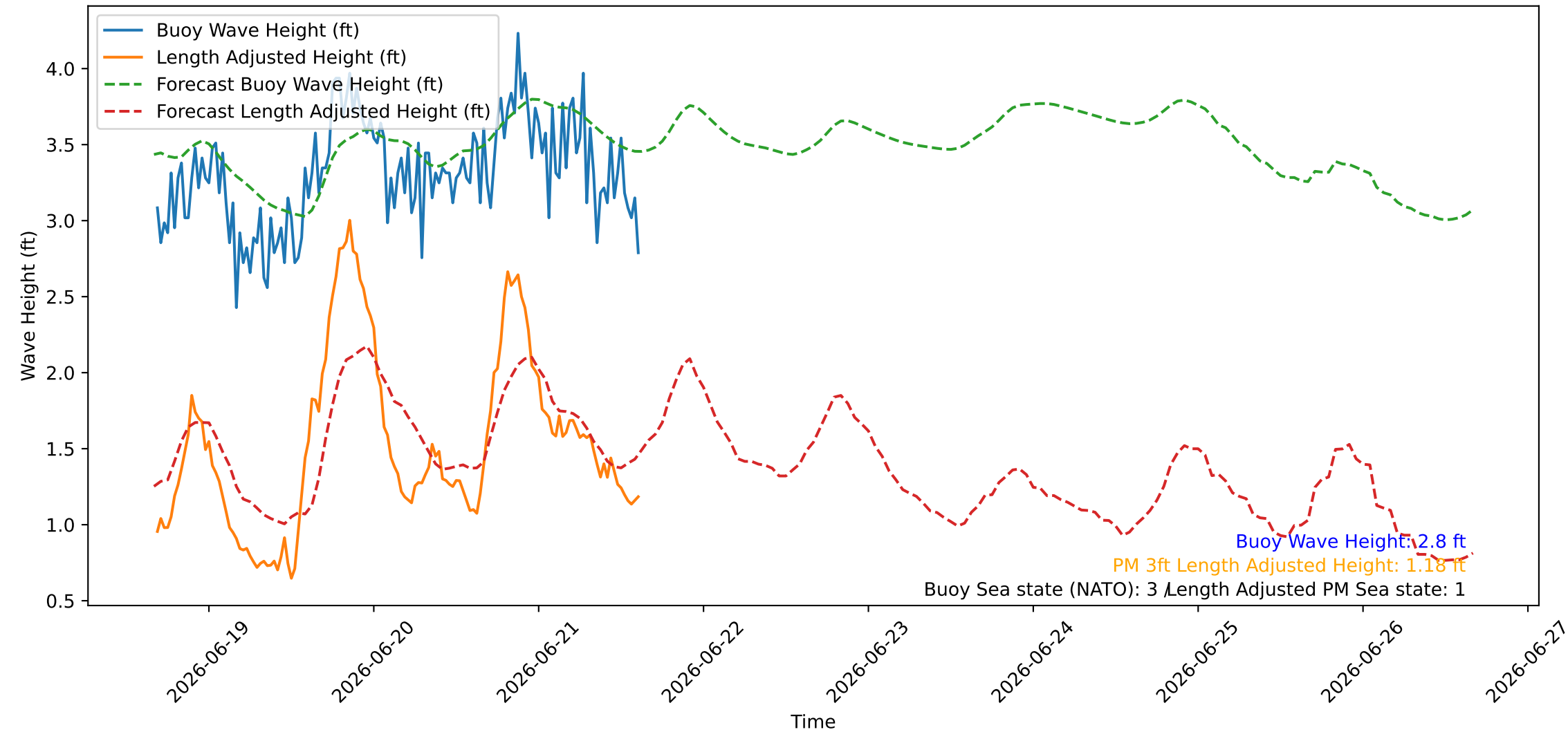
Wave Heights over Time for Green Beach at 2026-06-21 16:21:09
