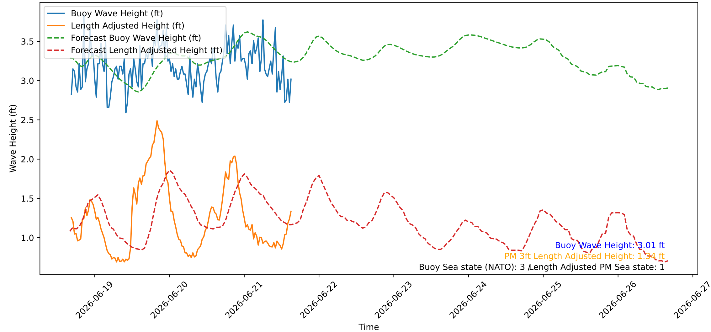
Wave Heights over Time for Red Beach at 2026-06-21 16:20:46
