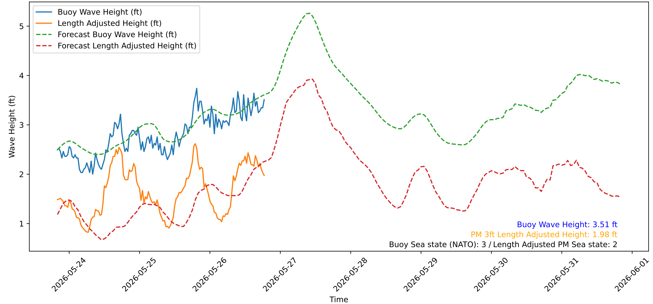
Wave Heights over Time for Red Beach at 2026-05-26 19:40:47
