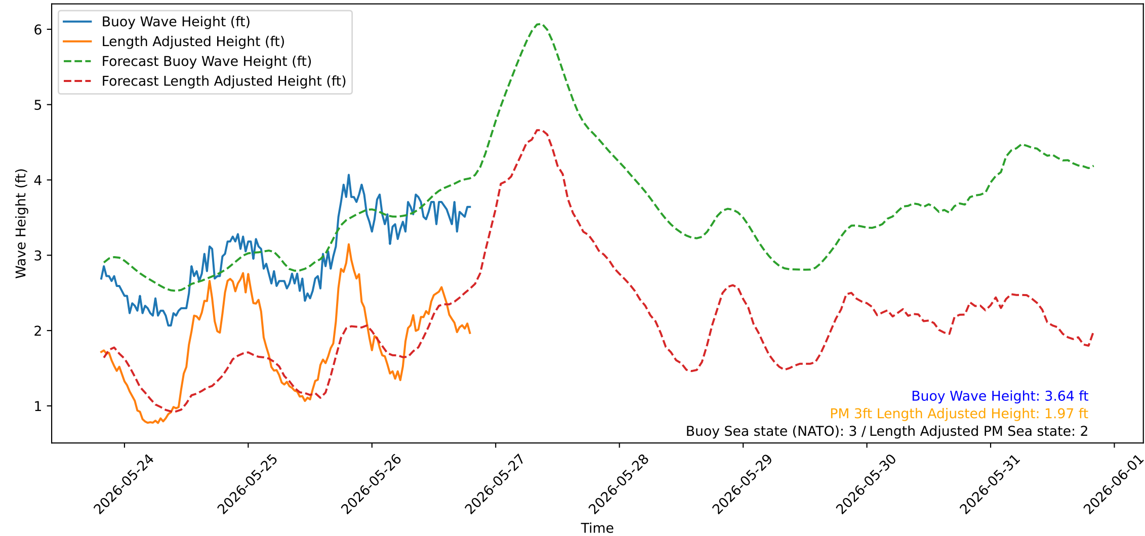
Wave Heights over Time for Green Beach at 2026-05-26 19:41:10
