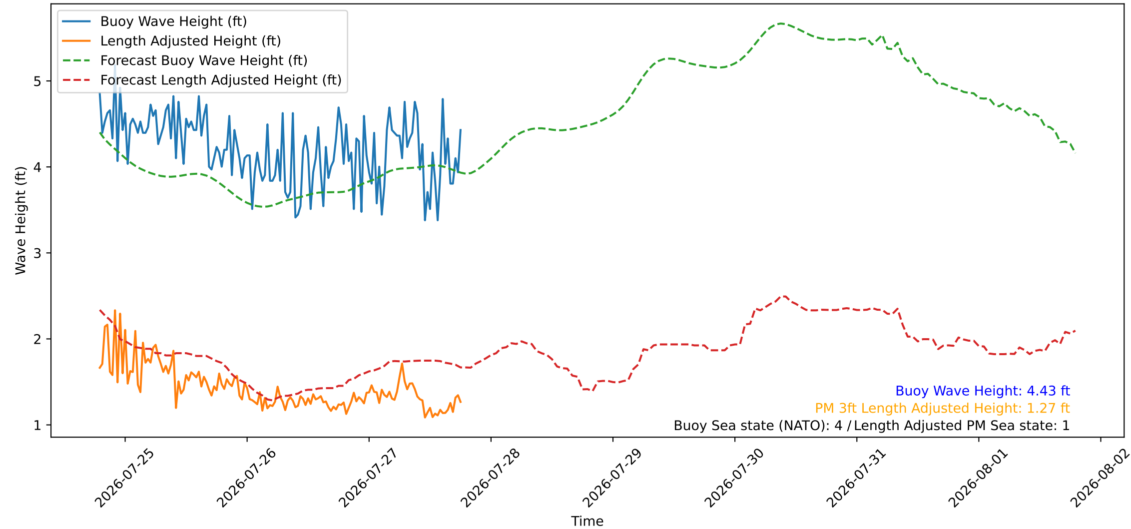
Wave Heights over Time for Green Beach at 2026-07-27 18:51:11
