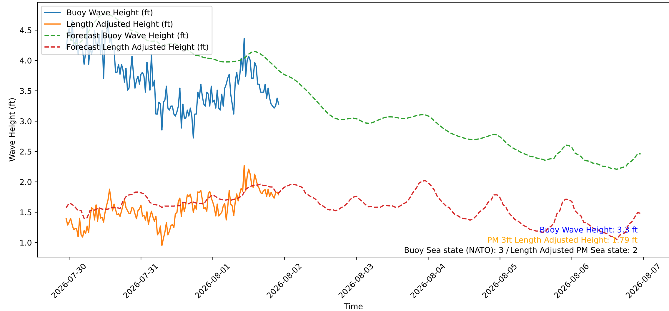
Wave Heights over Time for Oceanside Harbor at 2026-08-01 22:50:26
