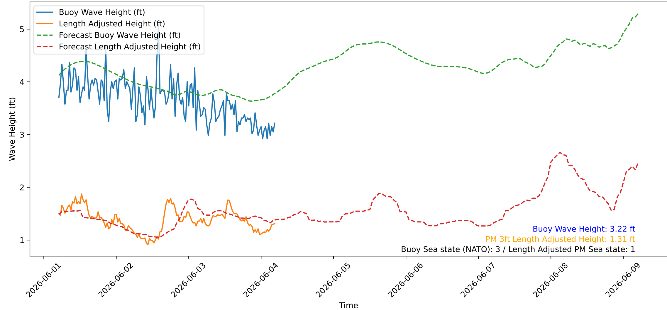
Wave Heights over Time for Oceanside Harbor at 2026-06-04 05:10:26
