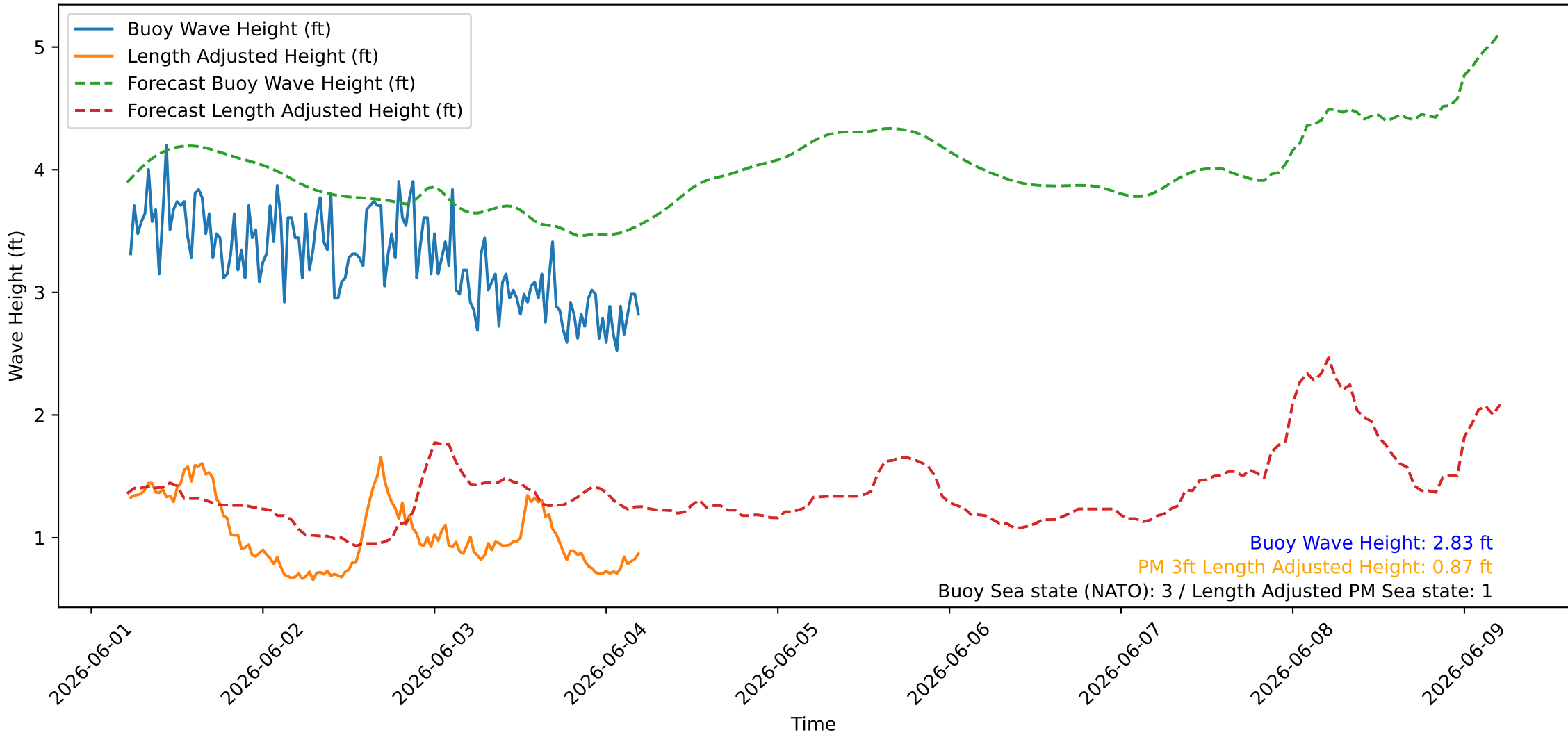
Wave Heights over Time for Red Beach at 2026-06-04 05:10:45
