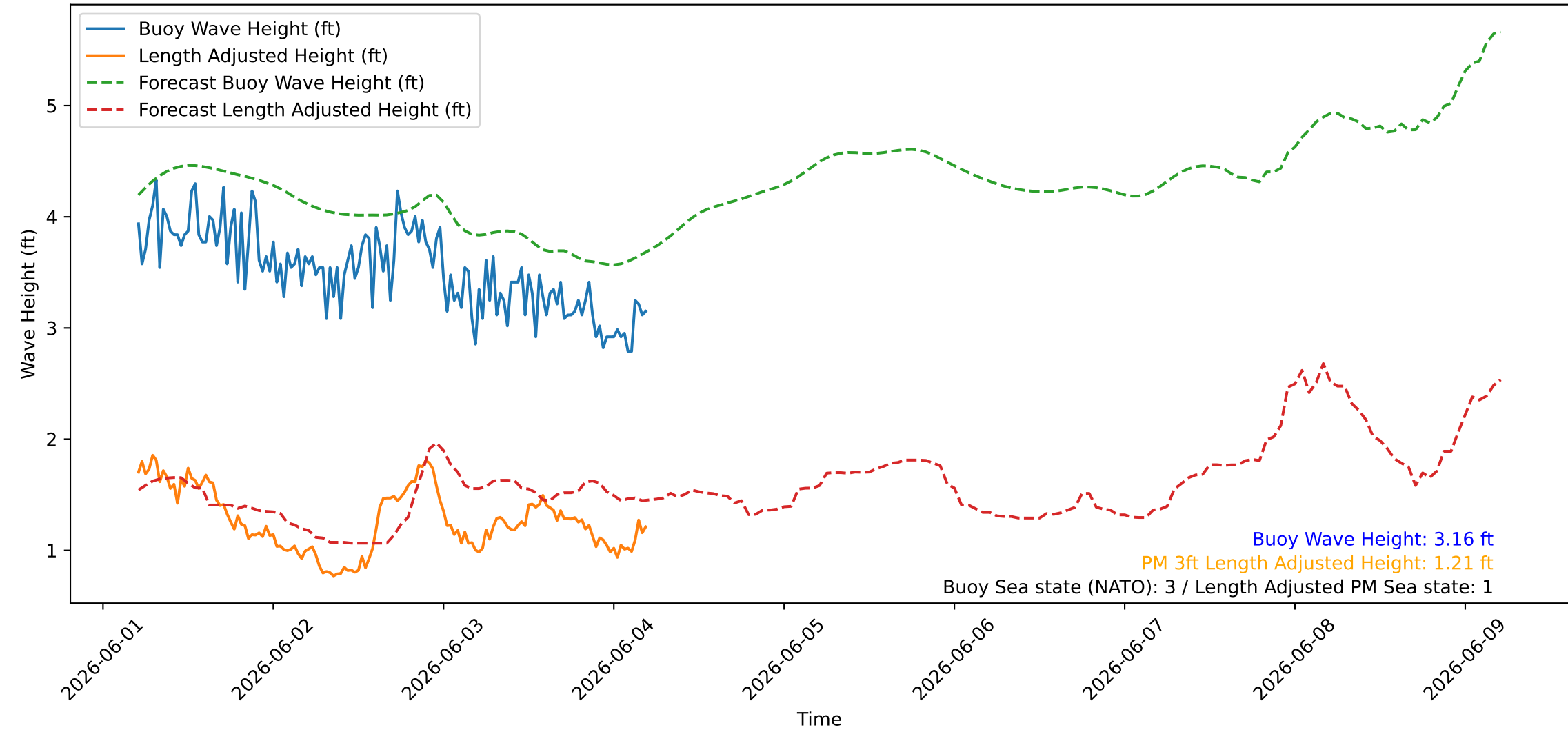
Wave Heights over Time for Green Beach at 2026-06-04 05:11:07
