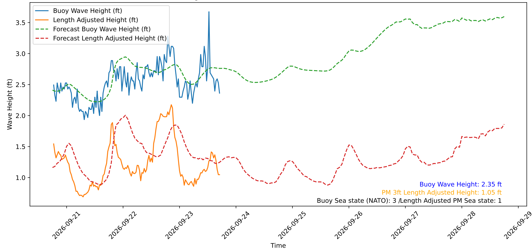
Wave Heights over Time for Red Beach at 2026-09-23 18:00:49
