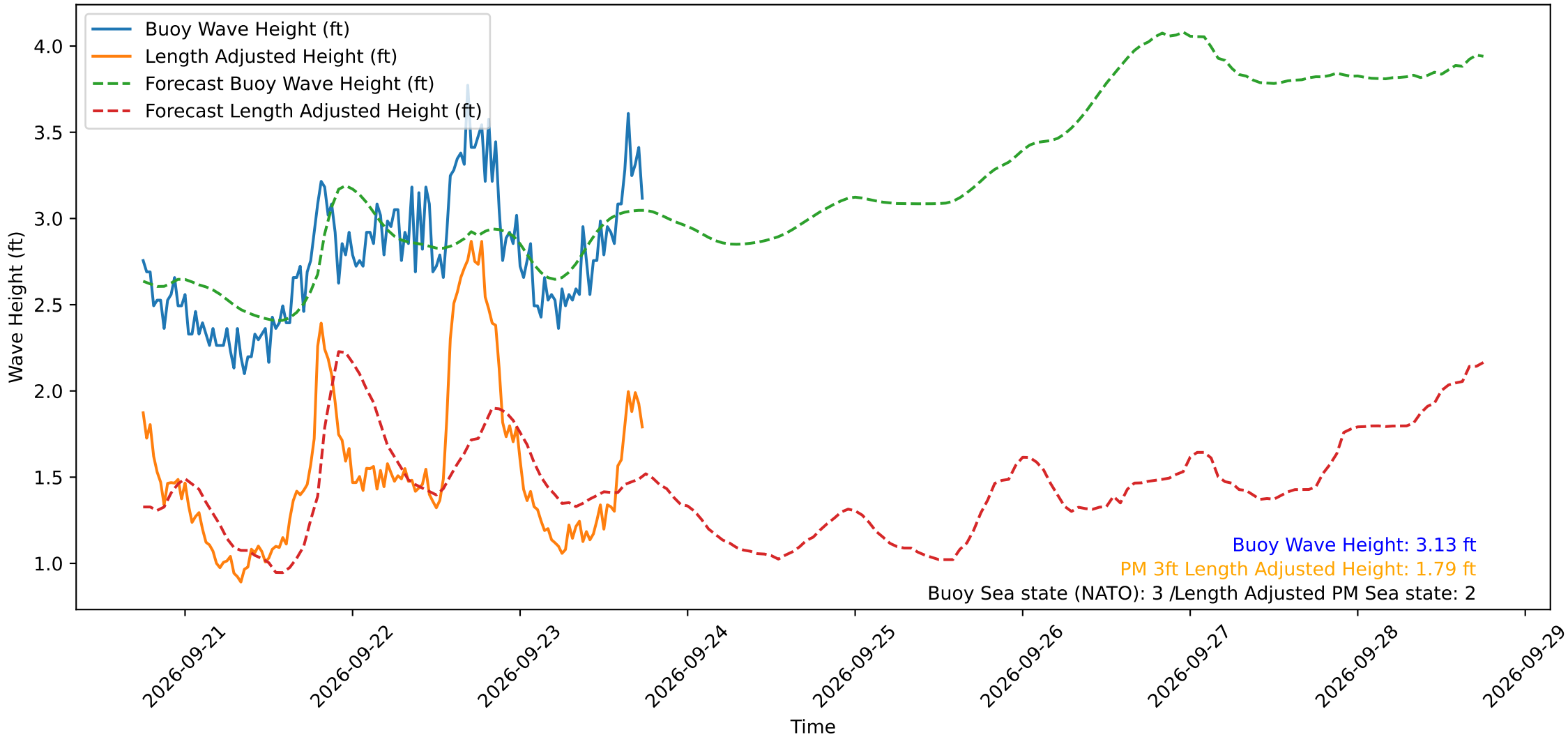
Wave Heights over Time for Oceanside Harbor at 2026-09-23 18:00:29
