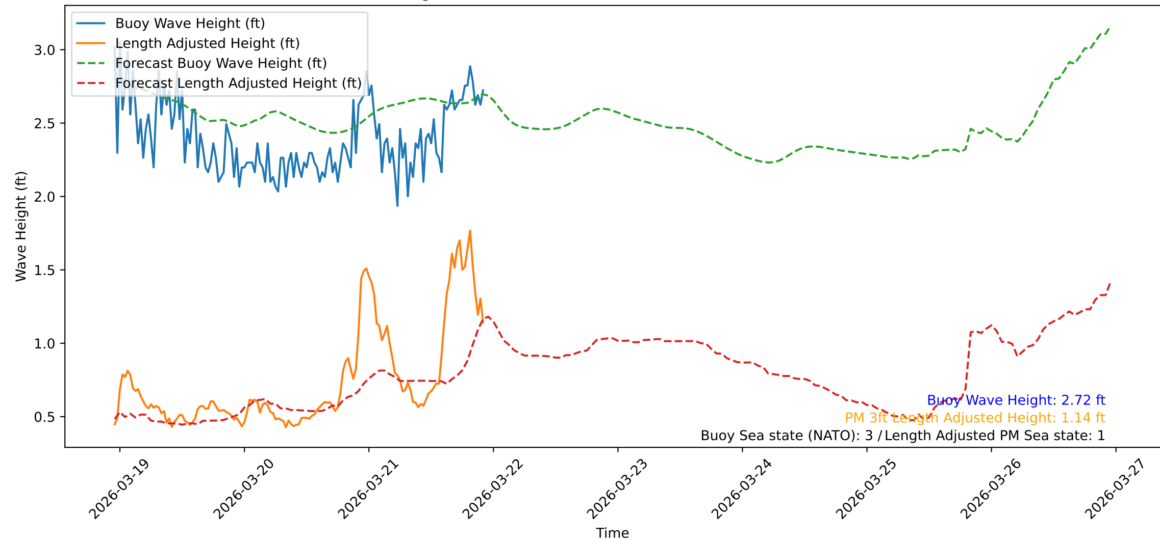
Wave Heights over Time for Green Beach at 2026-03-21 22:51:09
