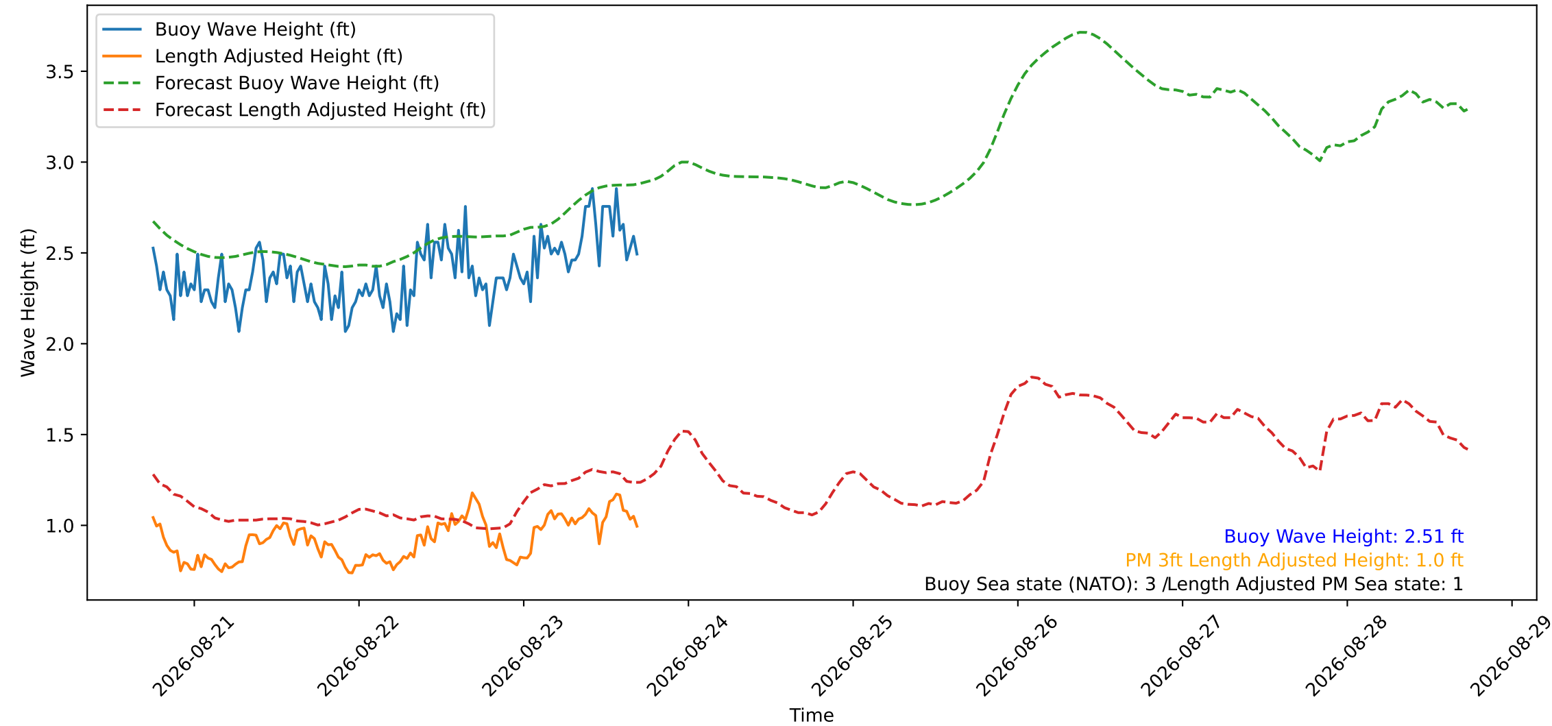
Wave Heights over Time for Red Beach at 2026-08-23 17:30:49
