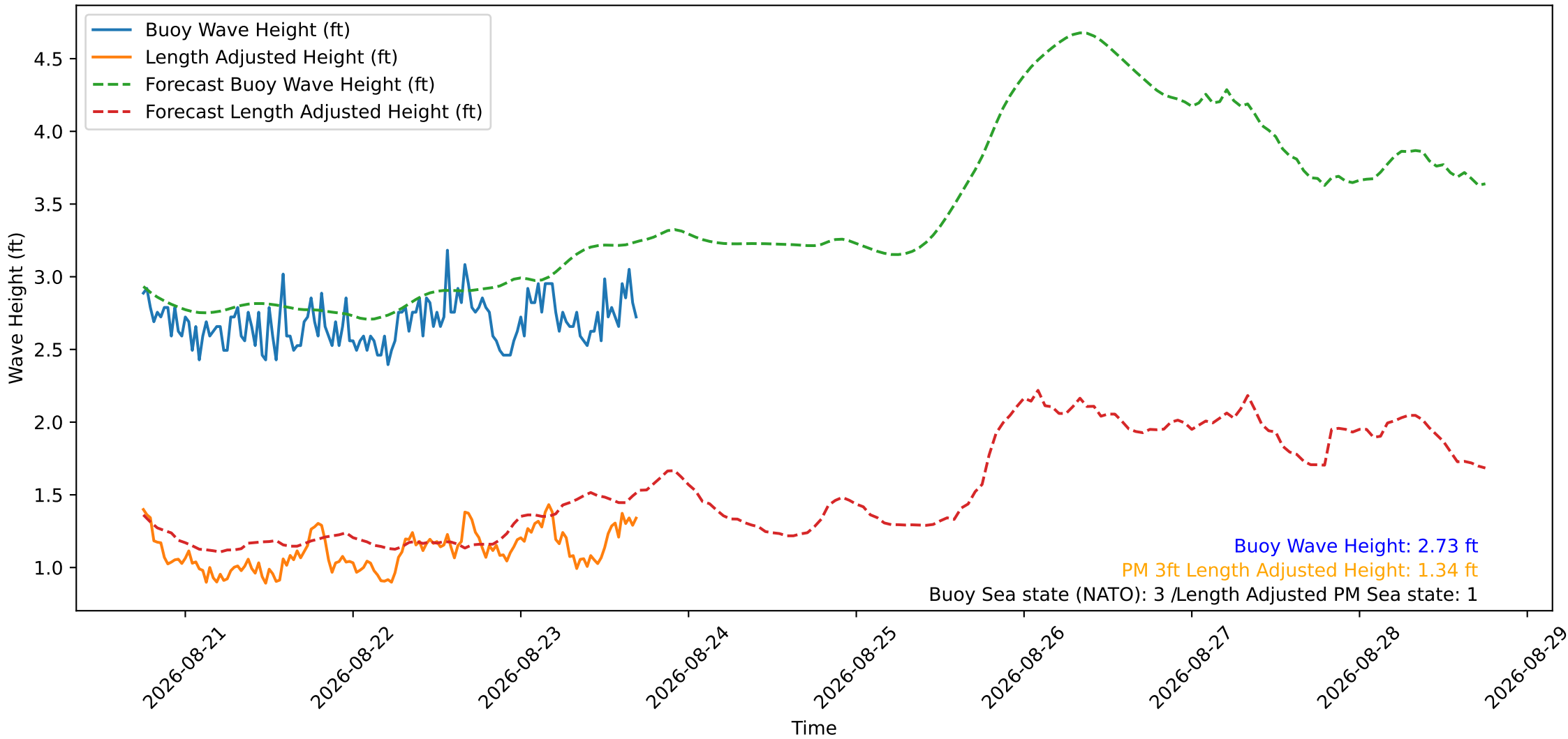
Wave Heights over Time for Green Beach at 2026-08-23 17:31:11
