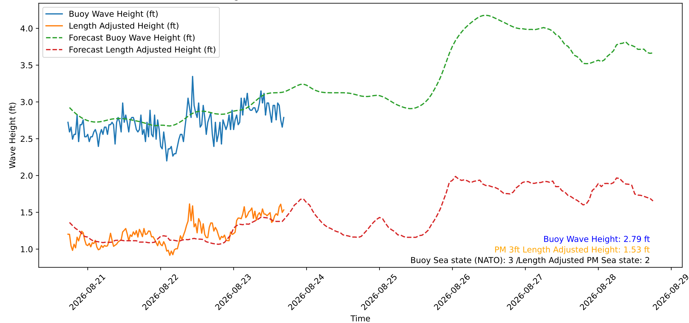
Wave Heights over Time for Oceanside Harbor at 2026-08-23 17:30:30
