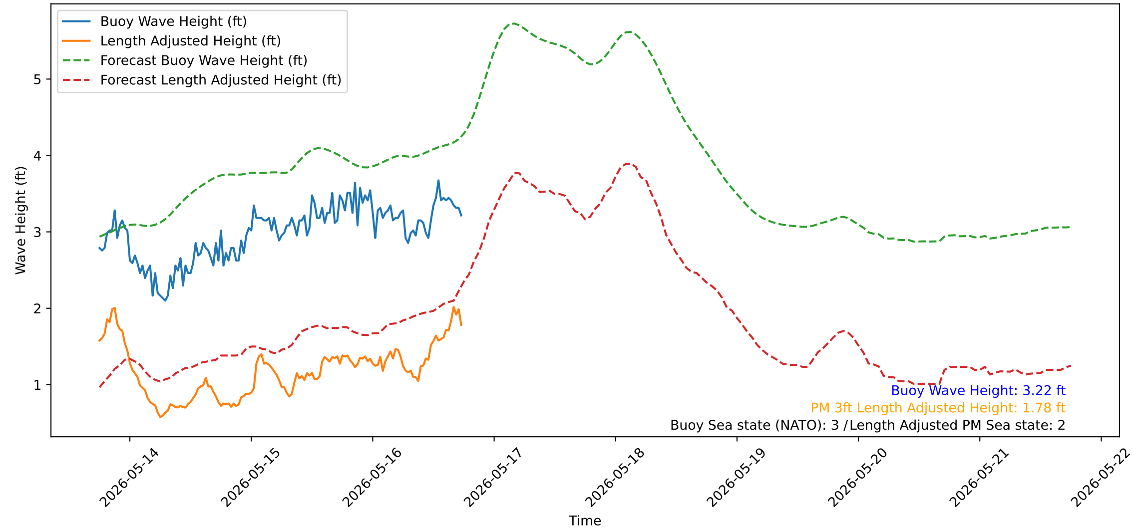
Wave Heights over Time for Green Beach at 2026-05-16 18:11:14
