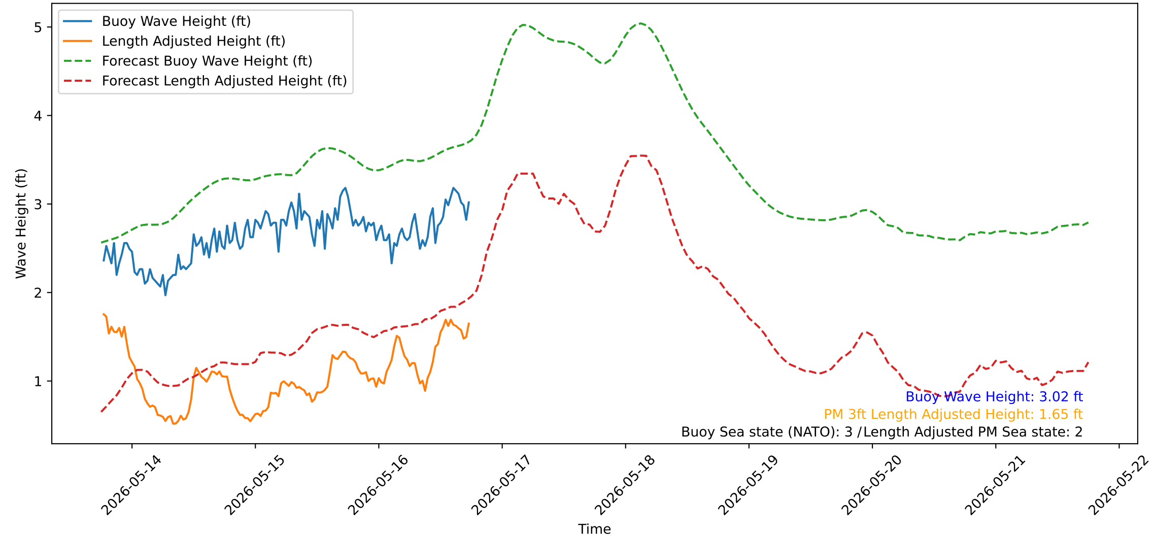
Wave Heights over Time for Red Beach at 2026-05-16 18:10:51
