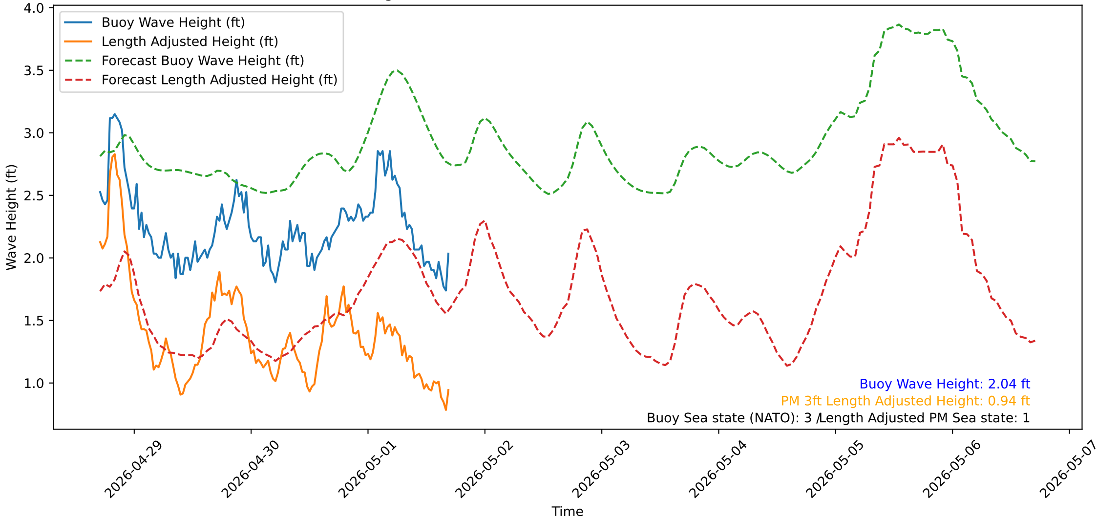
Wave Heights over Time for Green Beach at 2026-05-01 17:11:14
