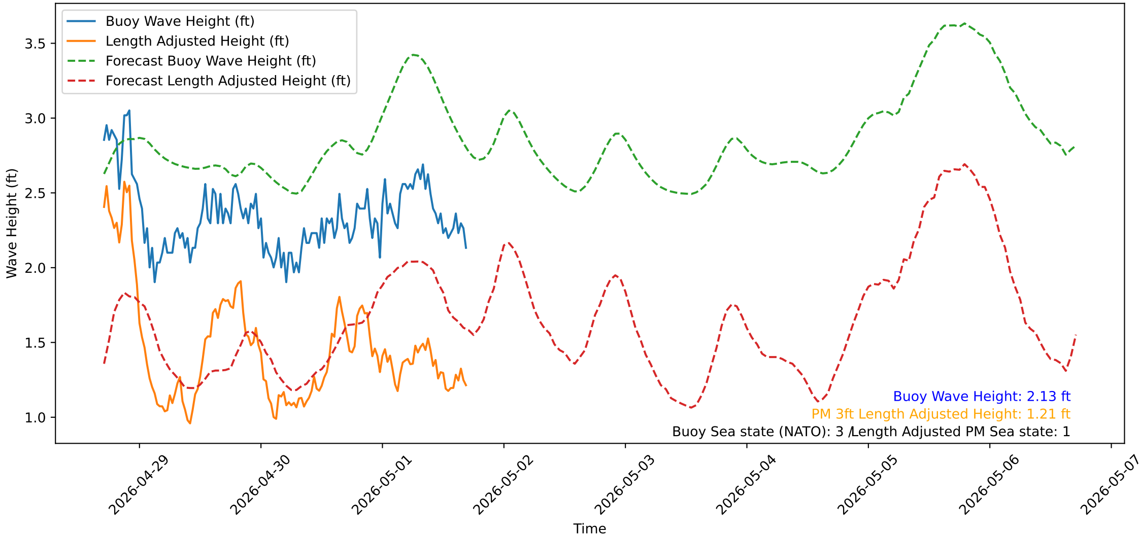
Wave Heights over Time for Oceanside Harbor at 2026-05-01 17:10:32
