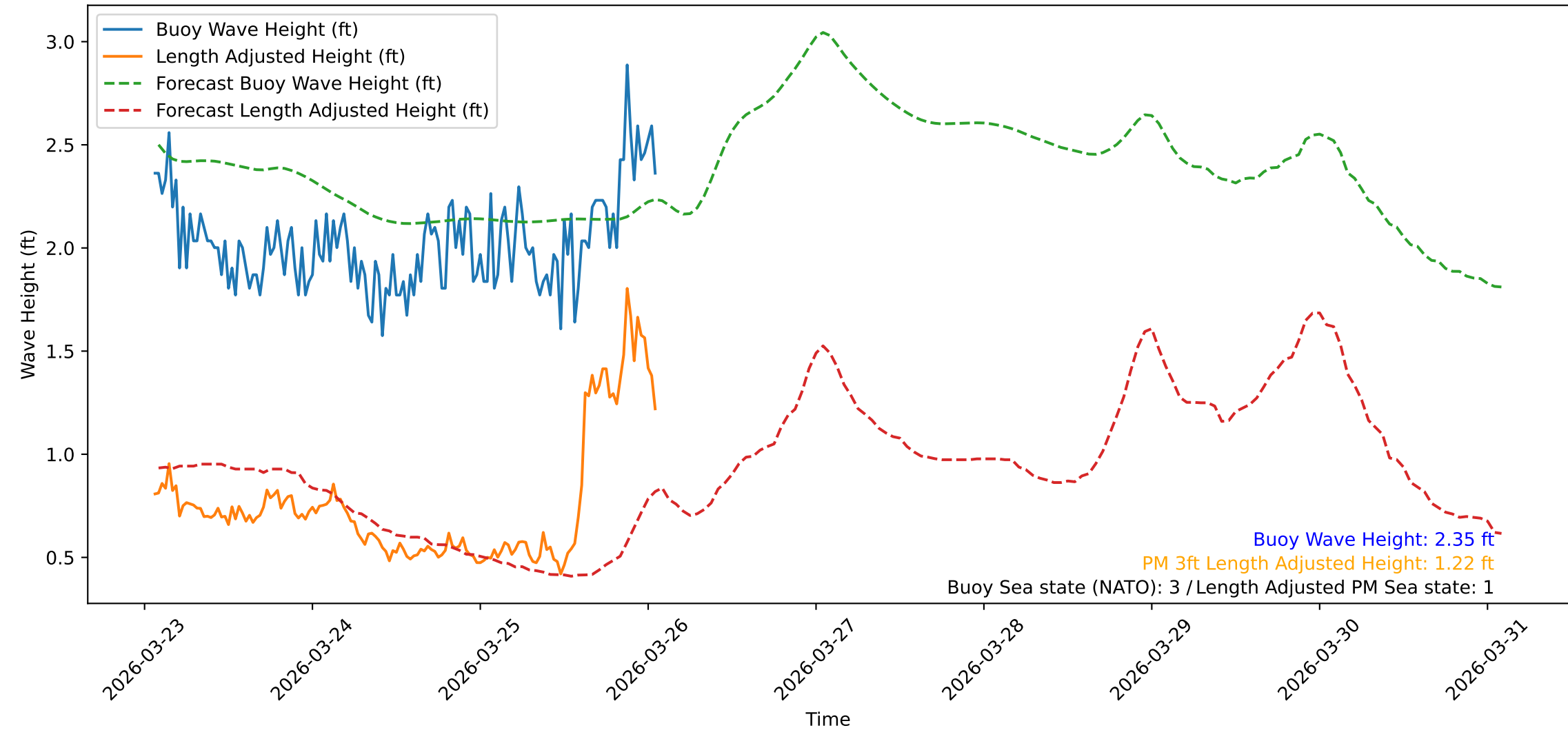
Wave Heights over Time for Oceanside Harbor at 2026-03-26 01:40:31
