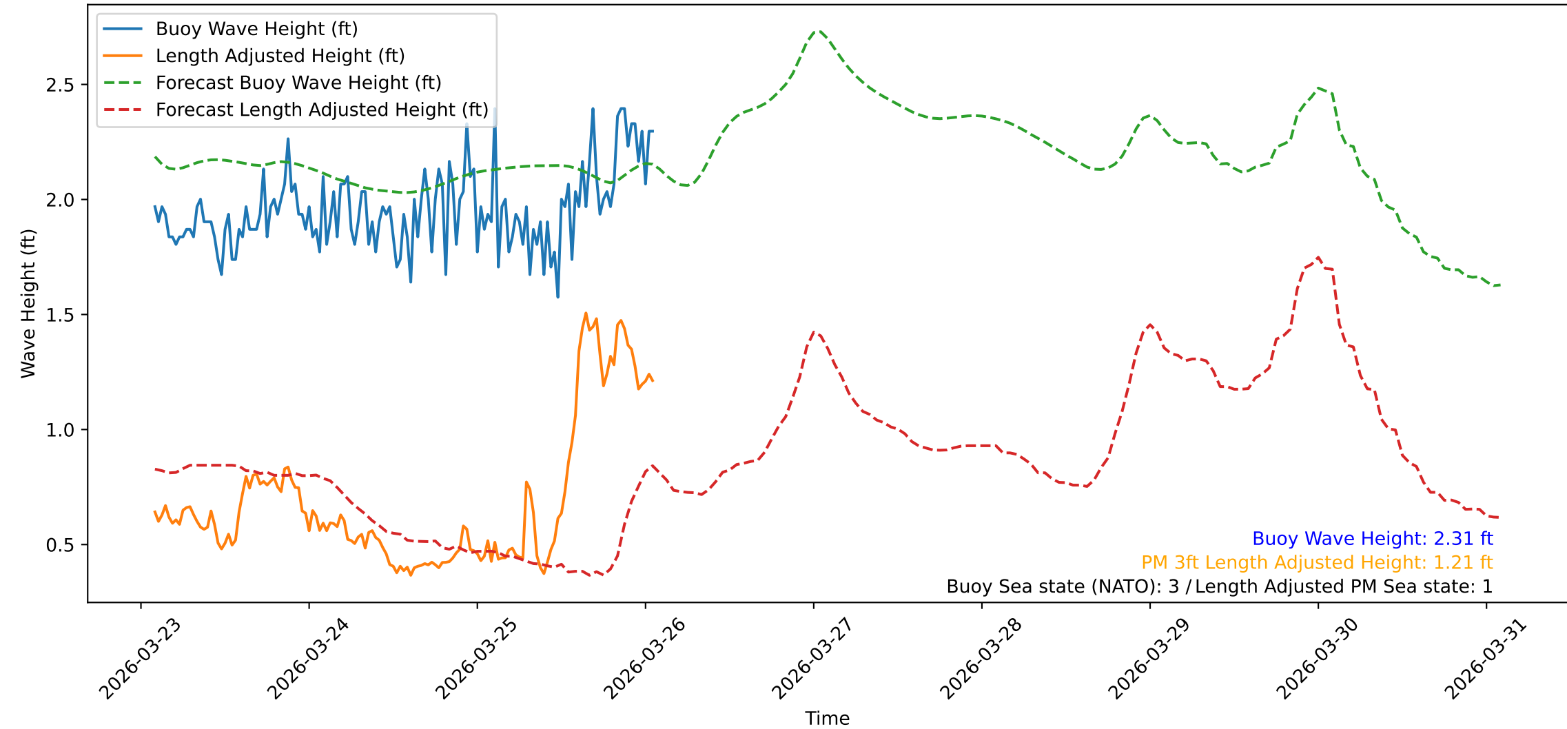
Wave Heights over Time for Red Beach at 2026-03-26 01:40:47
