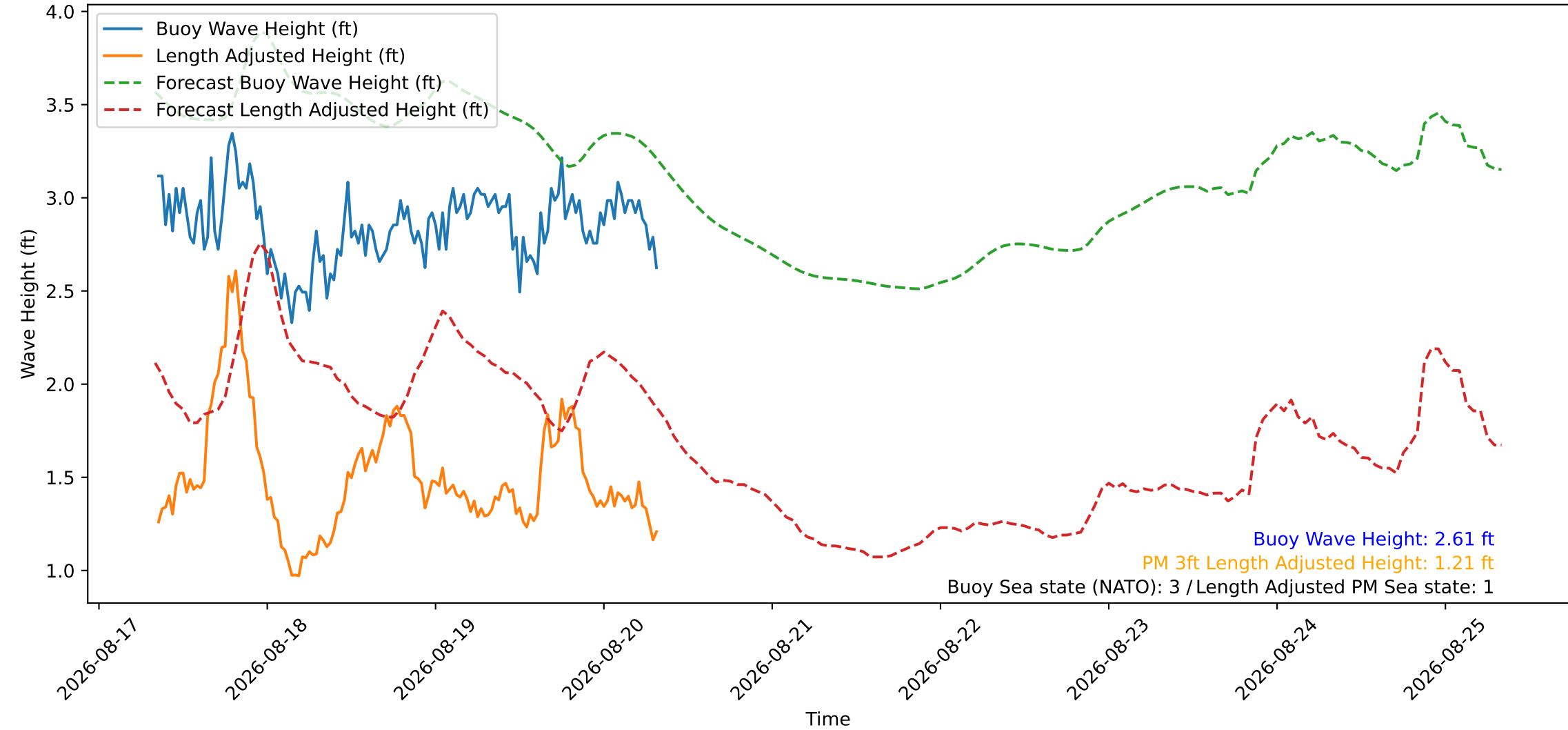
Wave Heights over Time for Red Beach at 2026-08-20 08:20:47
