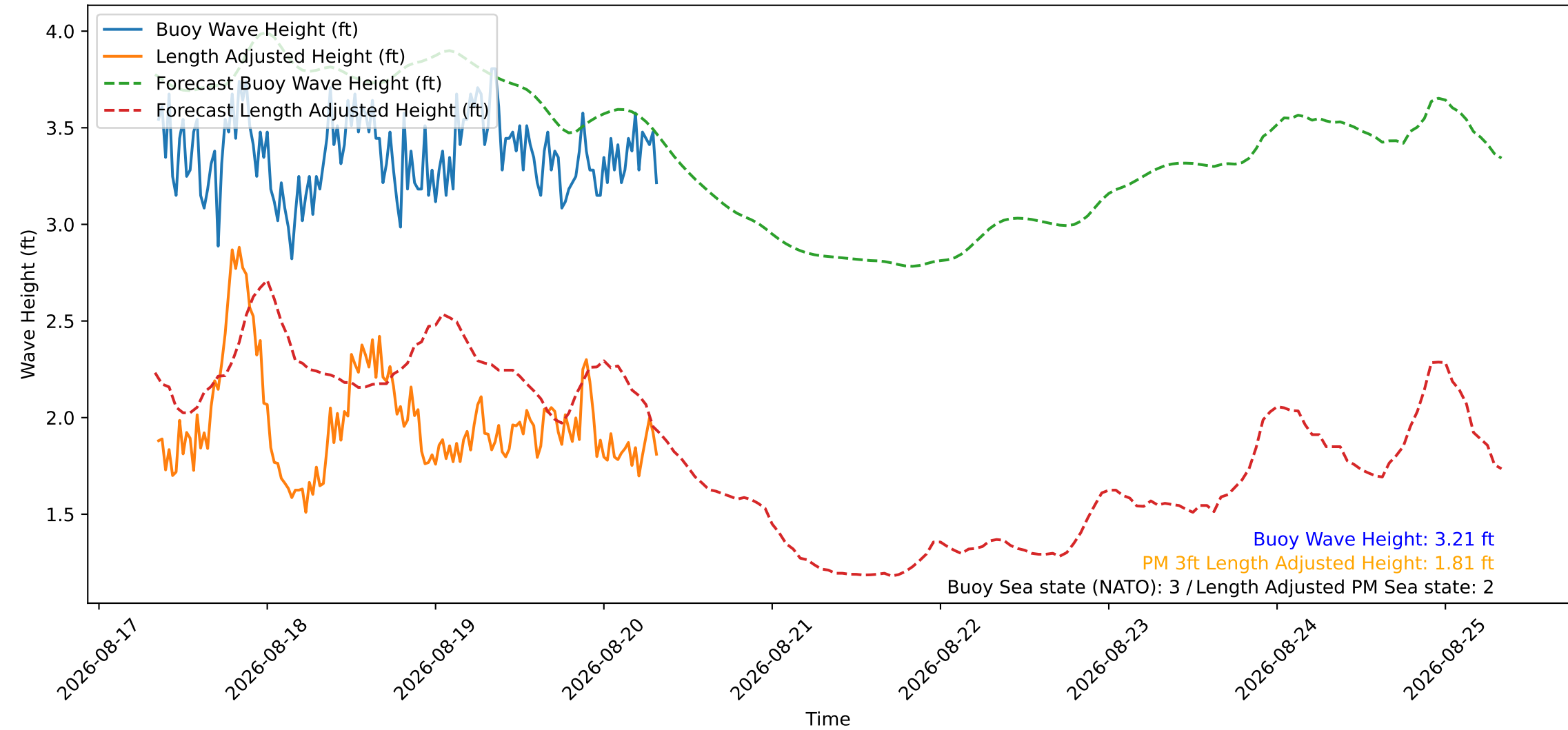
Wave Heights over Time for Oceanside Harbor at 2026-08-20 08:20:26
