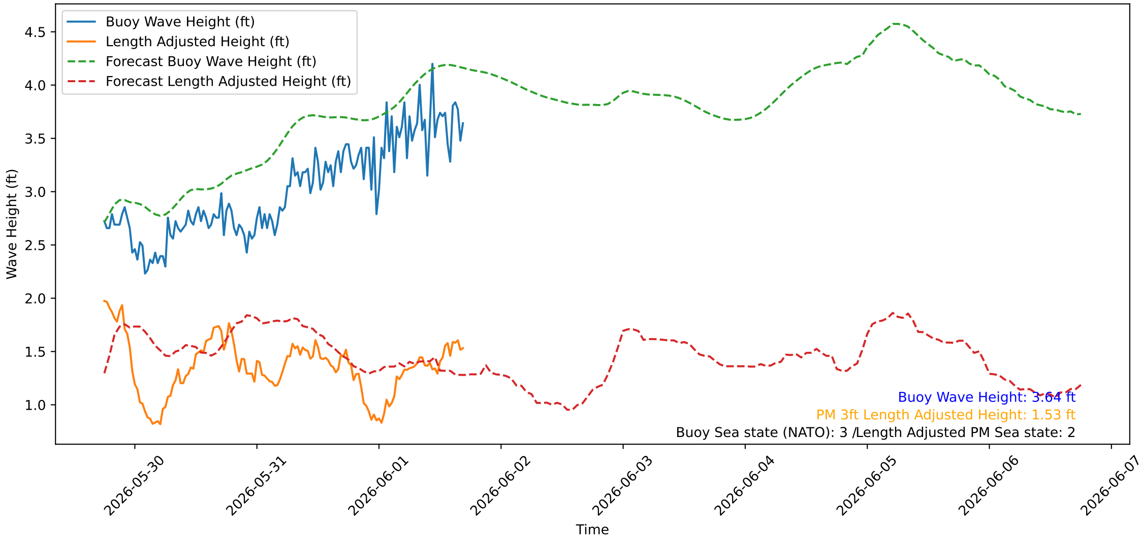
Wave Heights over Time for Red Beach at 2026-06-01 17:30:45
