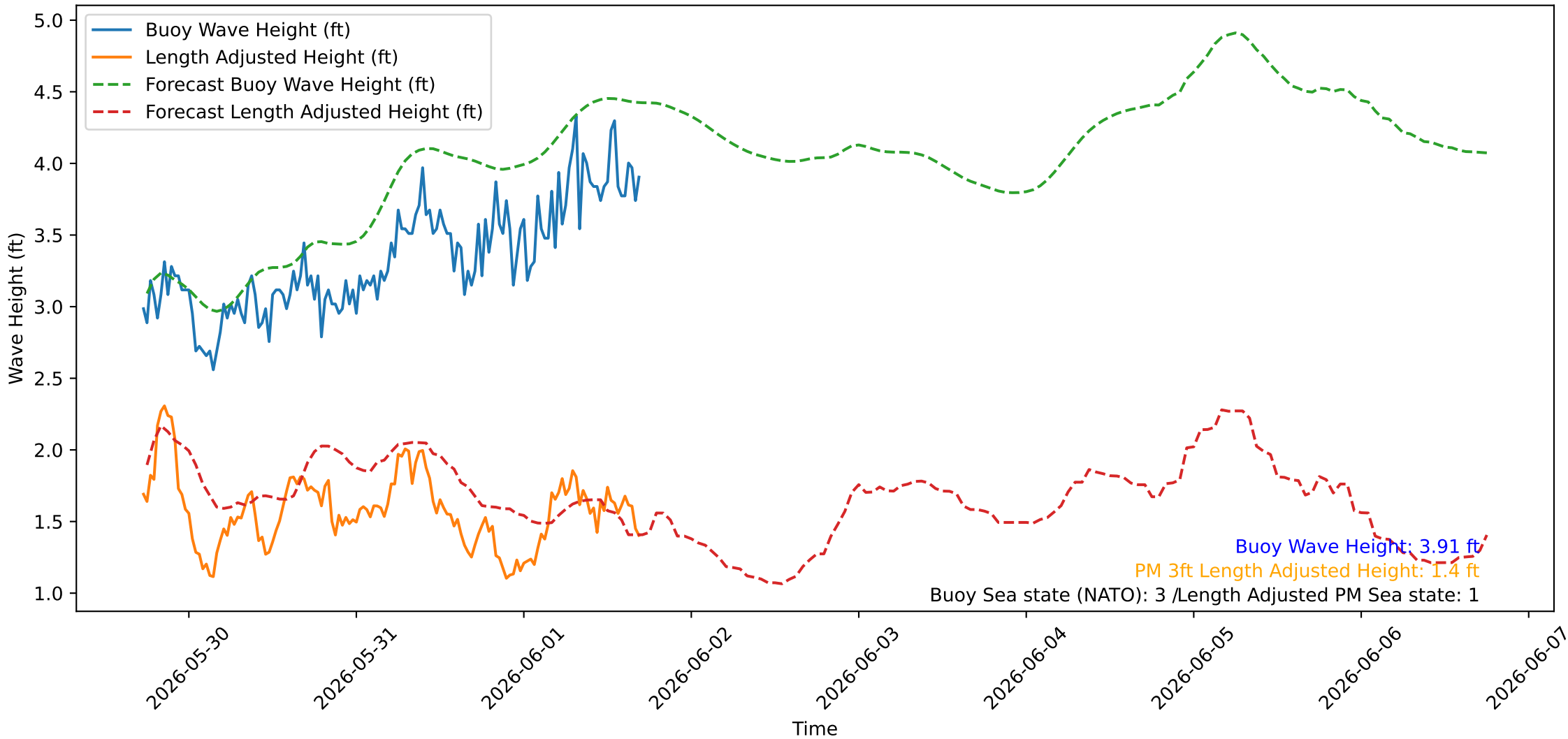
Wave Heights over Time for Green Beach at 2026-06-01 17:31:07
