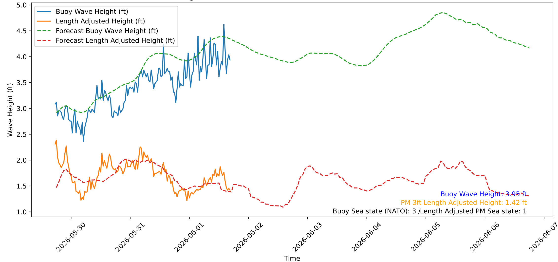
Wave Heights over Time for Oceanside Harbor at 2026-06-01 17:30:26
