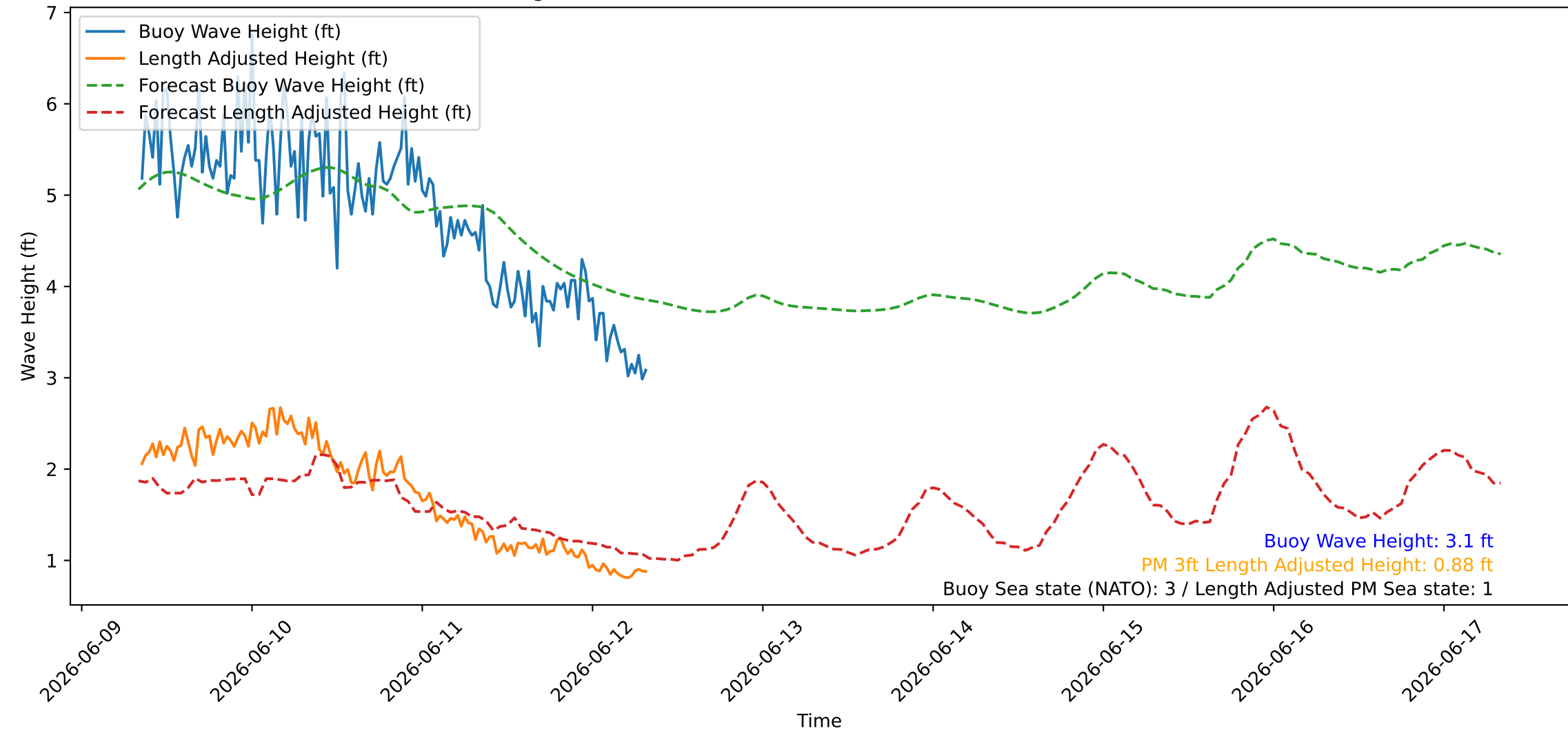
Wave Heights over Time for Oceanside Harbor at 2026-06-12 08:20:26
